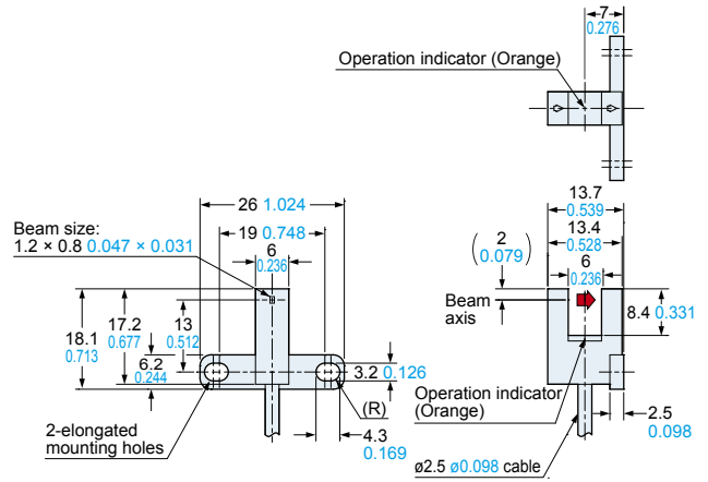
PM-T45□ Sensor
