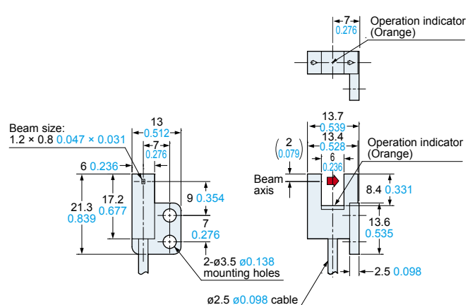
PM-R45□ Sensor
