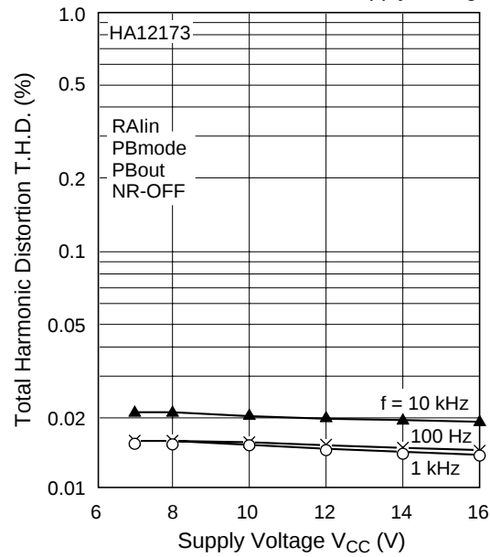
Total Harmonic Distortion vs. Supply Voltage (1)
