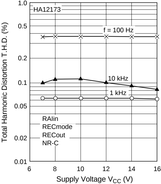
Total Harmonic Distortion vs. Supply Voltage (6)
