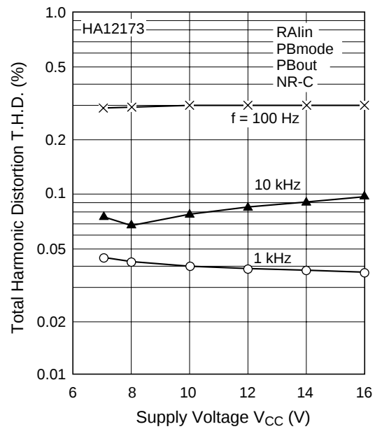
Total Harmonic Distortion vs. Supply Voltage (3)
