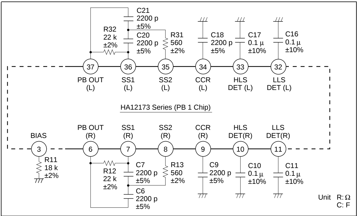
Figure 6 Tolerances of External Components
