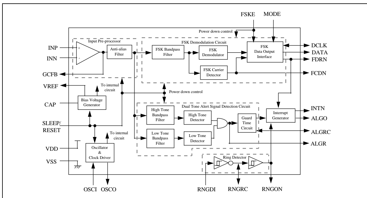
Figure 6. The Block Diagram of W91030B
