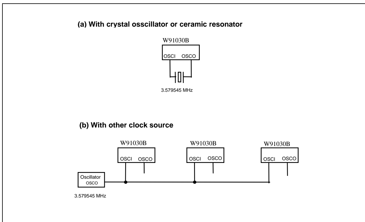
Figure 7-9. Some Application of Clock Driven Circuit
