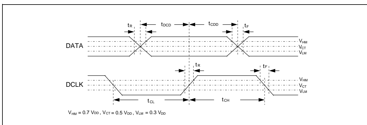
Figure 8-4. Data and DCLK Mode 0 Output Timing
