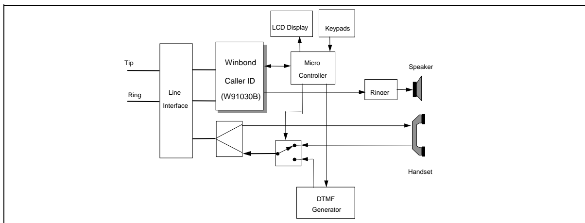
Figure 5. System Diagram for Caller ID Application
