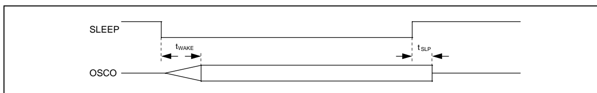
Figure 8-1. Wake up and Sleep Down Timing
