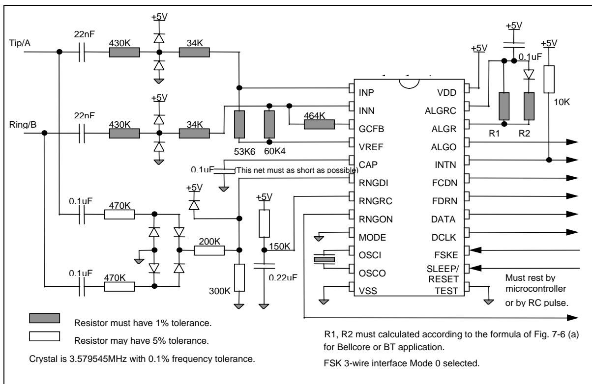
Figure 9-1 Application Circuit
