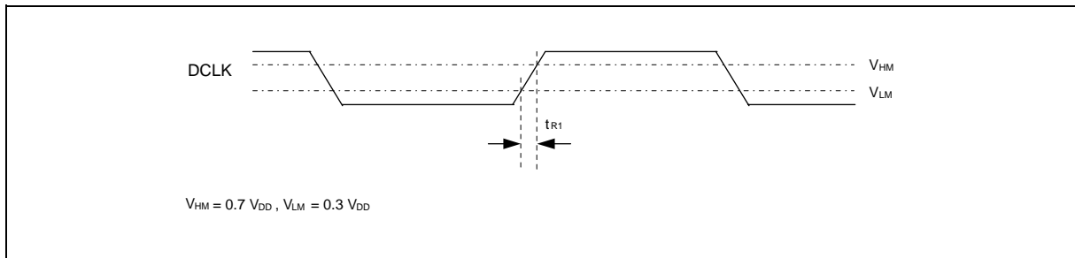
Figure 8-7. DCLK Mode 1 Input Timing
