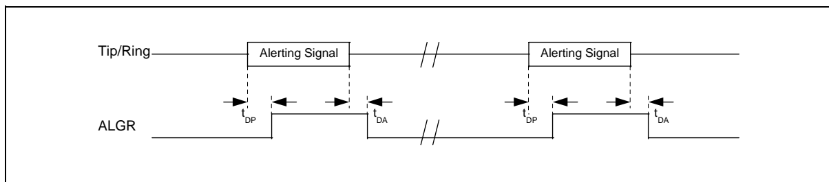
Figure 8-2. Alert Signal Present and Absent Detect Timing
