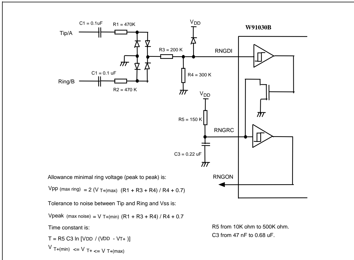
Figure 7-1. Application Circuit of the Ring Detector
