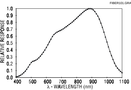
Fig. 3 Spectral Responsivity
