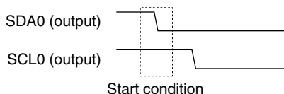
Figure 17.5.1 Start Condition
