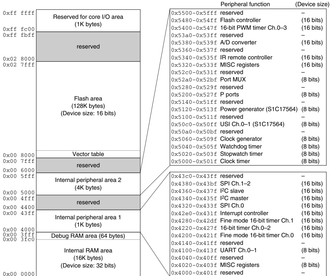
Figure 3.1 S1C17554/564 Memory Map
