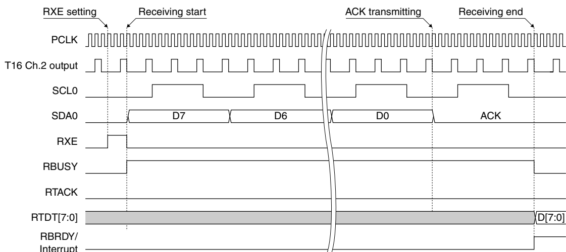
Figure 17.5.8 Data Receiving
