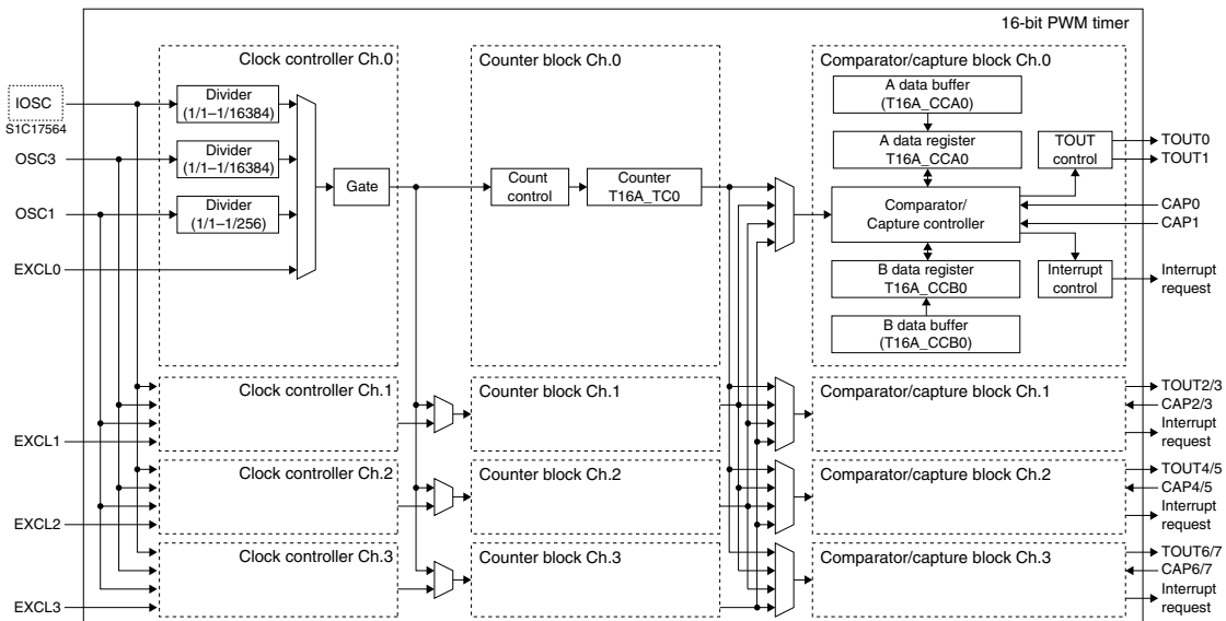
Figure 11.1.1 T16A Configuration
