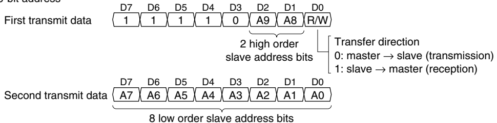
Figure 19.5.3.4 Transmit Data Specifying Slave Address and Transfer Direction
