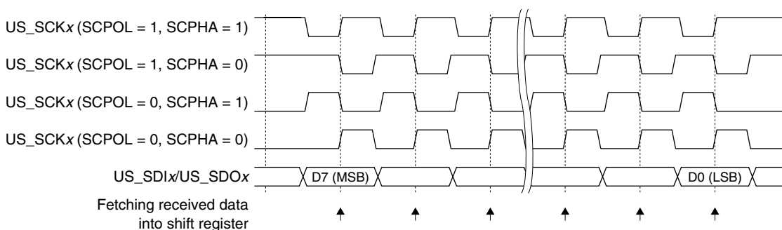
Figure 19.8.2 Clock and Data Transfer Timing
