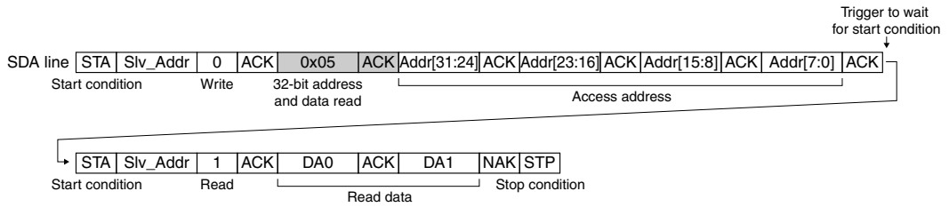
Figure 19.9.4 I 2 C Master Read (Data Transmission to Master)
