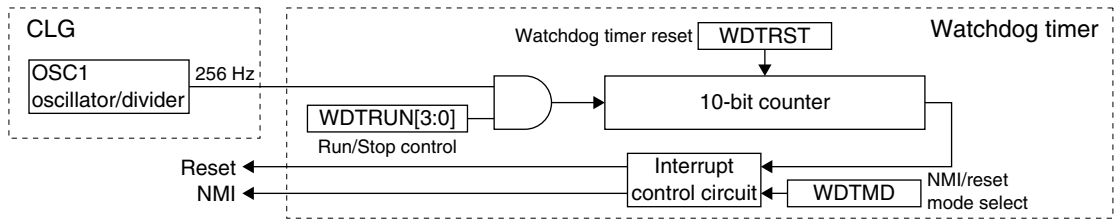
Figure 14.1.1 WDT Configuration
