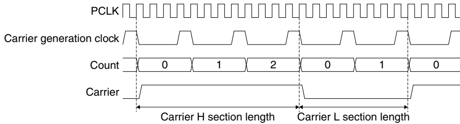
Figure 20.7.1 Carrier Signal Generation
