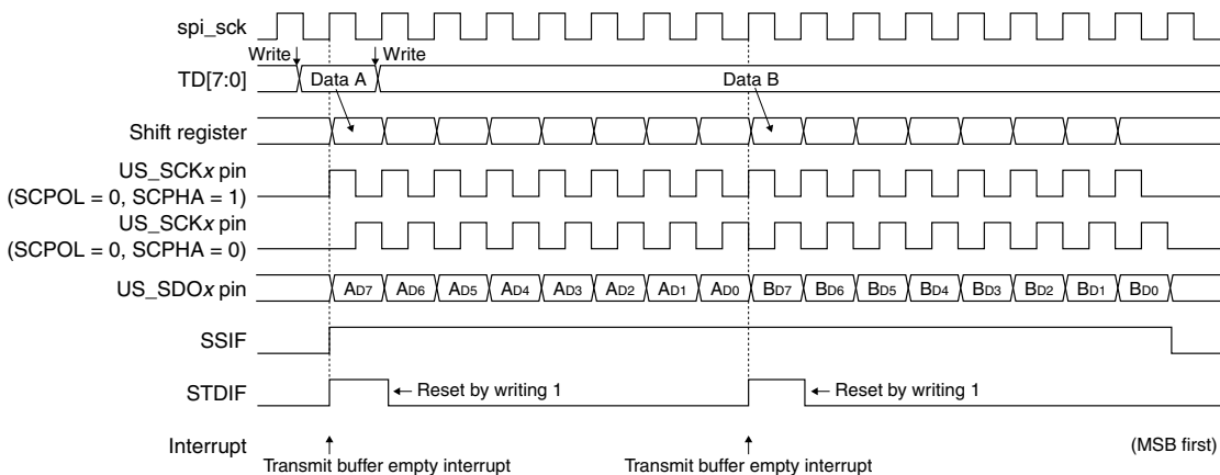
Figure 19.5.2.1 Data Transmission Timing Chart (SPI master mode)
