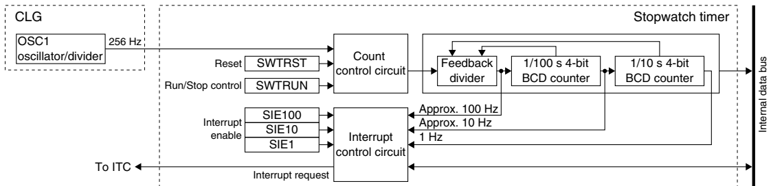
Figure 13.1.1 SWT Configuration
