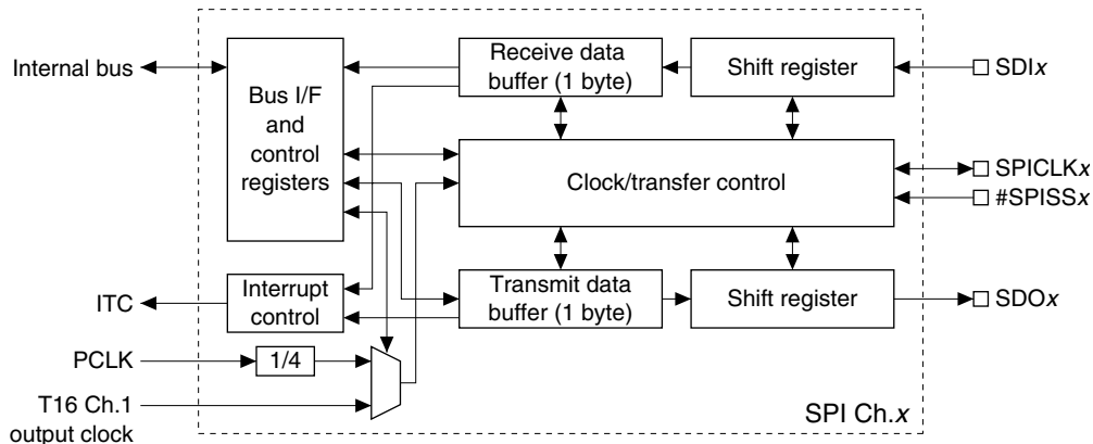
Figure 16.1.1 SPI Module Configuration (1 channel)
