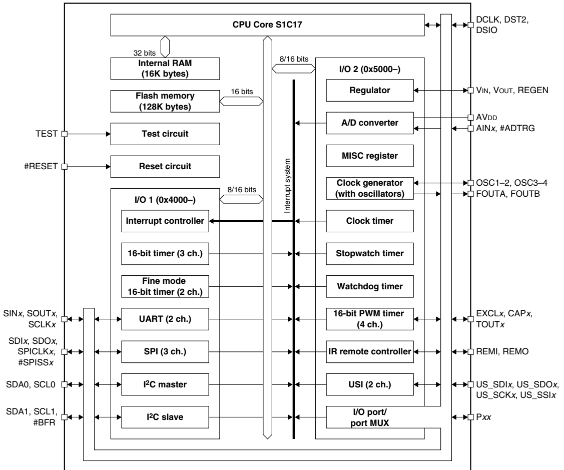
Figure 1.2.2 S1C17564 Block Diagram
