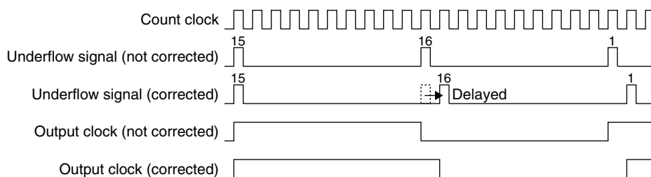
Figure 10.8.1 Delay Cycle Insertion in Fine Mode
