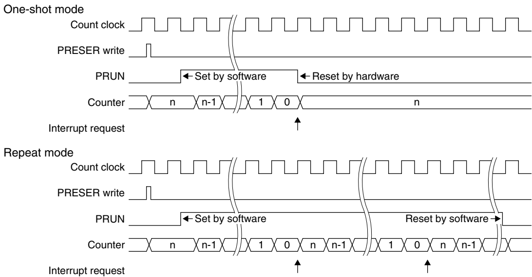
Figure 10.6.1 Count Operation
