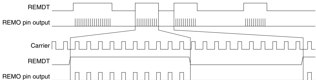
Figure 20.5.1 Data Transmission
