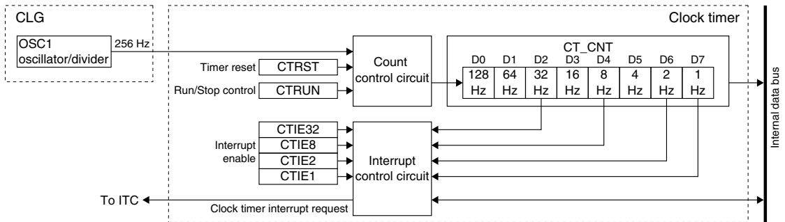
Figure 12.1.1 CT Configuration
