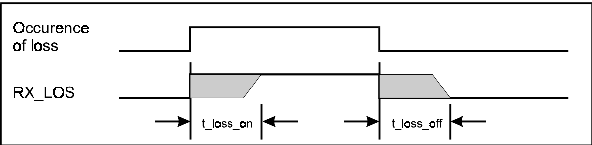
Figure 6: Timing of RX_LOS detection
