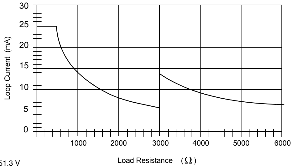
b. Loop Current vs. Load Resistance (Typical)
