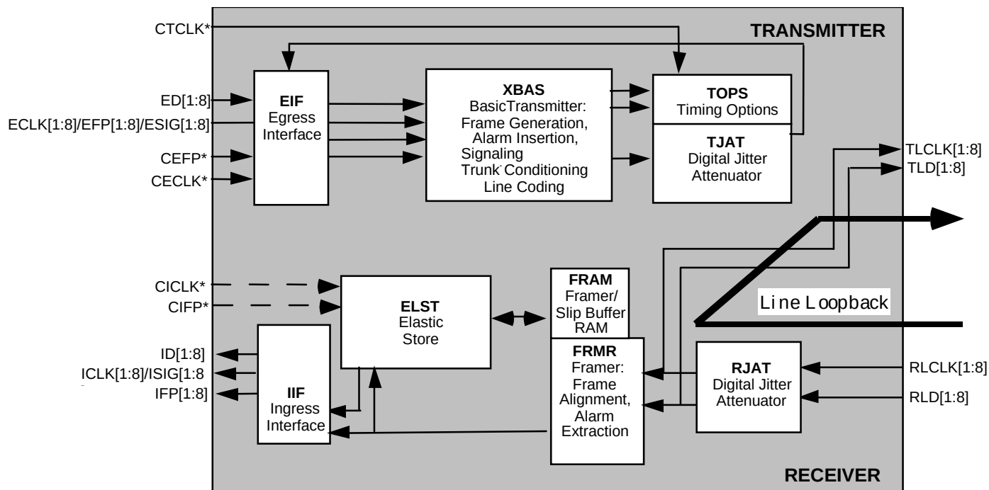
Figure 27 - Line Loopback
