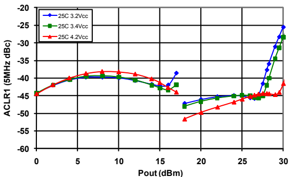
Figure 8: WCDMA ACLR1 (dBc) over Voltage ( T_c = 25\text{ }^\circ\text{C} )
