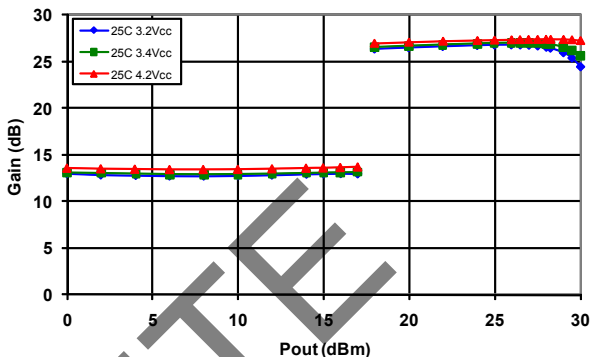
Figure 4: WCDMA Gain (dB) over Voltage ( T_c = 25\text{ }^\circ\text{C} )
