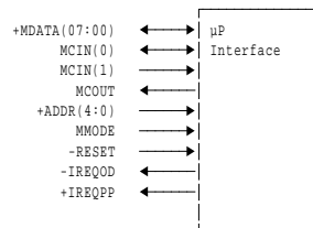
Figure 4-3. Microprocessor Interface
