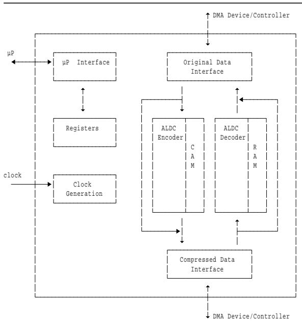
Figure 2-1. ALDC1-20S-HA High-level Functional Units
