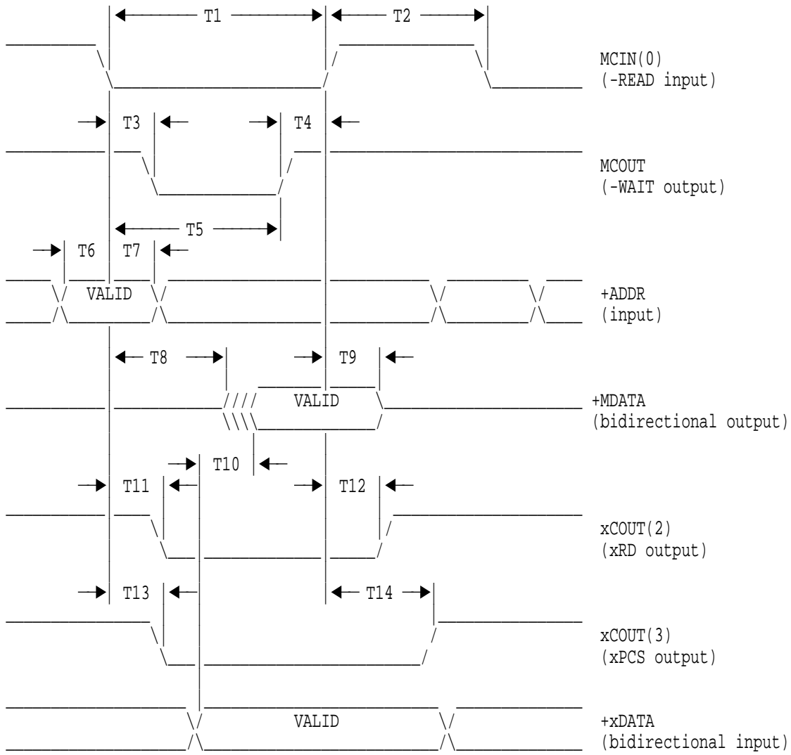
Figure 4-17 (Part 1 of 2). Peripheral Access Read Timing with MMODE Tied Low
