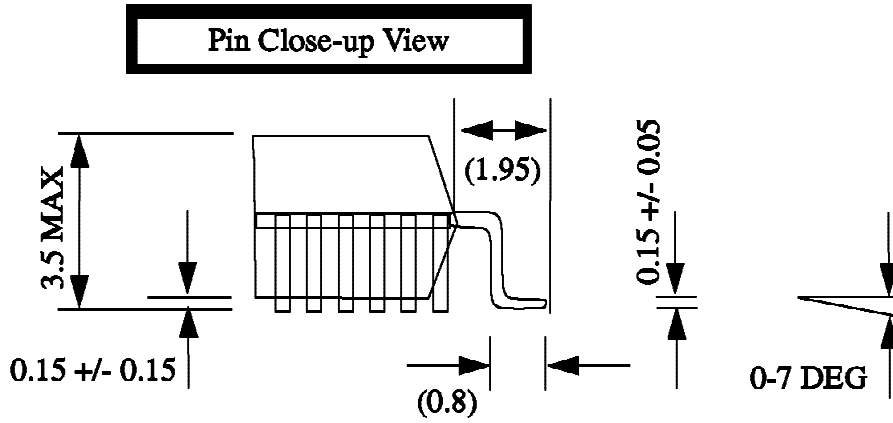
Figure 7-2. ALDC1-20S-HA Pin Close-up View. All length and tolerance dimensions in millimeters.
