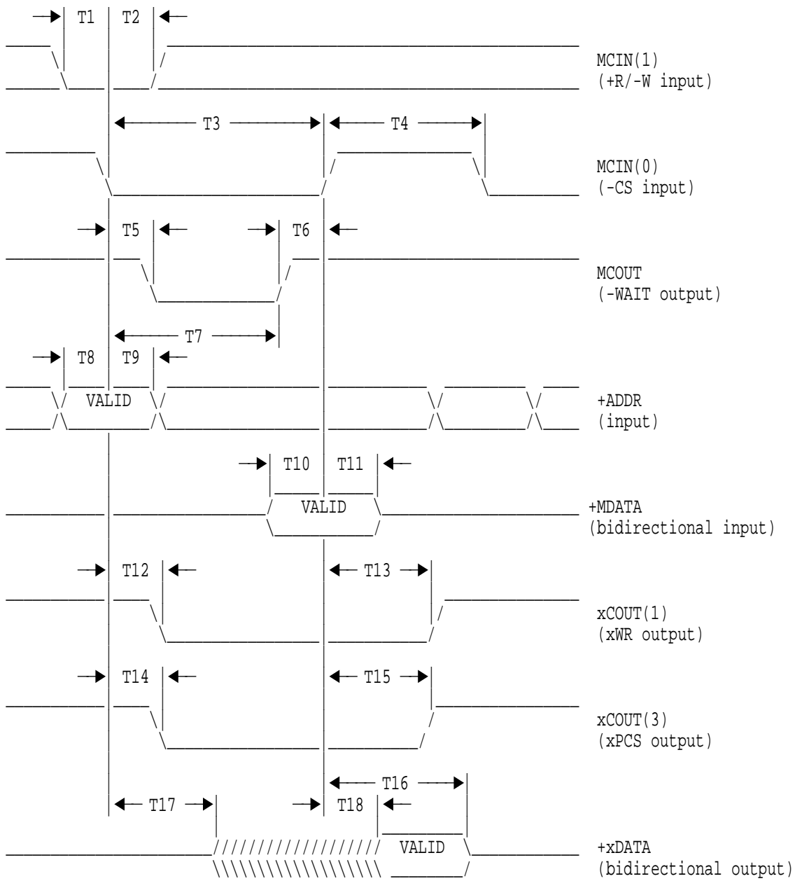
Figure 4-16 (Part 1 of 2). Peripheral Access Write Timing with MMODE Tied High
