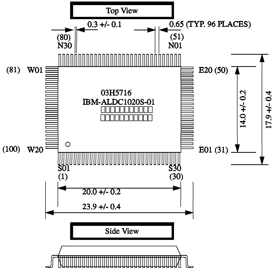
Figure 7-1. ALDC1-20S-HA Top and Side Views. All length and tolerance dimensions in millimeters. The orientation mark is shown in the lower left-hand corner of the top view.
