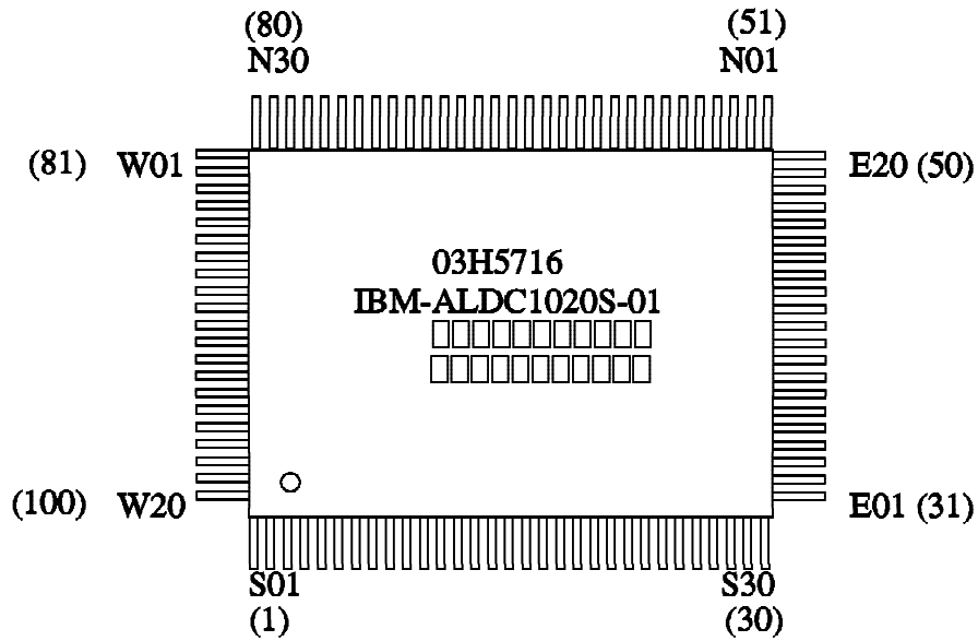
Figure 5-1. Preliminary Pin Numbering Diagram. For the ALDC1-20S-HA. Module is viewed from top. See Figure 5-2 for the corresponding pin names, signal directions, and descriptions.
