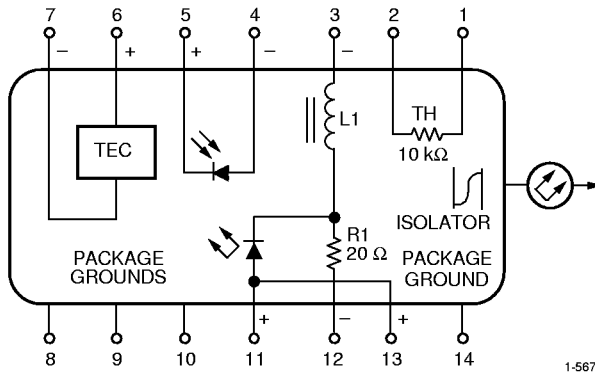
Figure 1. Circuit Schematic (Top View) Industry-Standard (2.5 Gbits/s) Pinout, 25 Ω Resistive Input Impedance
