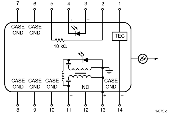
Figure 2. Circuit Schematic (Top View) Lucent Technologies Standard Pinout, 75 Ω Transformer-Matched Input Impedance
