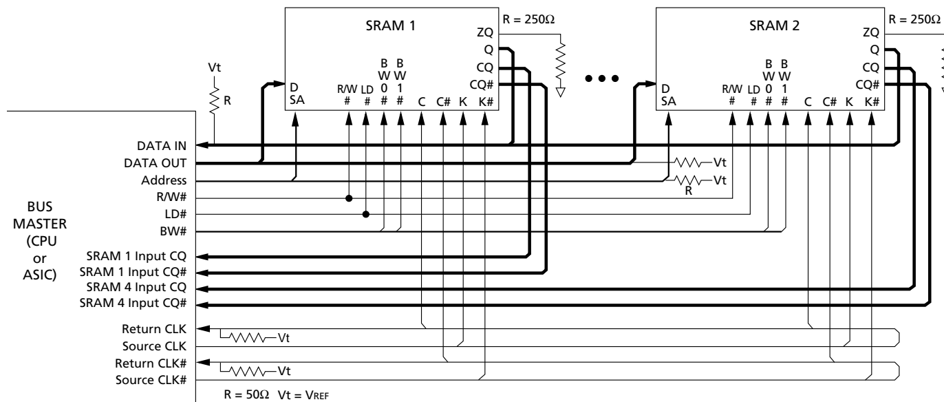
Figure 3: Application Example
