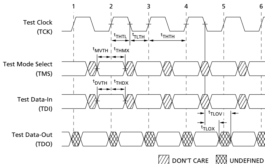
Figure 9: TAP Timing
