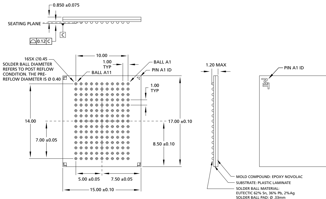
Figure 11: 165-Ball FBGA
