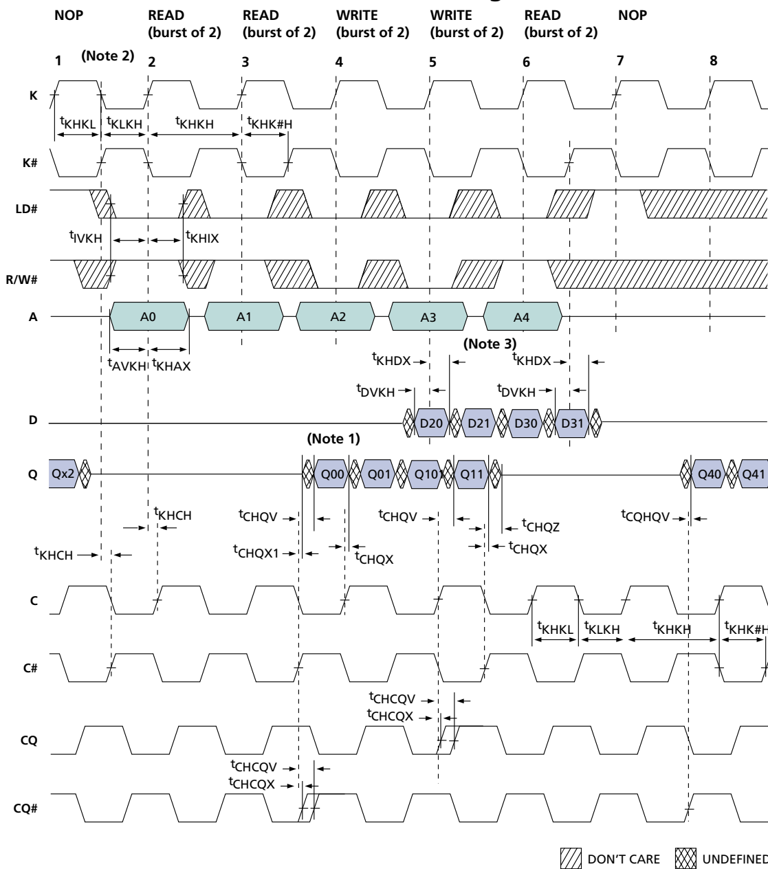
Figure 6: READ/WRITE Timing
