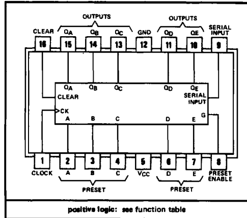
SN5496, SN54L96 . . . J OR W PACKAGE SN54L96 . . . J PACKAGE SN7496, SN74L96, SN74LS96 . . . J OR N PACKAGE (TOP VIEW)
