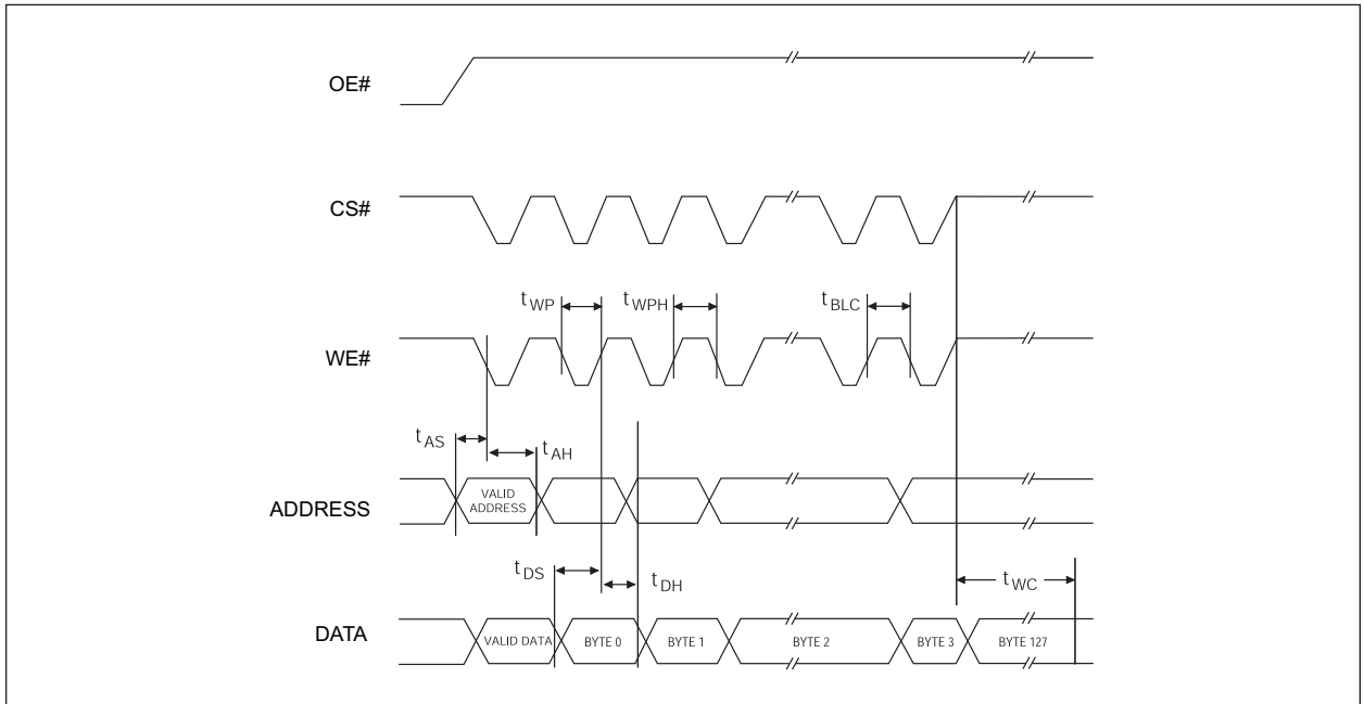
FIGURE 9 – PAGE MODE WRITE WAVEFORMS
