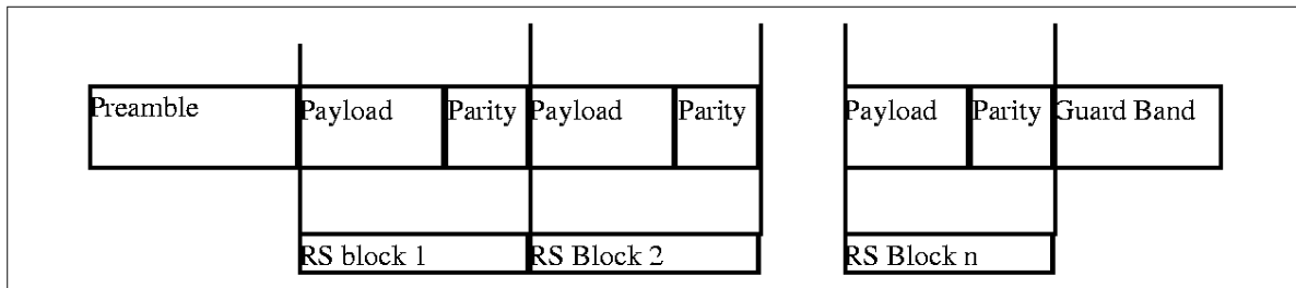
Figure 6 MCNS Packet Structure
