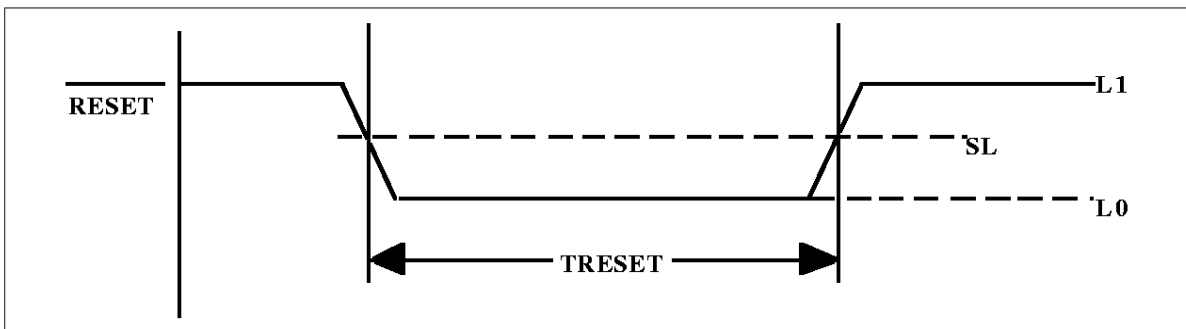
Figure 16 Reset
