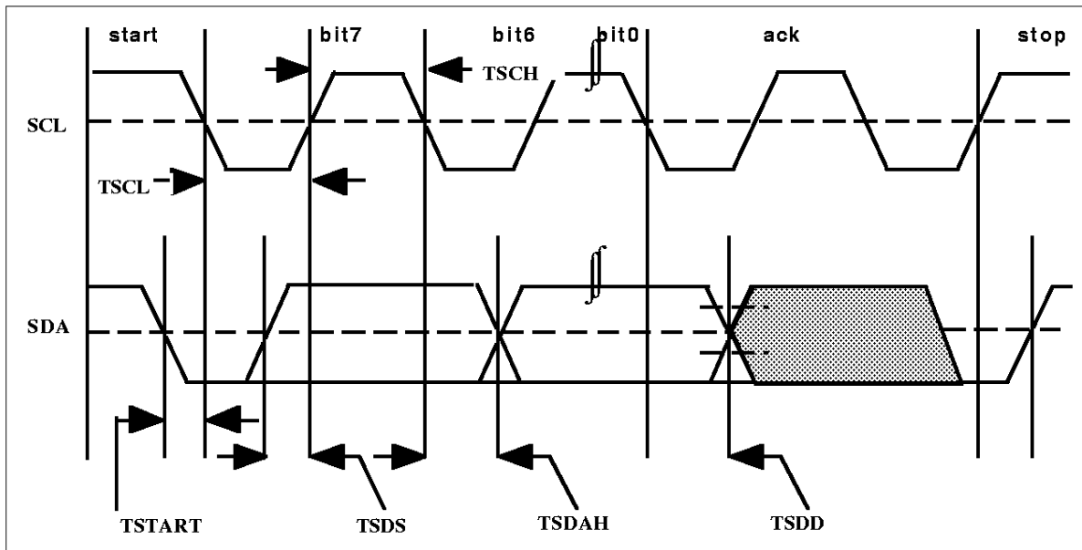
Figure 15 I 2 C Interface
