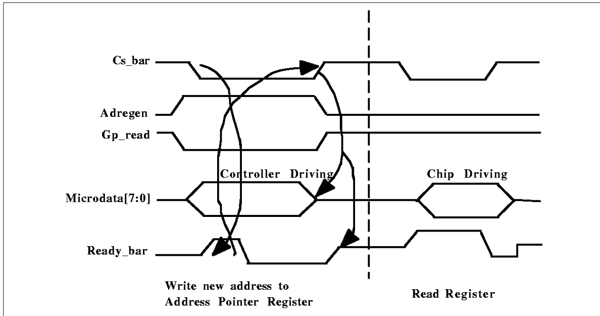
Figure 8 uP Interface Protocol
