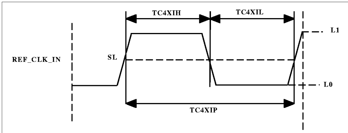
Figure 11 Clock Inputs
