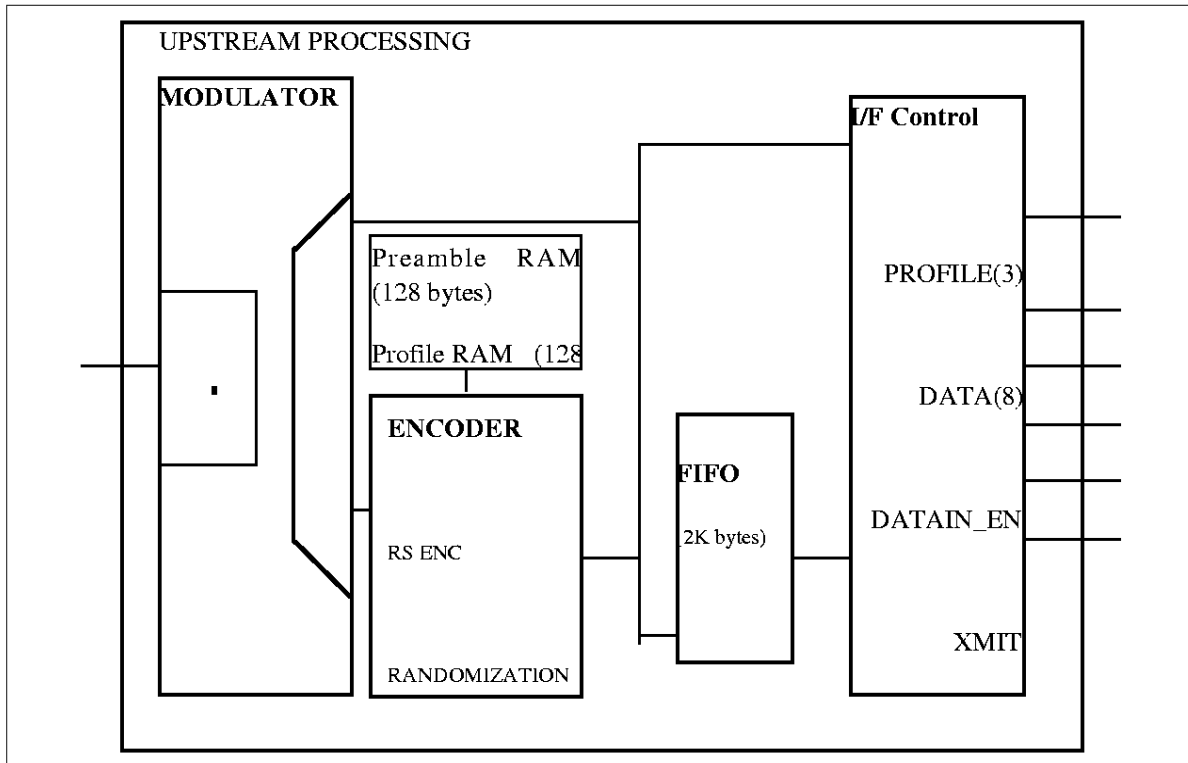
Figure 2 Upstream Modulator Block Diagram
