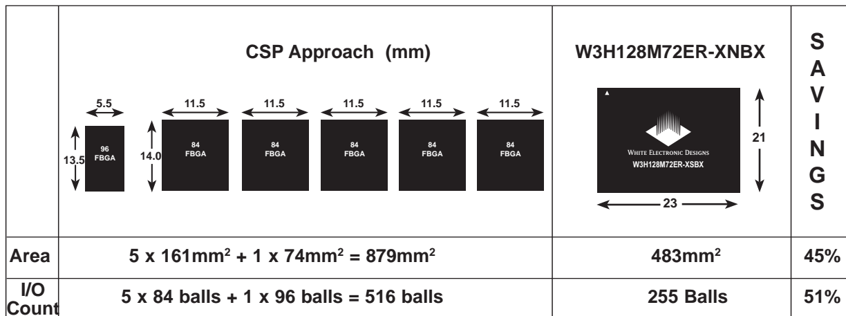
FIGURE 1 – DENSITY COMPARISONS
