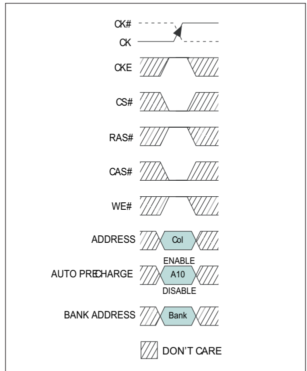
FIGURE 11 – READ COMMAND
