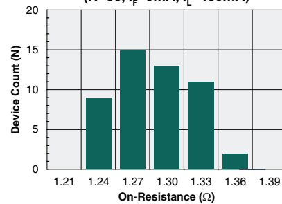
Typical On-Resistance Distribution (N=50, I_F=0\text{mA} , I_L=400\text{mA} )
