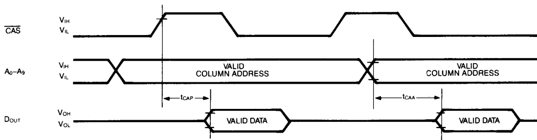
FIGURE 1. FAST PAGE MODE ACCESS TIME DETERMINATION
