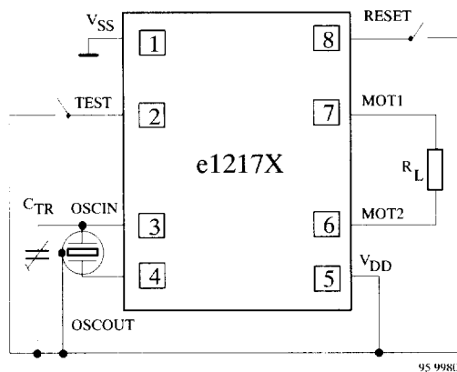
Figure 2. Functional test circuit
