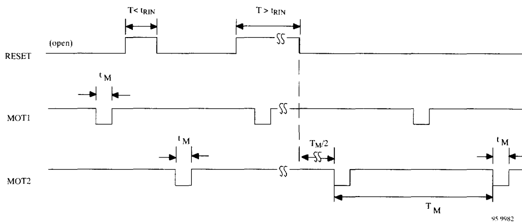
Figure 4. Motor drive outputs and RESET
