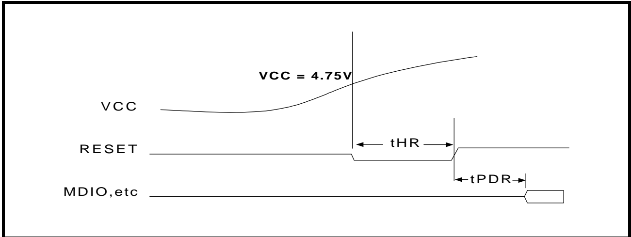
Figure 35: Power-Down/Hardware Reset Timing Parameters (Over Recommended Range)
