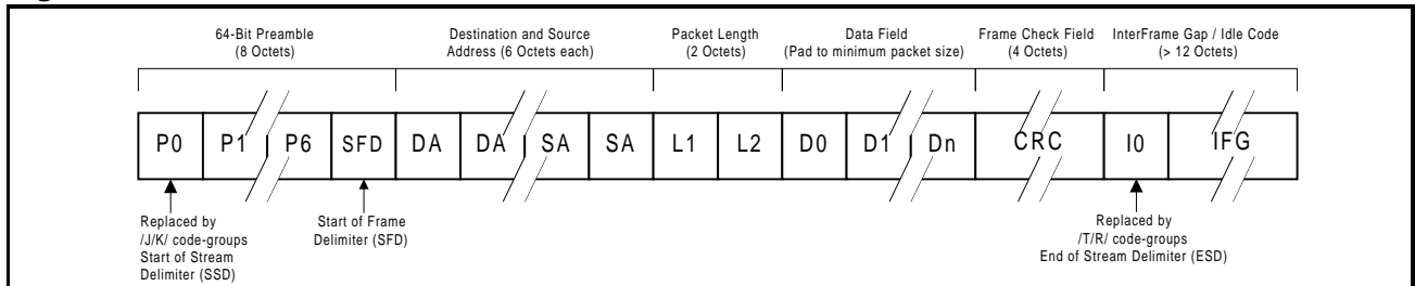
Figure 12: 100BASE-TX Frame Structure
