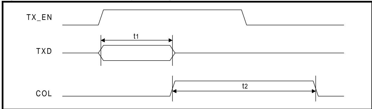
Figure 30: 10BASE-T Jab and Unjab Timing
