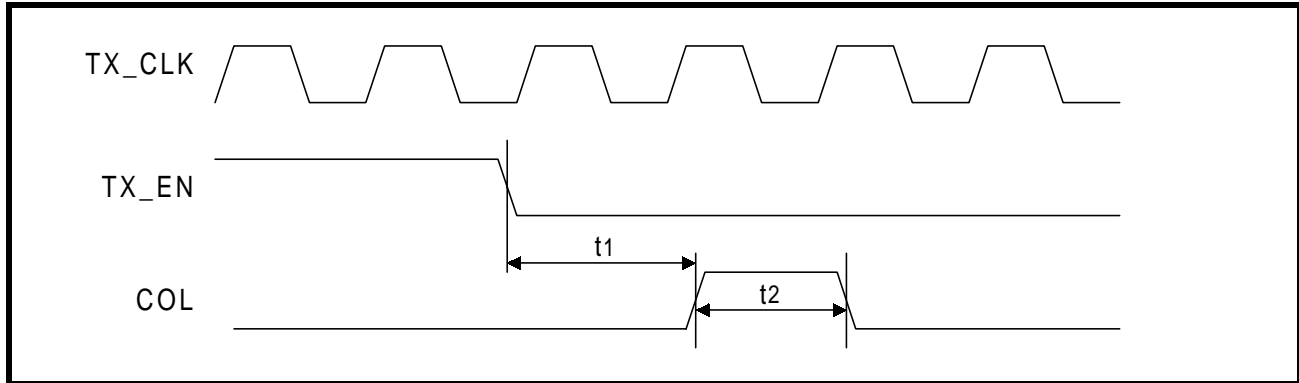
Figure 29: 10BASE-T SQE (Heartbeat) Timing
