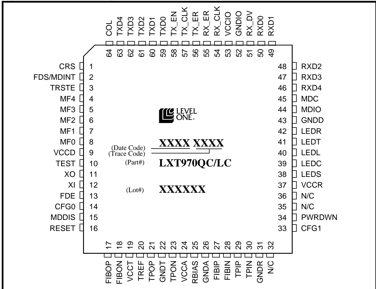
Figure 1: LXT970 Pin Assignments
