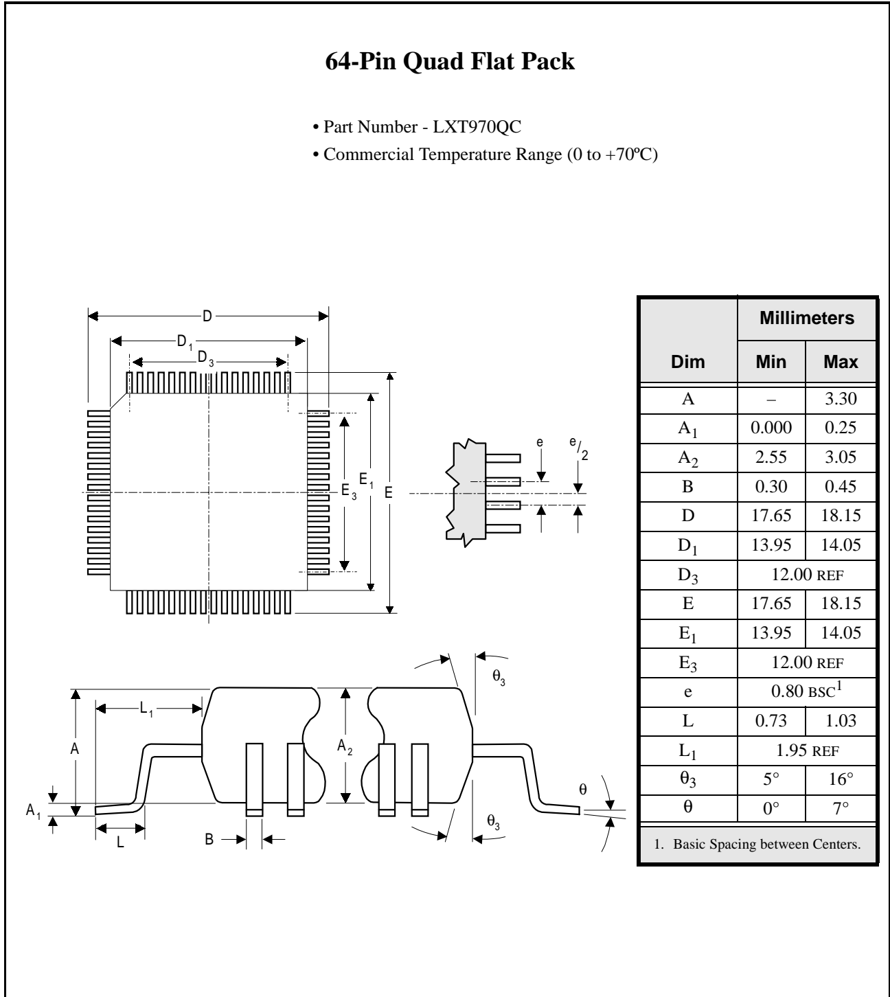
Figure 37: 64-Pin PQFP Package Diagram
