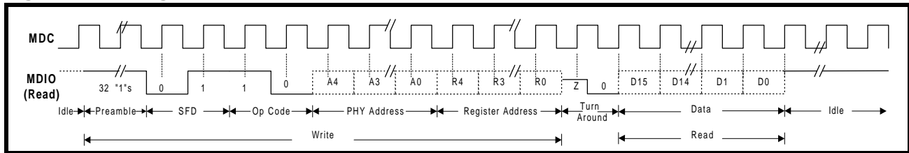
Figure 8: Management Interface - Read Frame Structure
