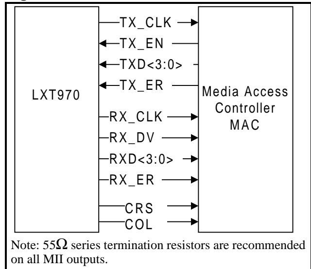
Figure 4: MII Data Interface
