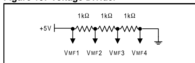
Figure 19: Voltage Divider
