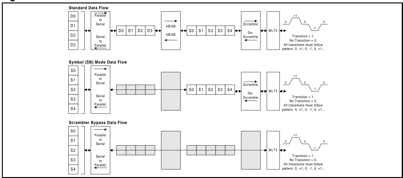
Figure 13: 100BASE-TX Data Flow
