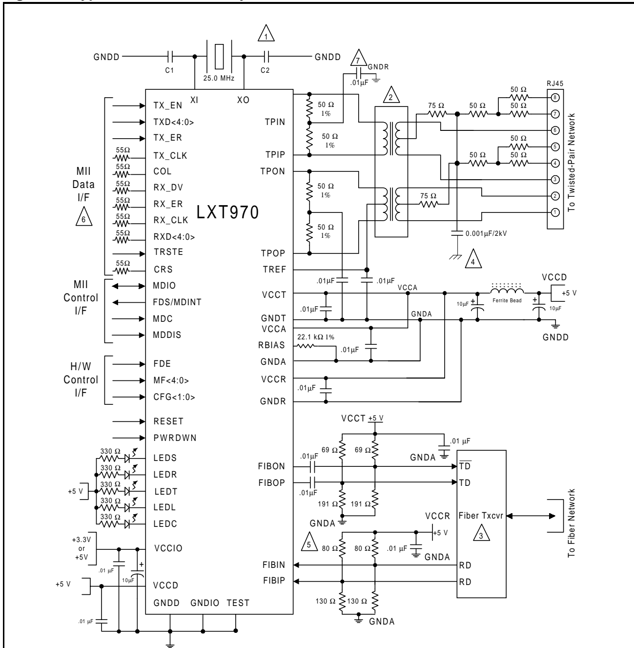
Figure 20: Typical Interface Circuitry
