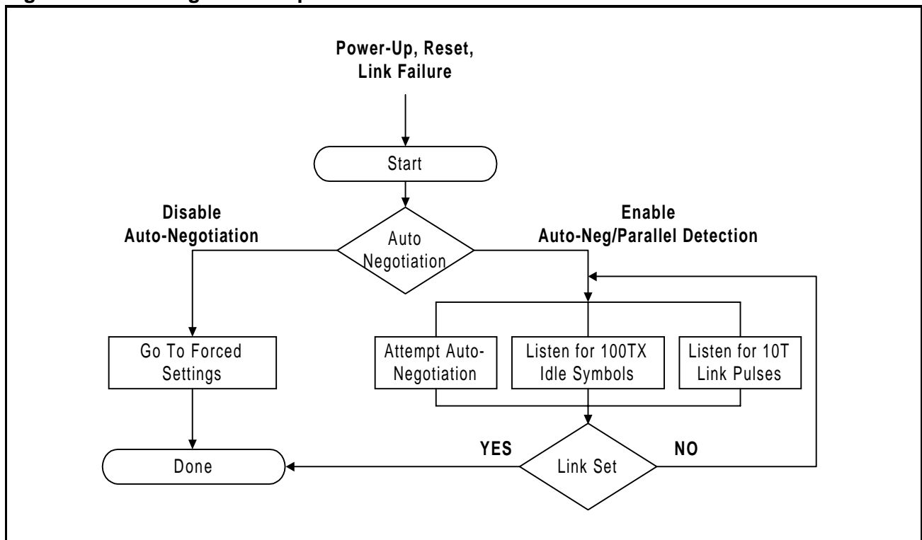
Figure 11: Auto-Negotiation Operation
