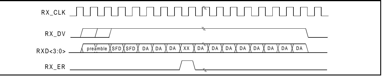
Figure 17: 100BASE-TX Transmission with No Errors
