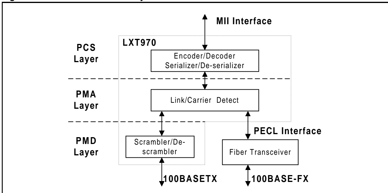
Figure 14: LXT970 Protocol Sublayers
