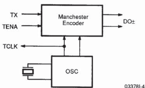
Figure 1. Transmit Section
