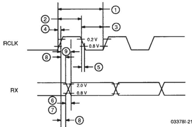
RCLK and RX Timing
