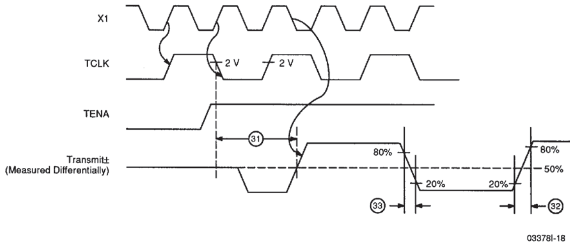
Transmit Timing (at start of packet)
