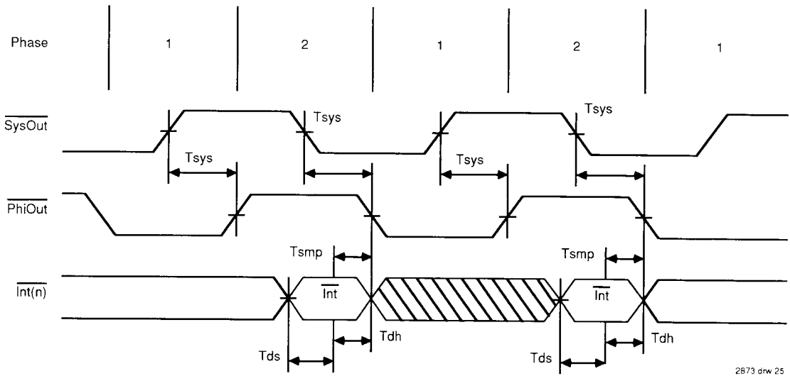
Figure 22. Interrupt Timing
