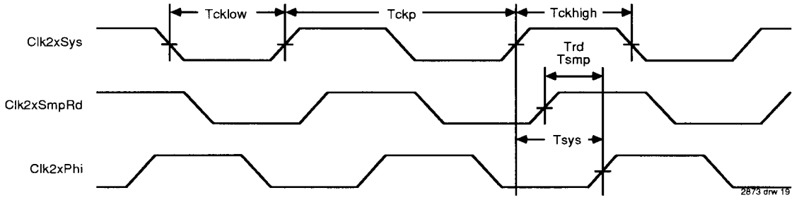
Figure 16. Input Clock Timing
