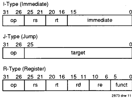
Figure 11. IDT79R3001 Instruction Formats
