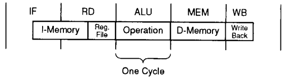
Figure 2. IDT79R3001 Five-Stage Pipeline
