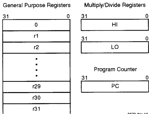
Figure 10. IDT79R3001 Registers
