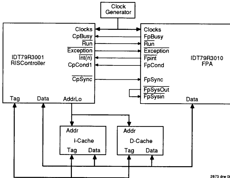
Figure 8. IDT79R3001 Interface to IDT79R3010 Floating Point Co-Processor
