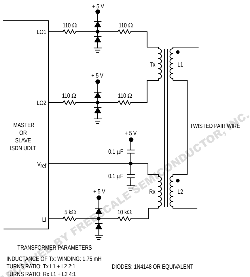
Figure 4. Interface to Twisted Pair Wire
