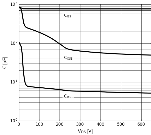
Figure 5. Typical Capacitance
