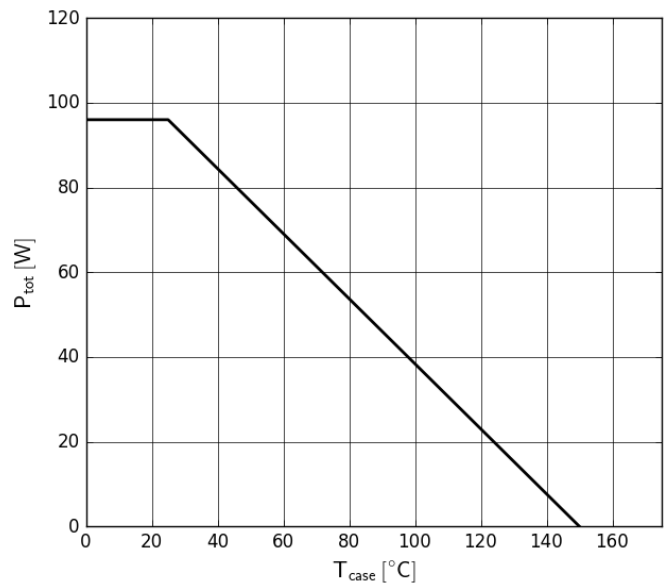
Figure 14. Power Dissipation
