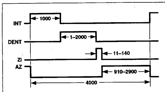
Figure 4 Conversion Timing During Normal Operation
