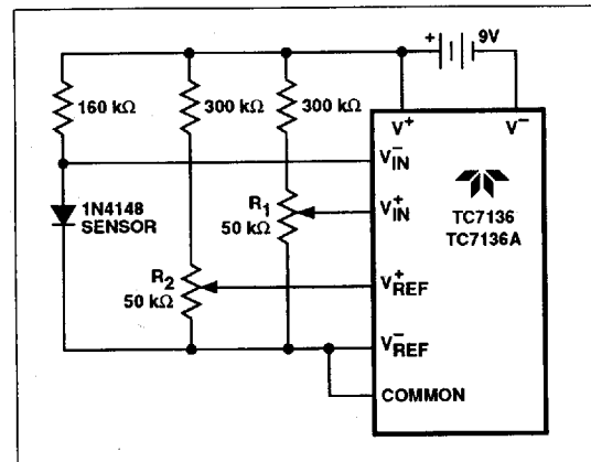
Figure 13 Temperature Sensor
