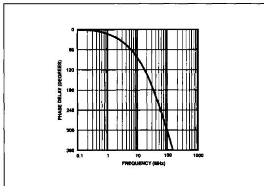
FIGURE 5: Preamplifier Phase Response
