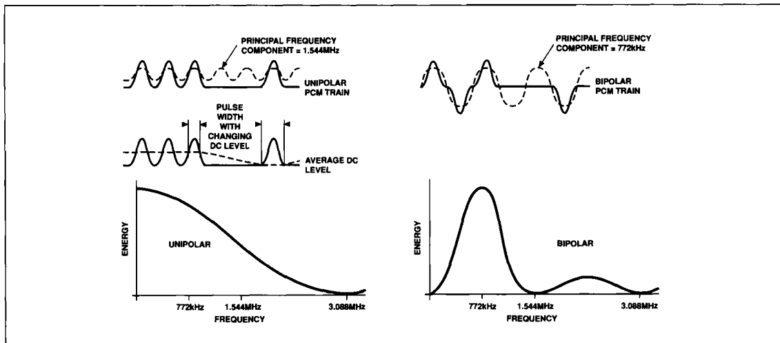
FIGURE 1: Energy Spectra of Bipolar and Unipolar Pulse Trains
