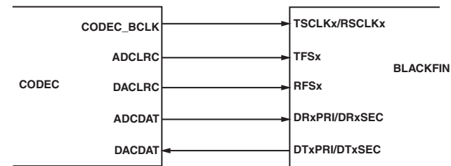
Figure 24. Master Mode
