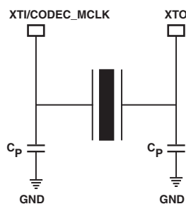
Figure 18. Crystal Connection
