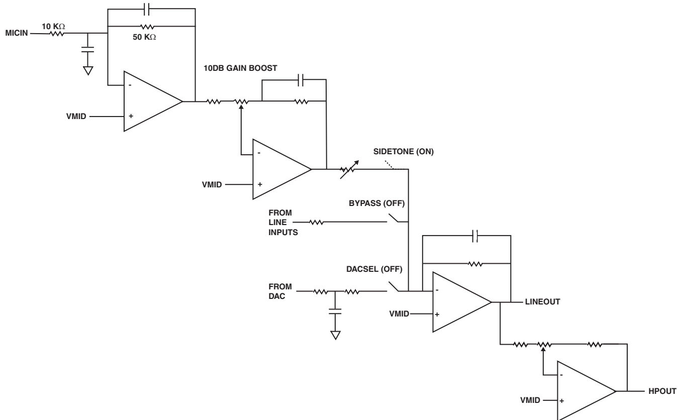
Figure 17. Sidetone Mode
