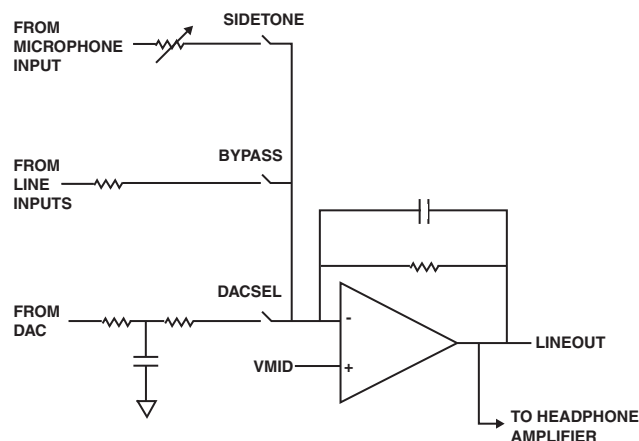
Figure 12. Line Output
