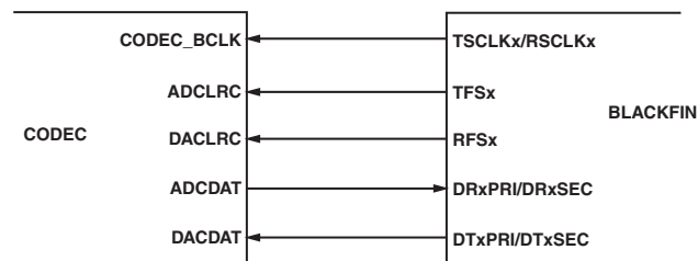
Figure 25. Slave Mode
