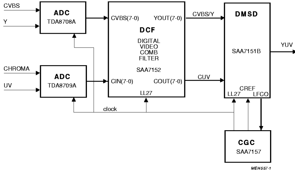
Fig.3 System environment.
