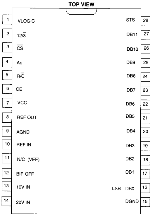
28-LEAD DIP
