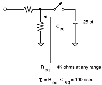
Figure 9 - Equivalent HADC674Z Input Circuit
