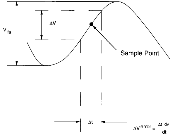
and V_{fs} is the full scale voltage) Figure 10 - Aperture Uncertainty
