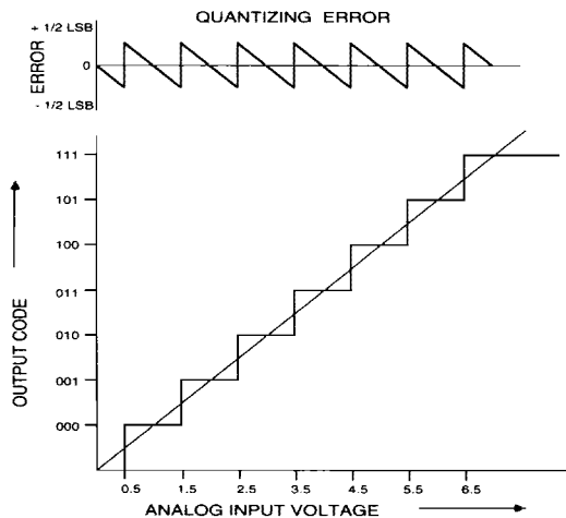
Figure 7 - Quantizing Error
