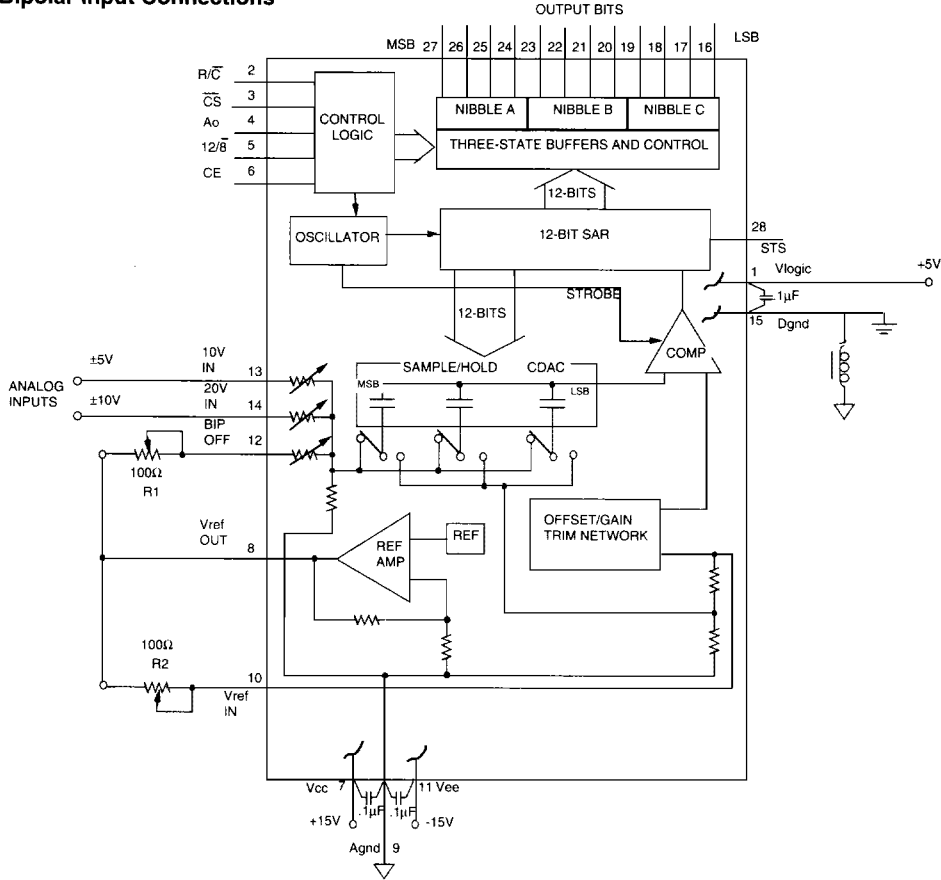
Figure 12 - Bipolar Input Connections
