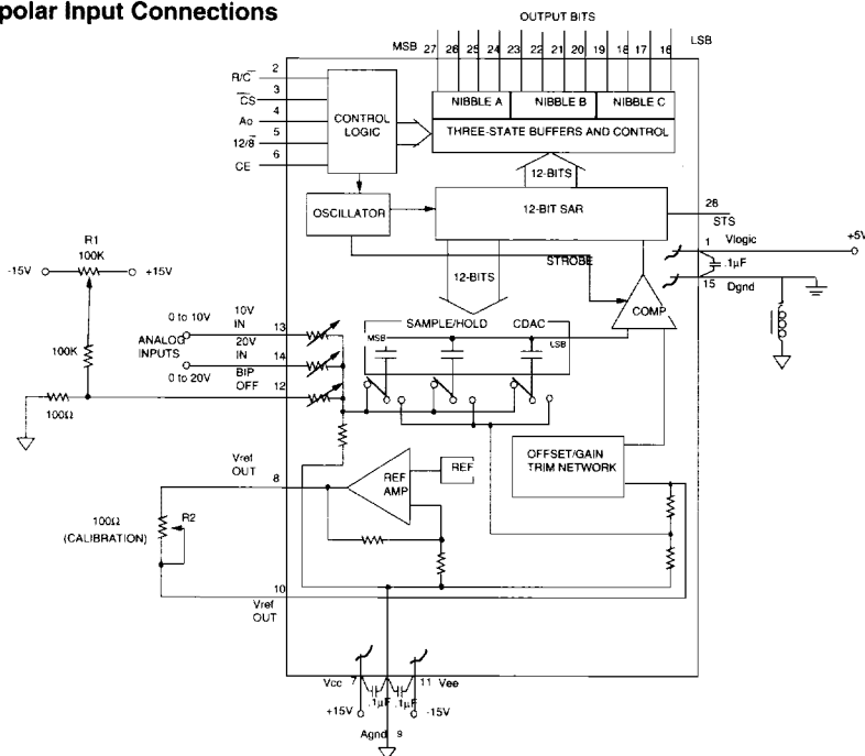
Figure 11 - Unipolar Input Connections
