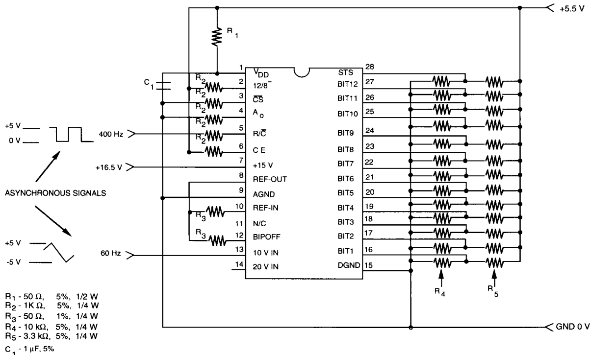
Figure 15 - Burn-In Schematic
