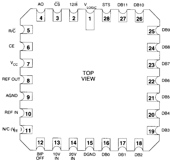
28-LEAD LCC
