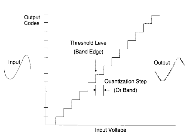
Figure 5 - Static Input Conditions
