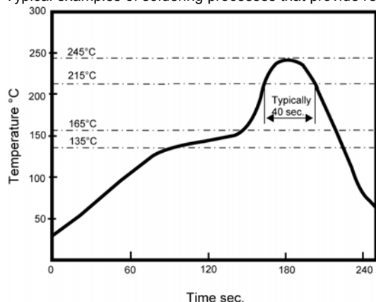
Fig. 2 Infrared soldering profile
