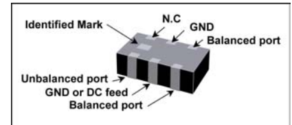
Fig 1. Outline of 2.4GHz Balun
