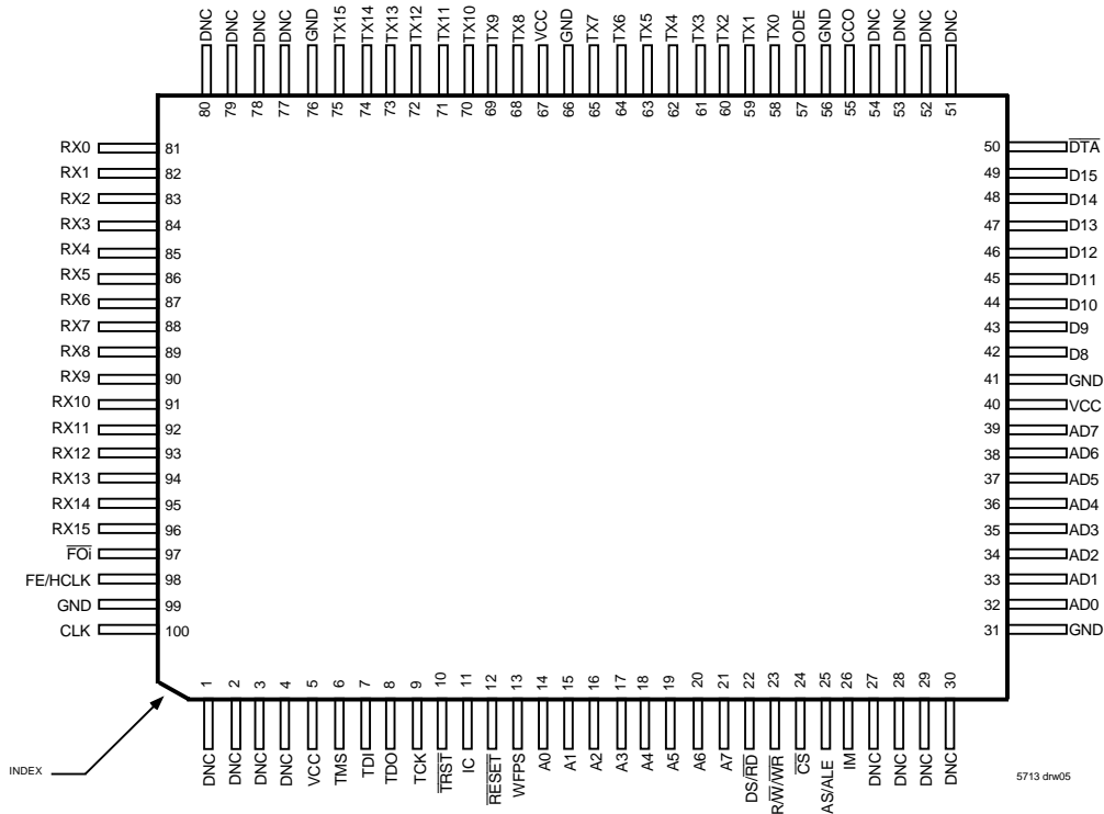
TQFP (PK100-1, order code: TF) TOP VIEW
