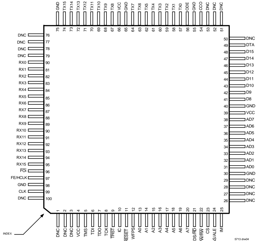
TQFP (PN100-1, order code: PF) TOP VIEW
