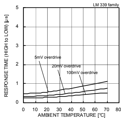
Fig. 40 Response Time (High to Low) – Ambient Temperature (VCC=5[V], VRL=5[V], RL=5.1[kΩ])
