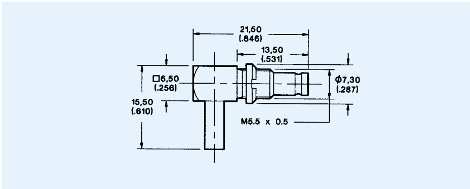
Mounting Plan J (Page 108). Maximum Panel Thickness 2,00 (0.078) Assembly Instruction BBAI-1252 (Apply ITT Cannon Sales Dept.)
