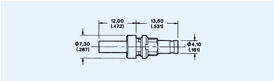
Mounting Plan K (Page 108). Maximum Panel Thickness 1,50 (0.059) Assembly Instruction BBAI-1250 (Apply ITT Cannon Sales Dept.)
