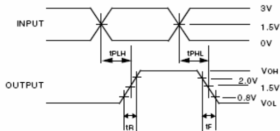
Propagation Delay
