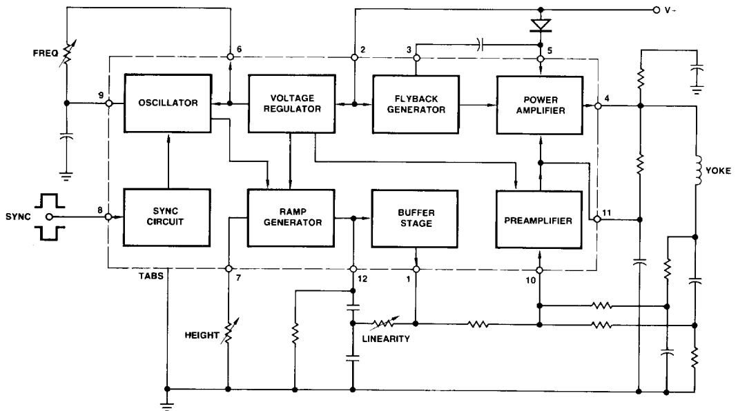
TDA1170
