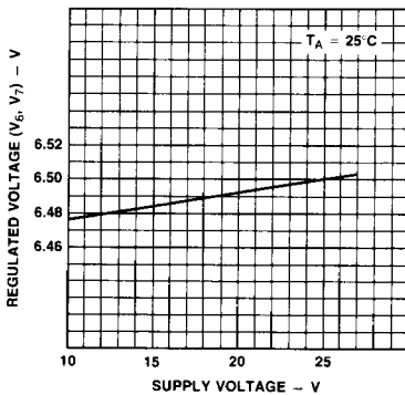
REGULATED VOLTAGE ( V_6, V_7 ) AS A FUNCTION OF SUPPLY VOLTAGE
