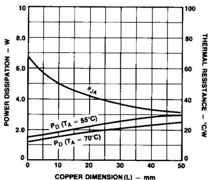
MAXIMUM POWER DISSIPATION AND THERMAL RESISTANCE AS A FUNCTION OF COPPER LENGTH (L)
