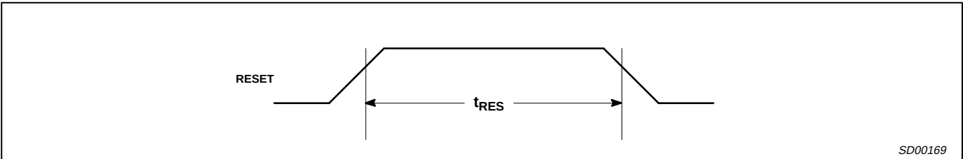
Figure 7. Reset Timing
