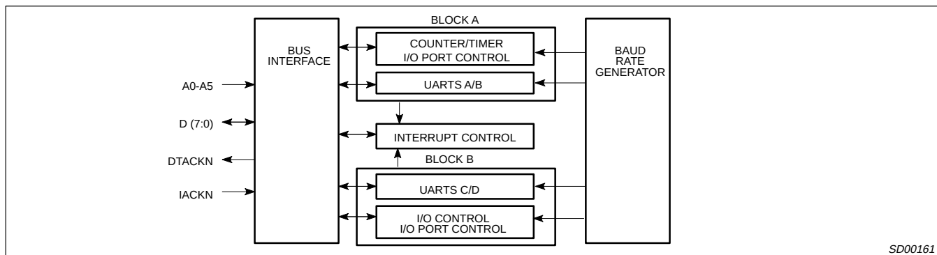
Figure 1. Channel Architecture
