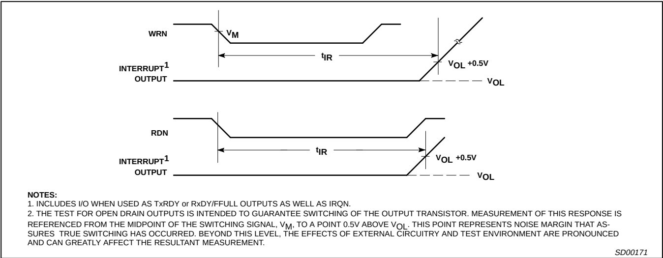
Figure 9. Interrupt Timing
