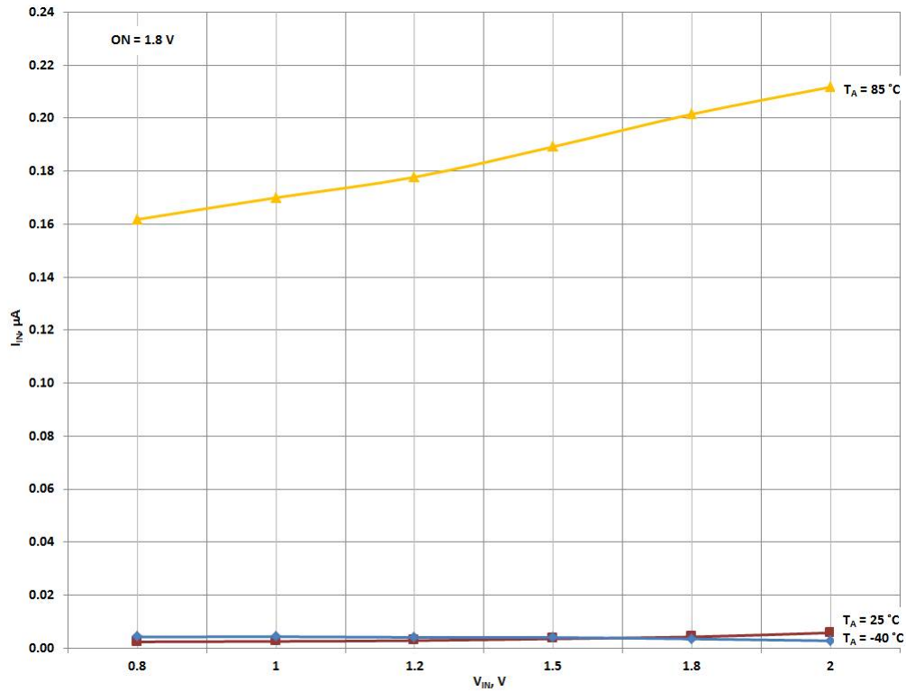
I_{IN} when ON = 1.8 V vs. V_{IN} and Temperature
