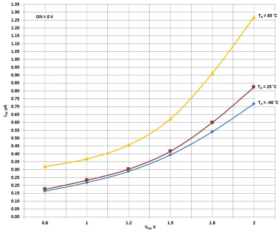
I_{IN} when OFF vs. V_{IN} and Temperature
