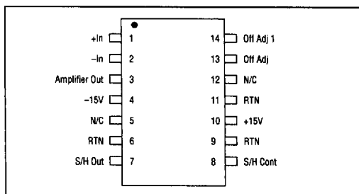
Figure 3. SHA2410 Pinout.
