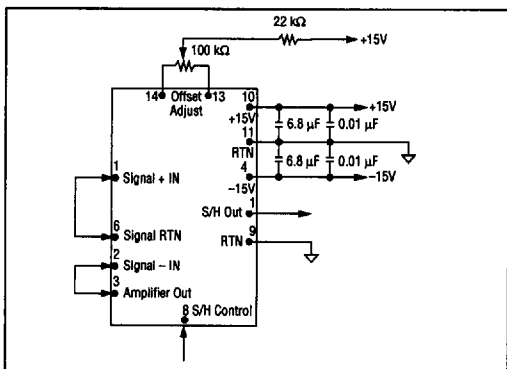
Figure 5. Offset Adjustment.
