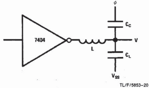
FIGURE 5. Clock Coupling
