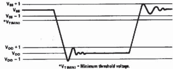
FIGURE 3. Clock Waveform
