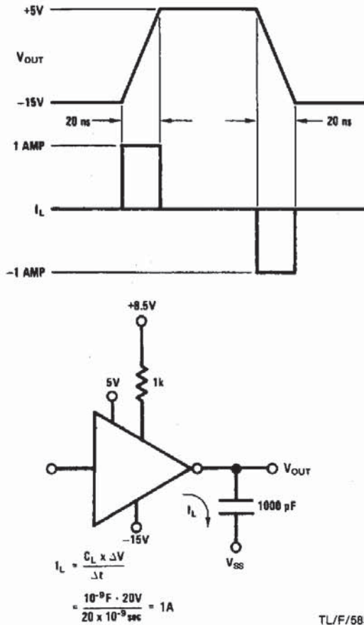
FIGURE 4. Clock Waveforms (Voltage and Current)
