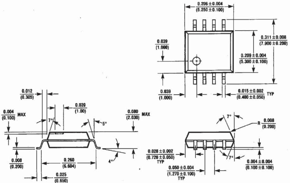
8-Lead Surface Mount Package Order Number DS0026CL
