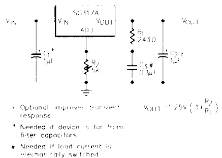
FIGURE 19 - 1.2V-25V ADJUSTABLE REGULATOR
