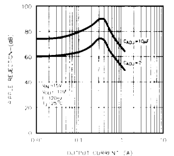
FIGURE 9. RIPPLE REJECTION VS. OUTPUT CURRENT
