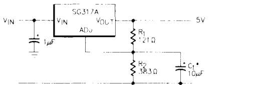
FIGURE 21 - IMPROVING RIPPLE REJECTION
