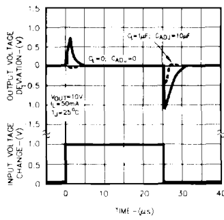
FIGURE 11. LINE TRANSIENT RESPONSE
