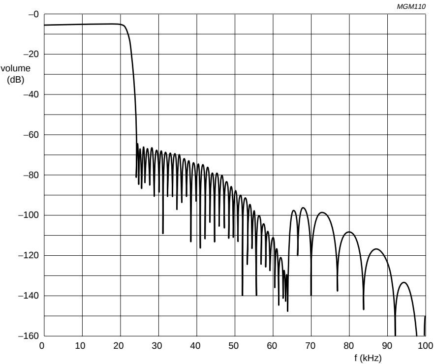
Fig.6 Overall filter characteristics of the UDA1331H.
