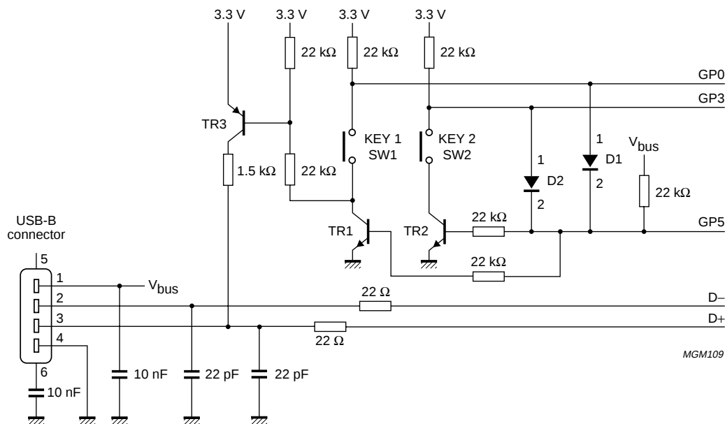
Fig.4 Diode matrix selection.
