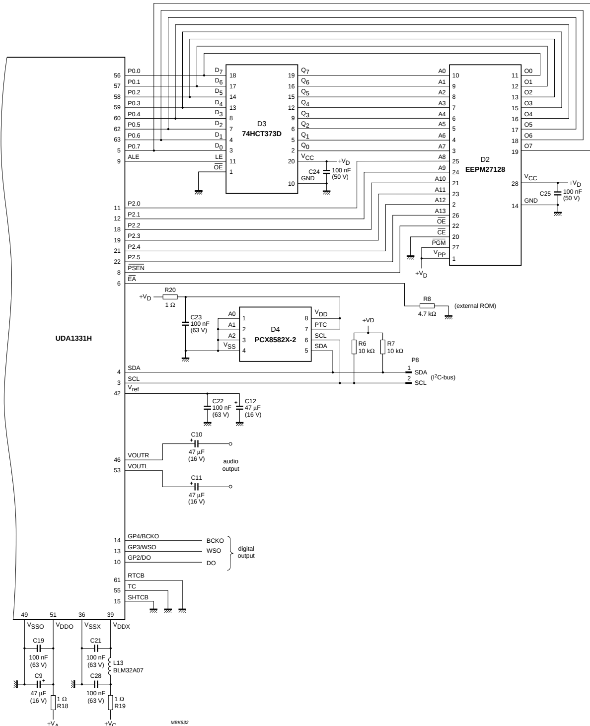
Fig.10 Application diagram (continued from Fig.9).
