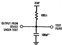
FIGURE 7. BUSY, CBRQ LOAD CIRCUIT
