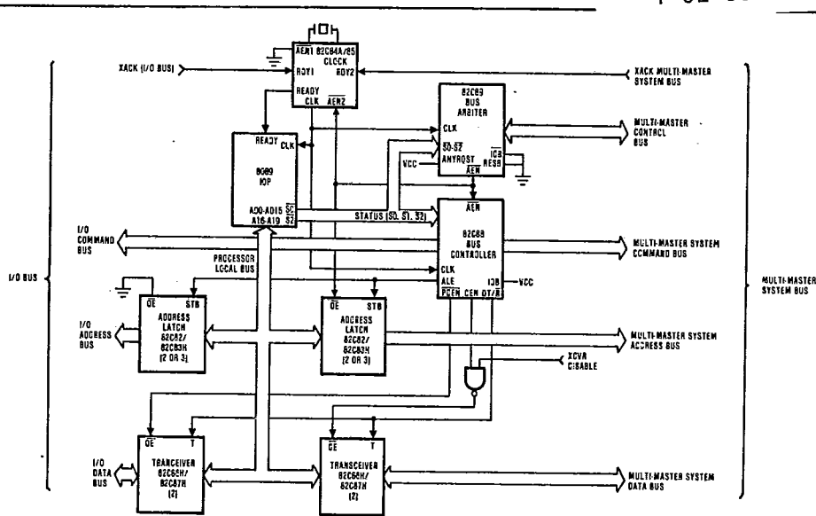
FIGURE 5. TYPICAL MEDIUM COMPLEXITY IOB SYSTEM
