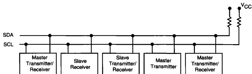
Typical System Configuration (Figure 11)
