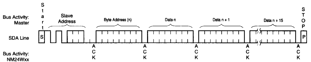
Page Write (Figure 6)
