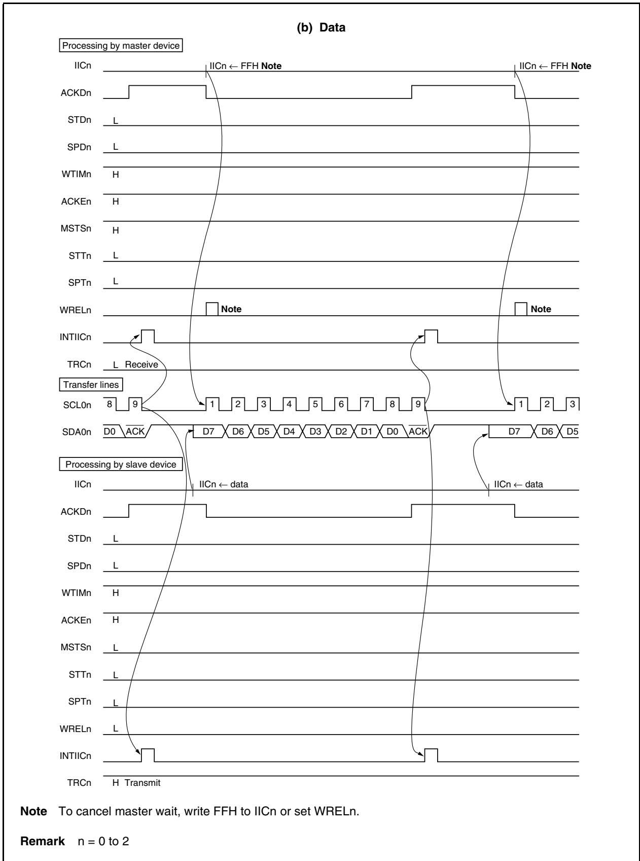
Figure 17-22. Example of Slave to Master Communication (When 9-Clock Wait Is Selected for Both Master and Slave) (2/3)
