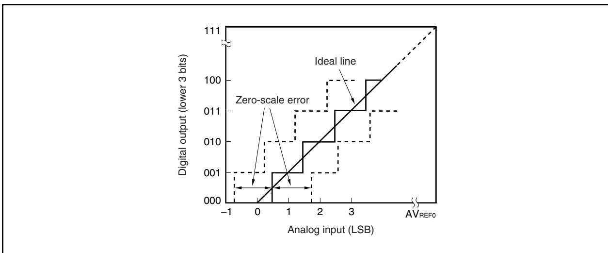
Figure 13-17. Zero-Scale Error
