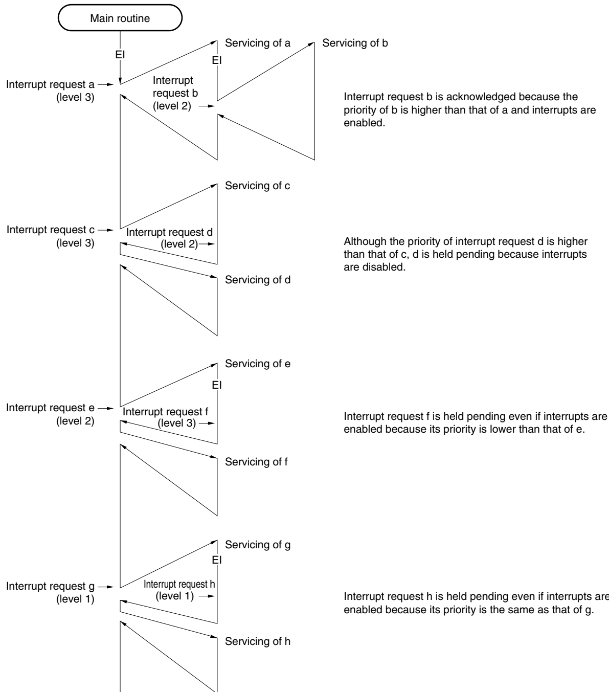
Figure 22-6. Example of Processing in Which Another Interrupt Request Signal Is Issued While an Interrupt Is Being Serviced (1/2)
