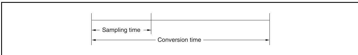
Figure 13-21. Sampling Time
