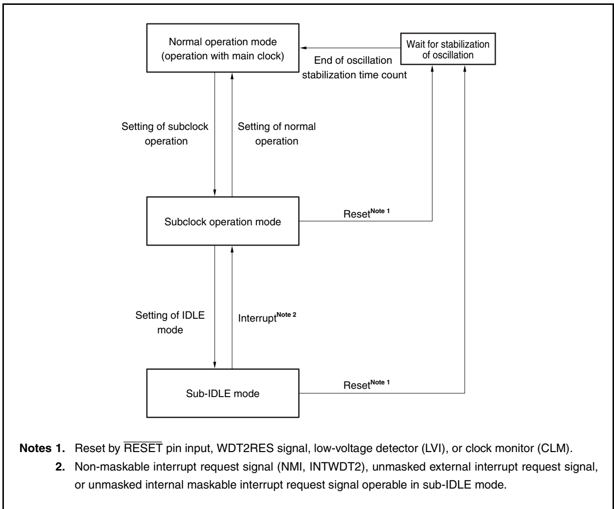
Figure 24-2. Status Transition (During Subclock Operation)
