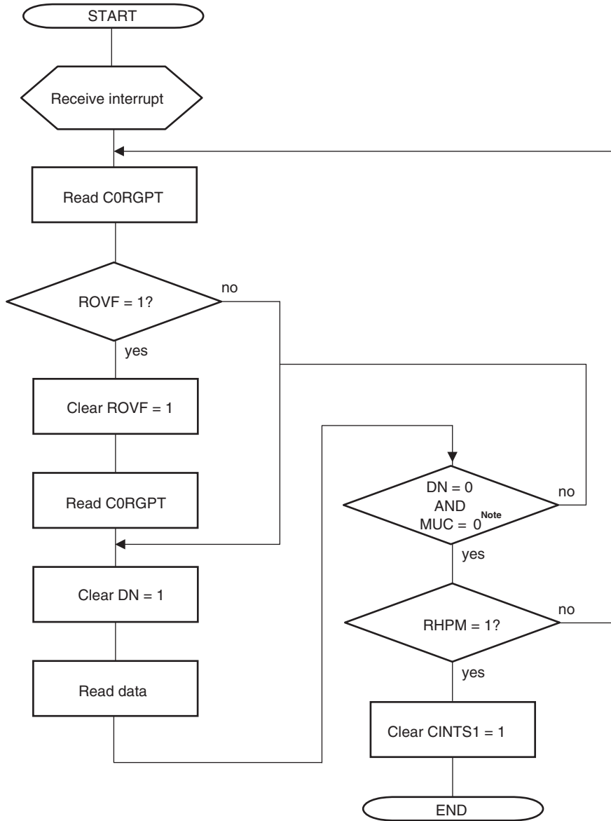
Figure 19-56. Reception via Interrupt (C0RGPT)
