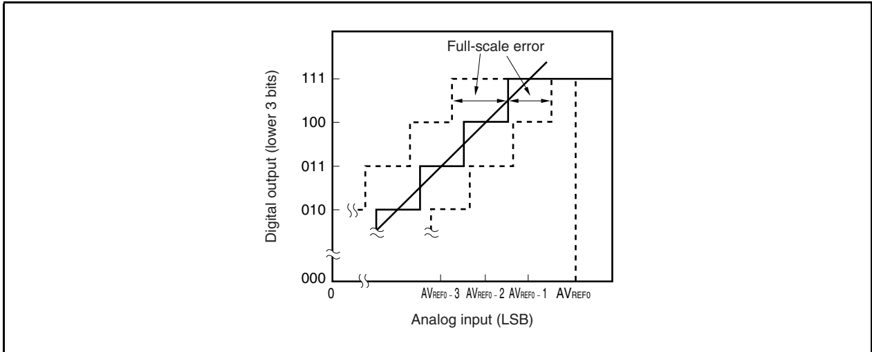
Figure 13-18. Full-Scale Error
