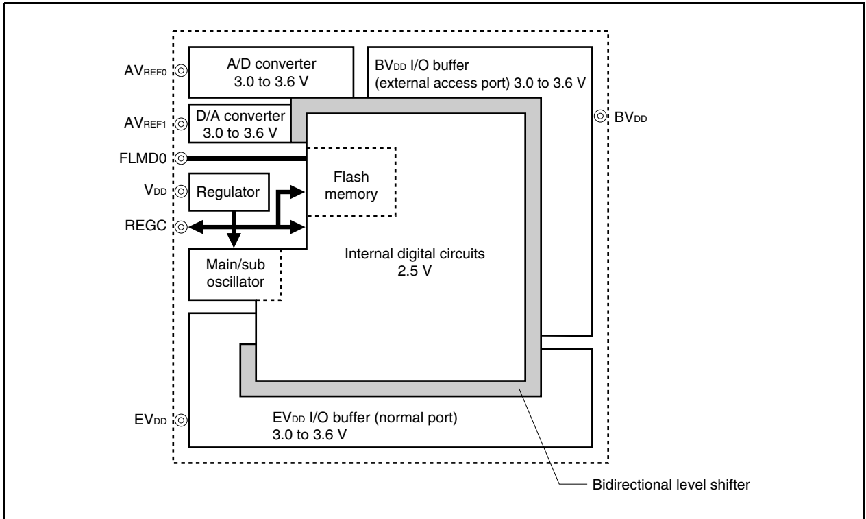
Figure 26-1. Regulator
