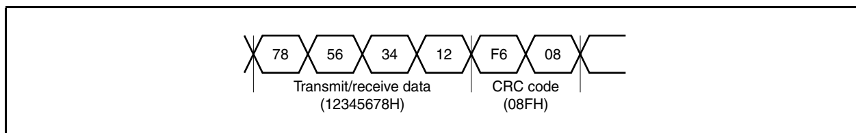
Figure 21-5. CRC Transmission Example
