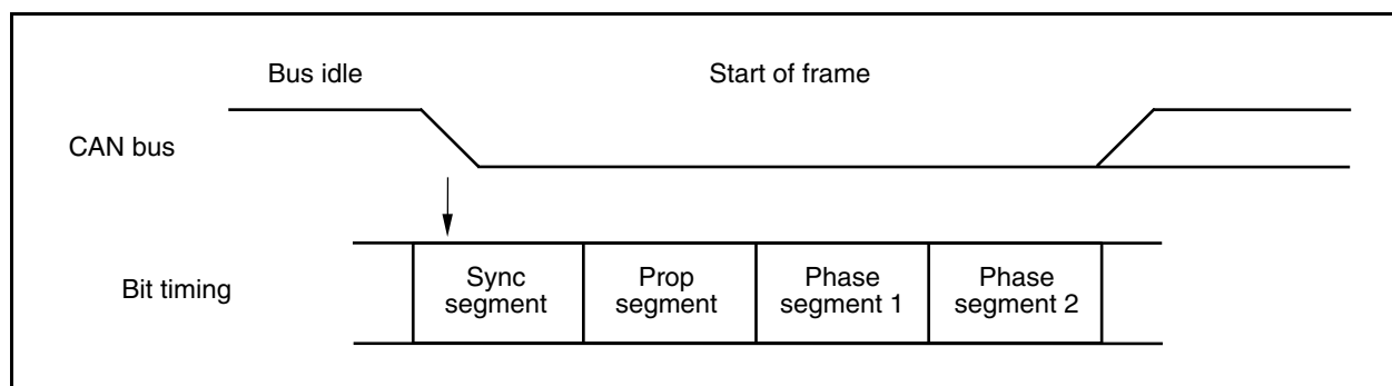
Figure 19-18. Adjusting Synchronization of Data Bit
