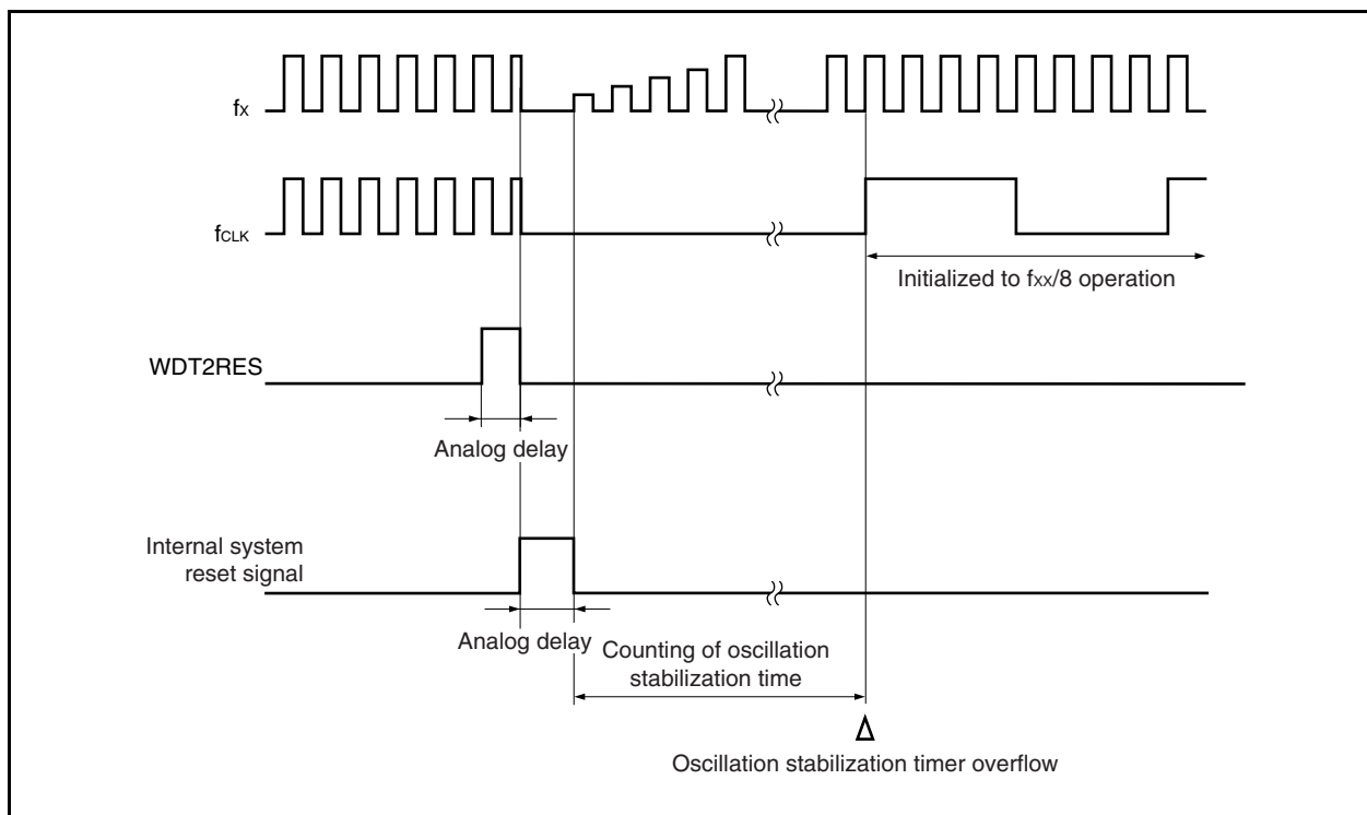
Figure 25-3. Timing of Reset Operation by WDT2RES Signal Generation
