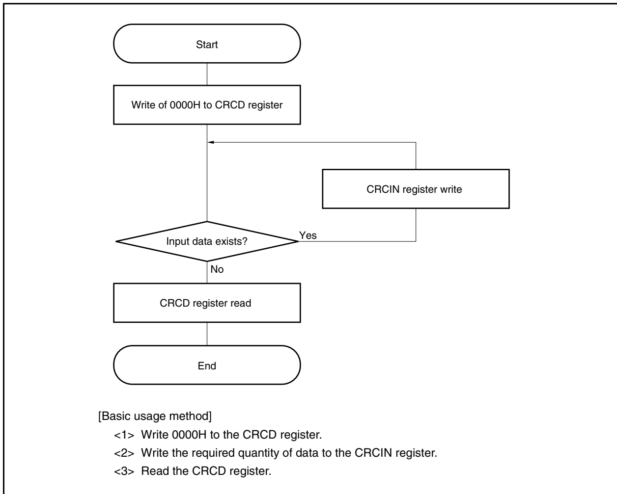
Figure 21-4. CRC Operation Flow
