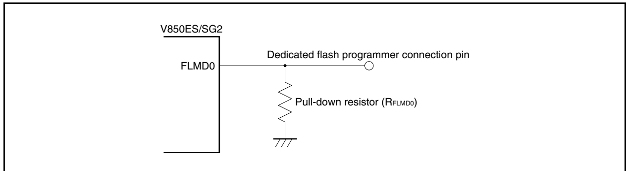
Figure 28-5. FLMD0 Pin Connection Example
