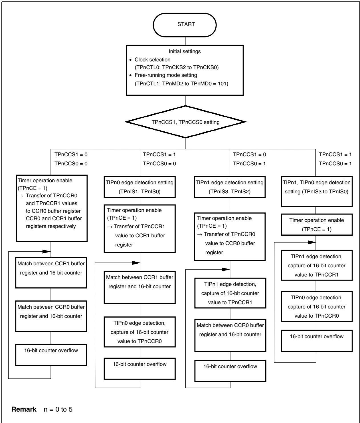
Figure 7-16. Flowchart of Basic Operation in Free-Running Mode
