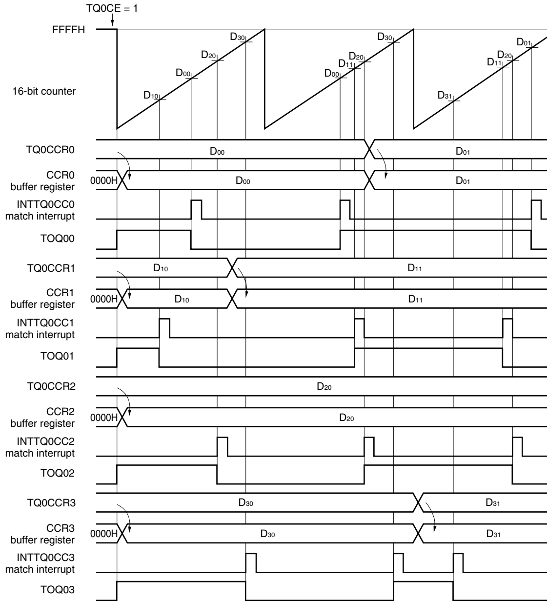
Figure 8-17. Basic Operation Timing in Free-Running Mode (TQ0CCS3 = 0, TQ0CCS2 = 0, TQ0CCS1 = 0, TQ0CCS0 = 0)
