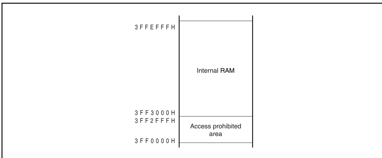
Figure 3-12. Internal RAM Area (48 KB)
