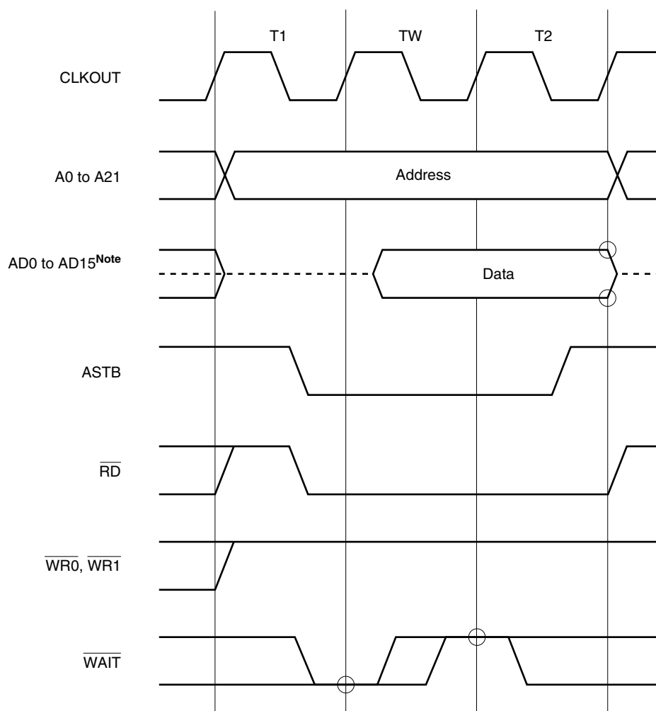
Figure 5-14. When Wait State (1 Wait) Is Inserted
