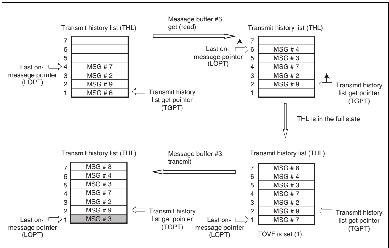
Figure 19-37. Transmit History List
