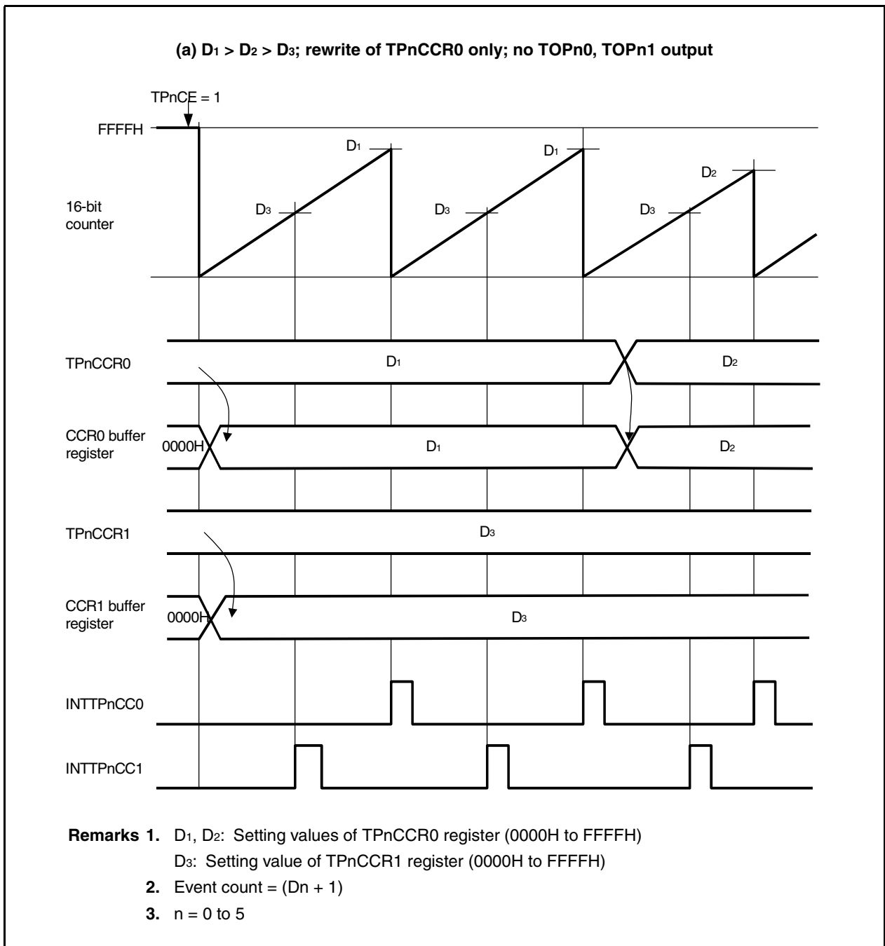
Figure 7-9. Basic Operation Timing in External Event Count Mode (1/2)
