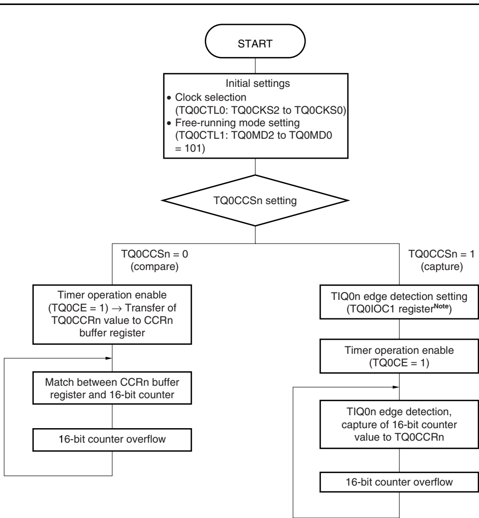
Figure 8-16. Flowchart of Basic Operation in Free-Running Mode
