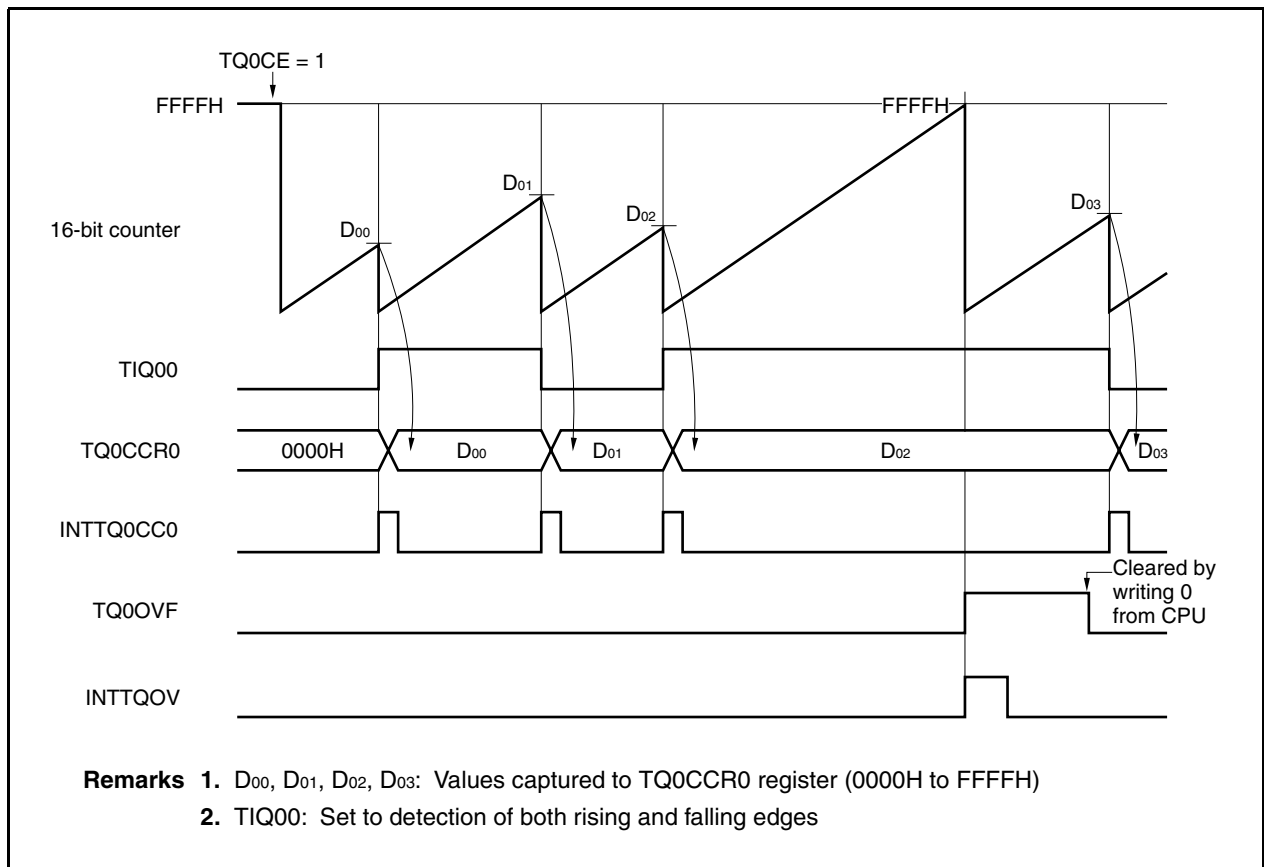
Figure 8-22. Basic Operation Timing in Pulse Width Measurement Mode
