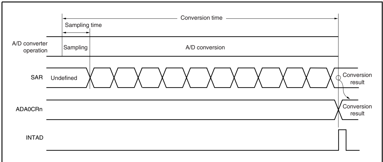
Figure 13-3. A/D Converter Basic Operation
