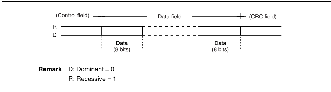
Figure 19-9. Data Field
