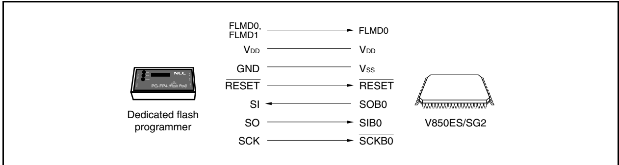
Figure 28-3. Communication with Dedicated Flash Programmer (CSIB0)
