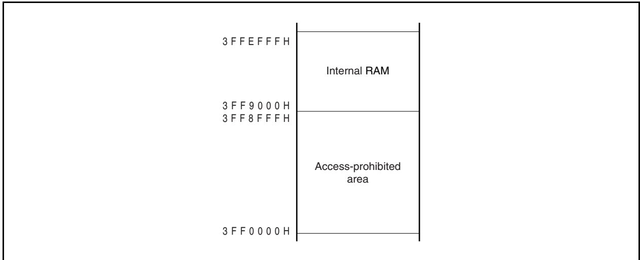
Figure 3-9. Internal RAM Area (24 KB)
