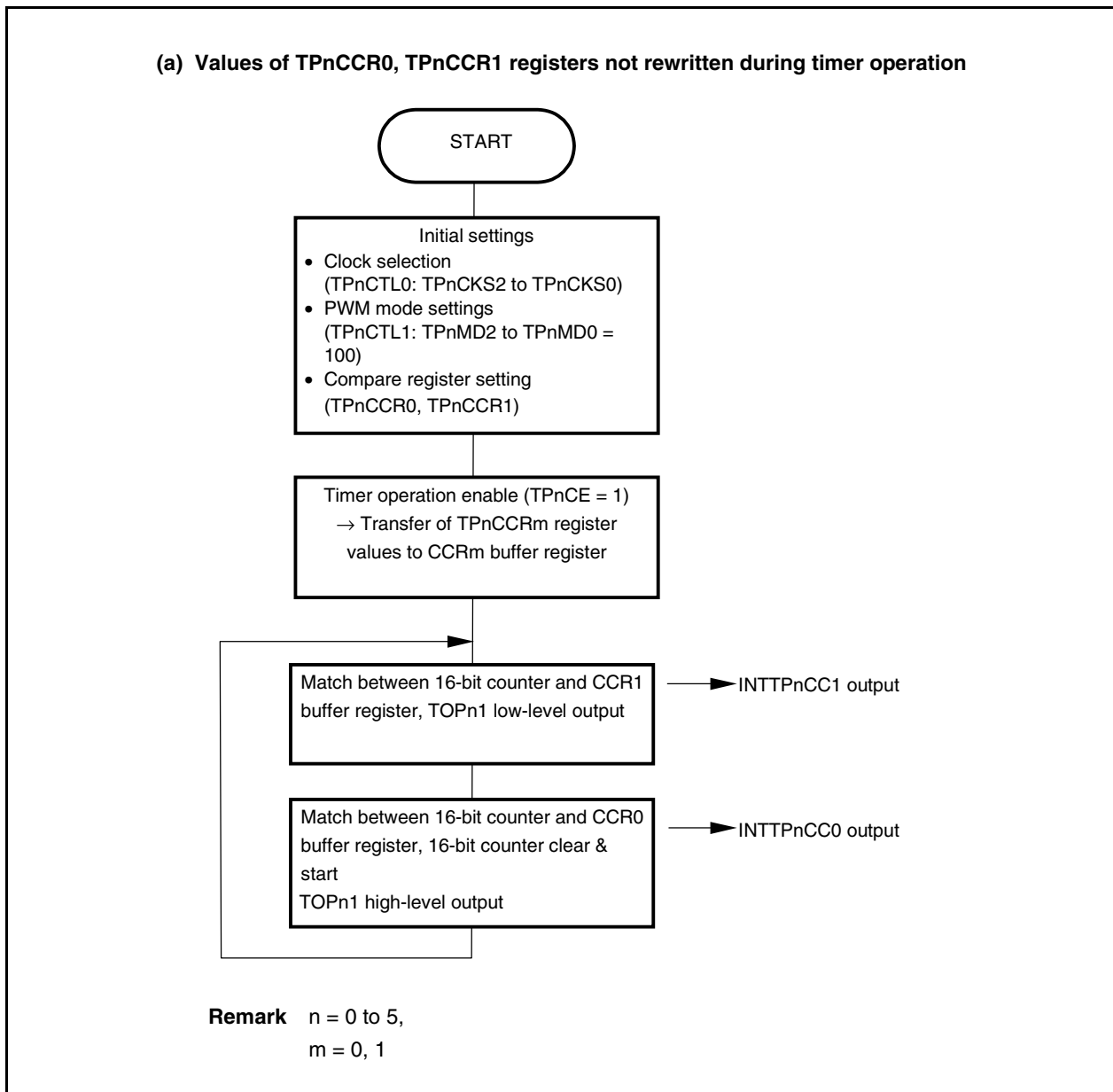
Figure 7-14. Flowchart of Basic Operation in PWM Mode (1/2)
