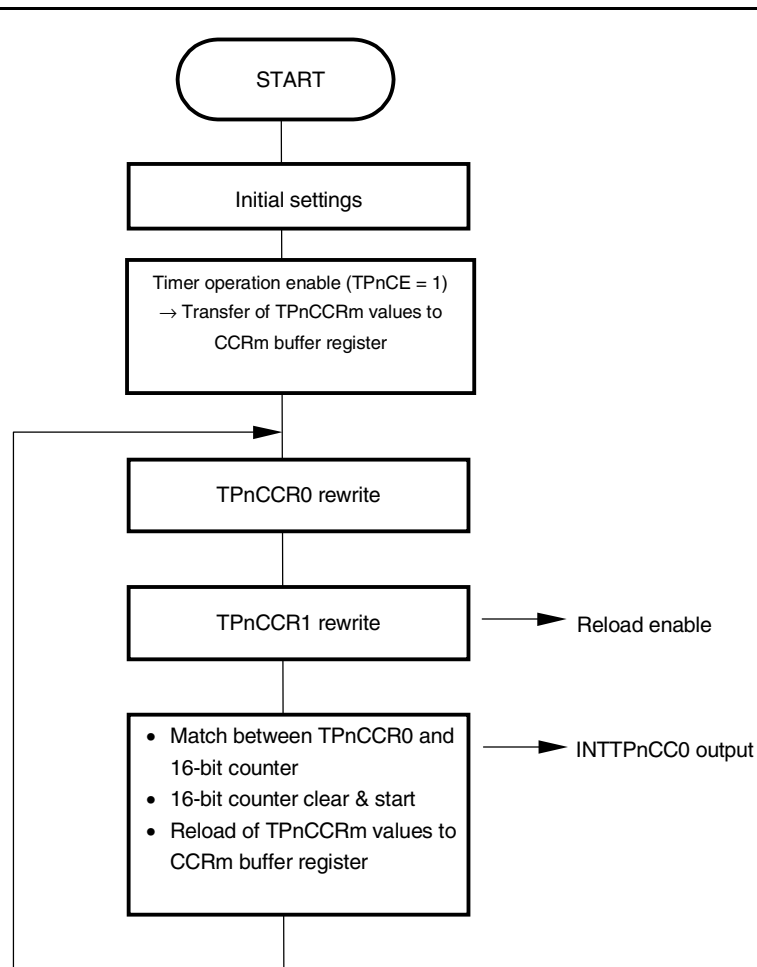
Figure 7-4. Flowchart of Basic Operation for Reload
