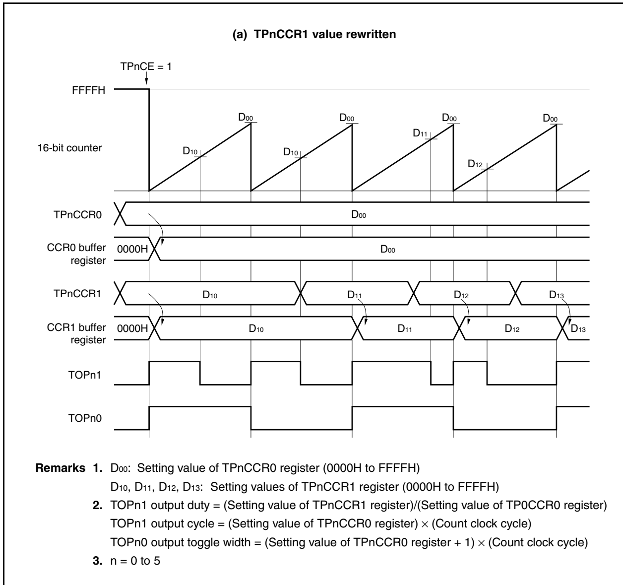
Figure 7-15. Basic Operation Timing in PWM Mode (1/2)
