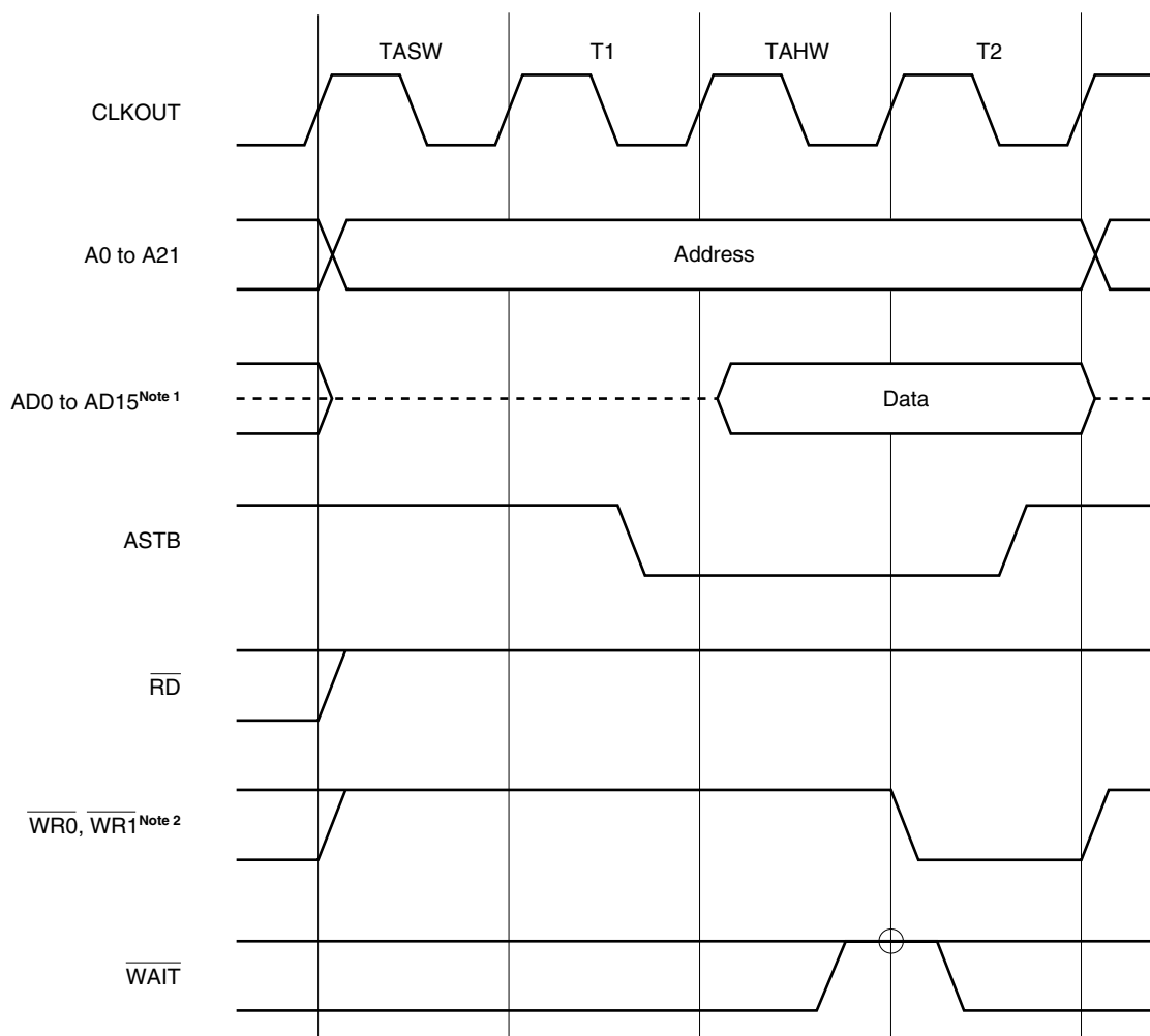
Figure 5-20. When Address Wait State Is Inserted
