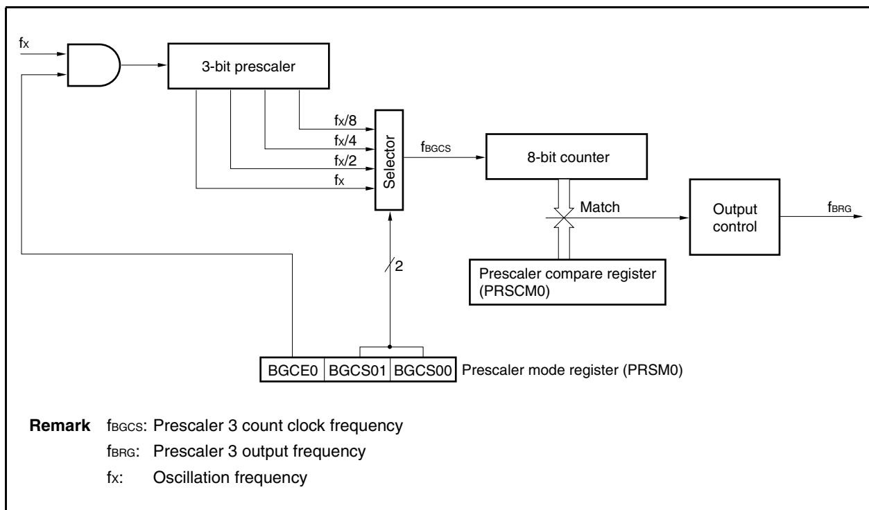
Figure 11-2. Block Diagram of Prescaler 3
