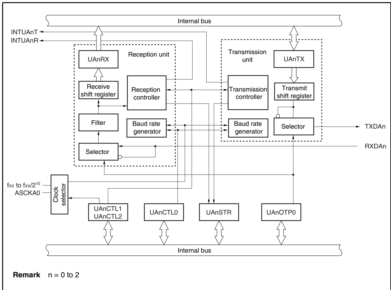
Figure 15-4. Block Diagram of Asynchronous Serial Interface n
