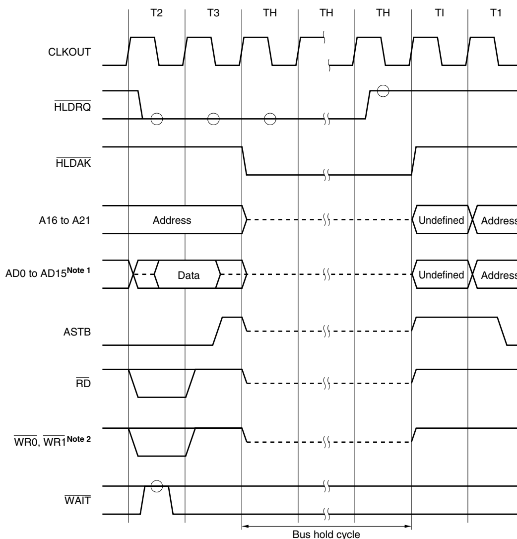
Figure 5-12. Bus Hold Cycle
