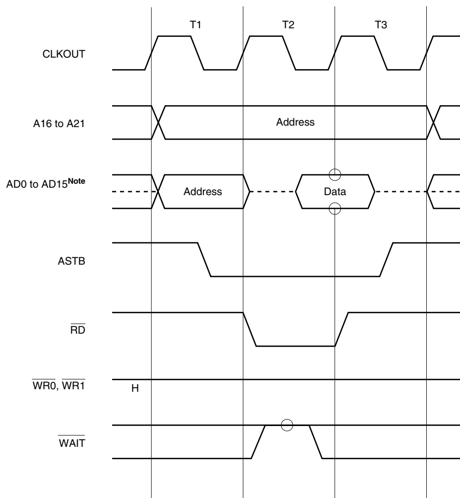
Figure 5-4. Basic Bus Cycle
