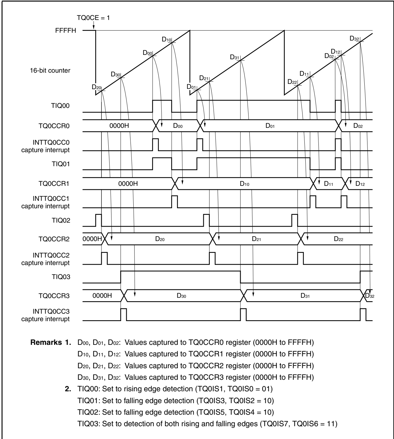
Figure 8-18. Basic Operation Timing in Free-Running Mode (TQ0CCS3 = 1, TQ0CCS2 = 1, TQ0CCS1 = 1, TQ0CCS0 = 1)
