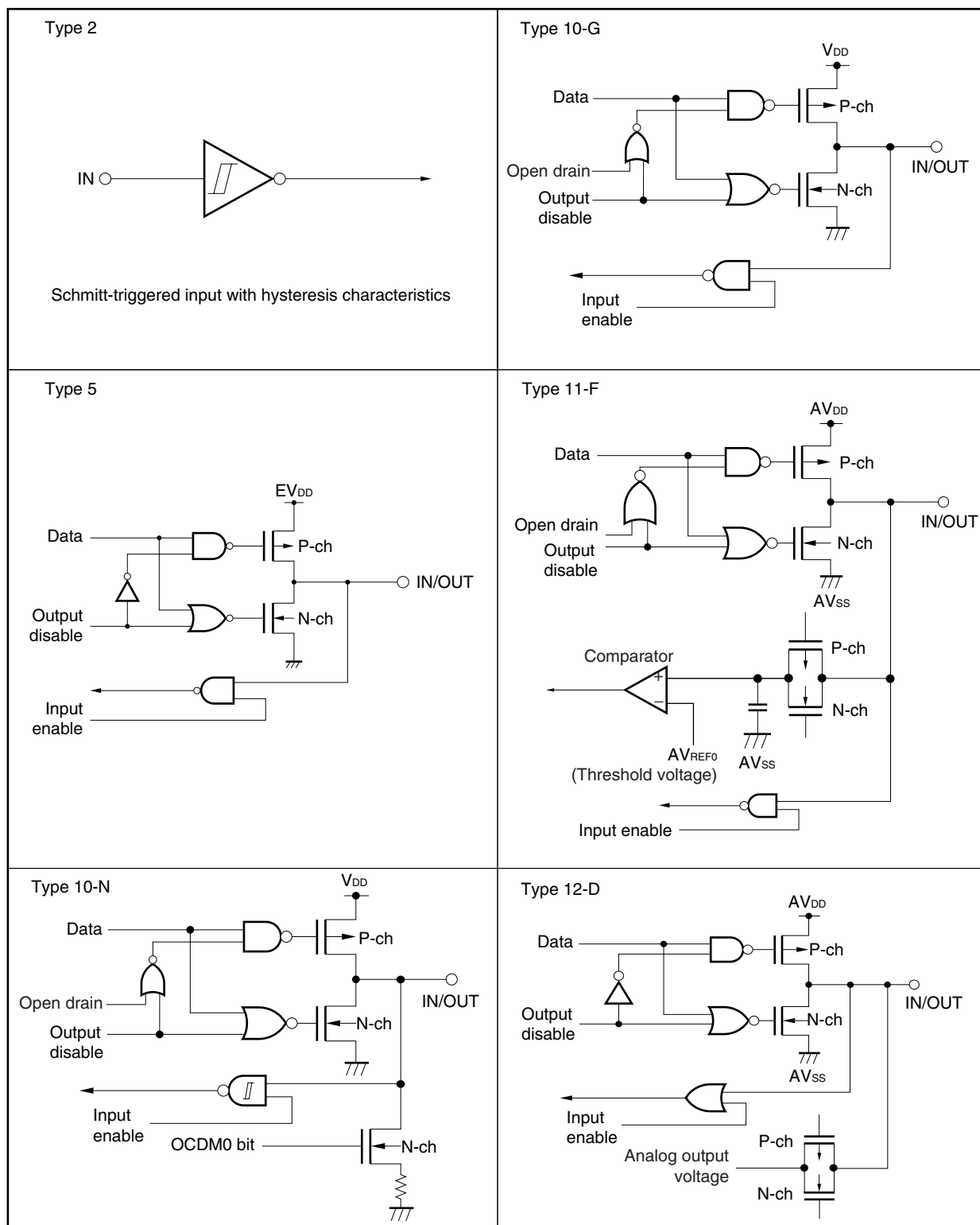
Figure 2-1. Pin I/O Circuits (1/2)
