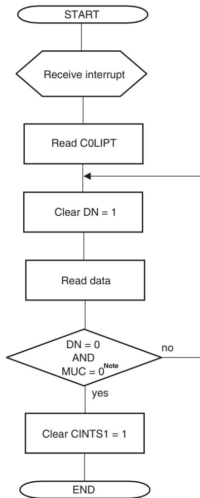
Figure 19-55. Reception via Interrupt (C0LIPT)
