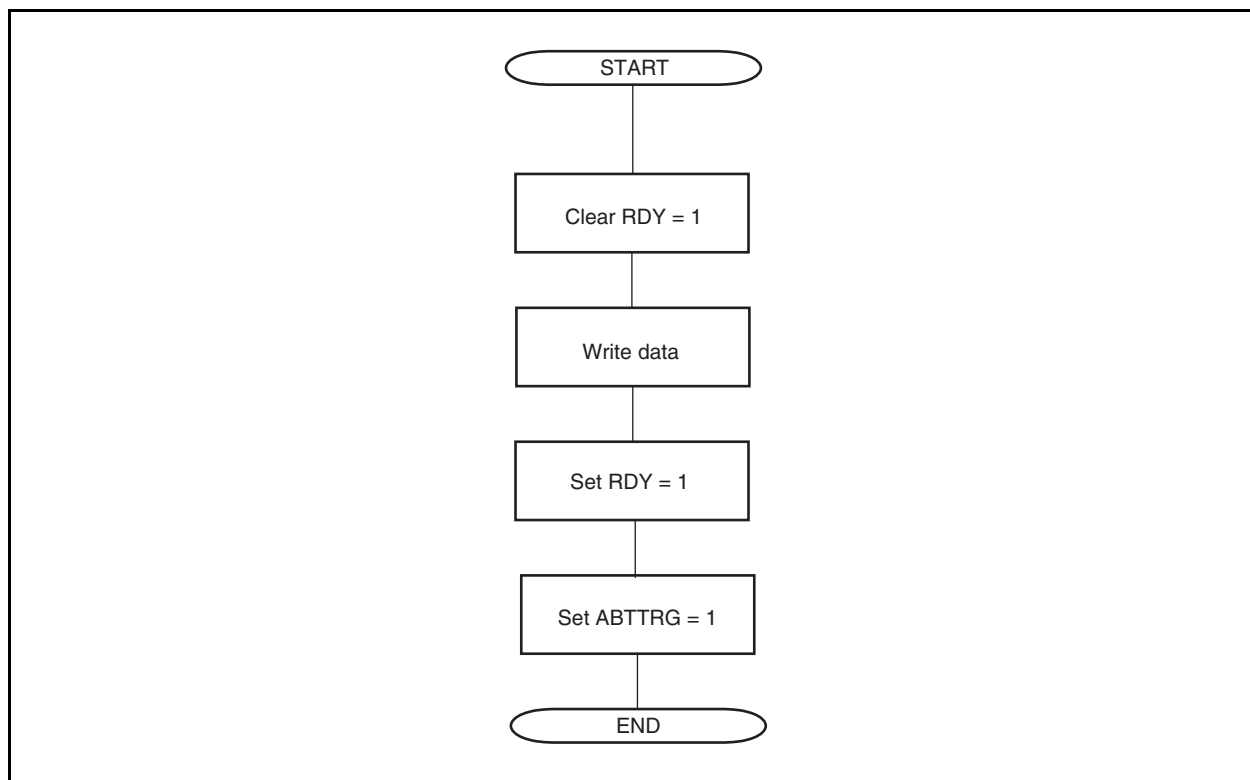
Figure 19-49. Transmit Preparation (ABT Mode)
