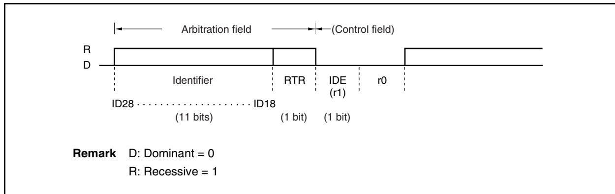
Figure 19-7. Arbitration Field (in Extended Format Mode)
