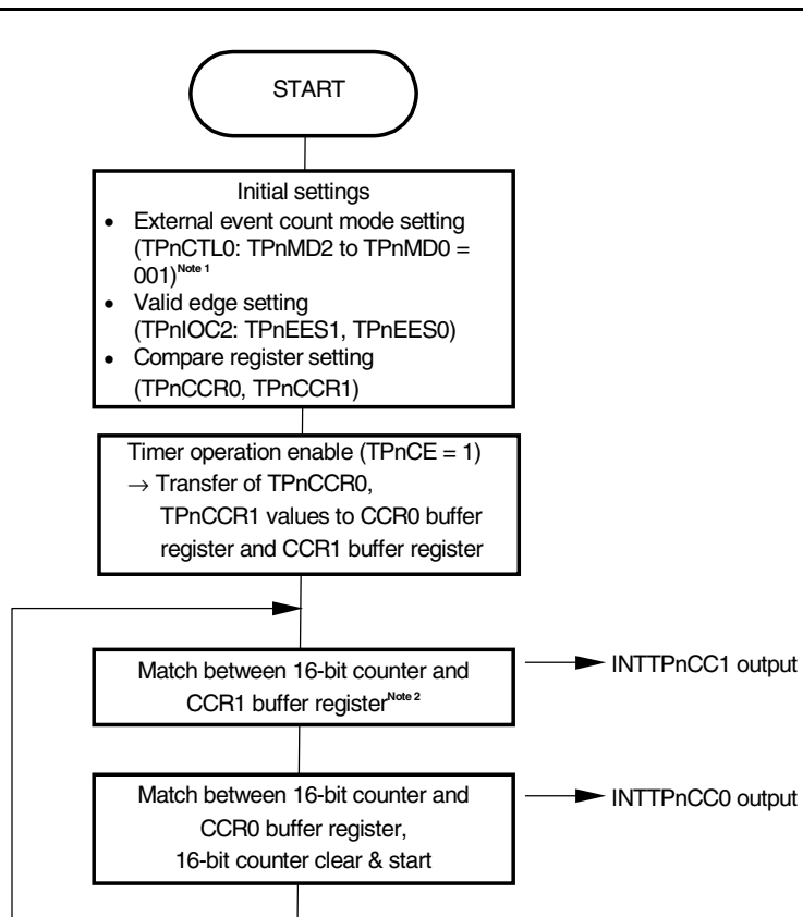
Figure 7-8. Flowchart of Basic Operation in External Event Count Mode
