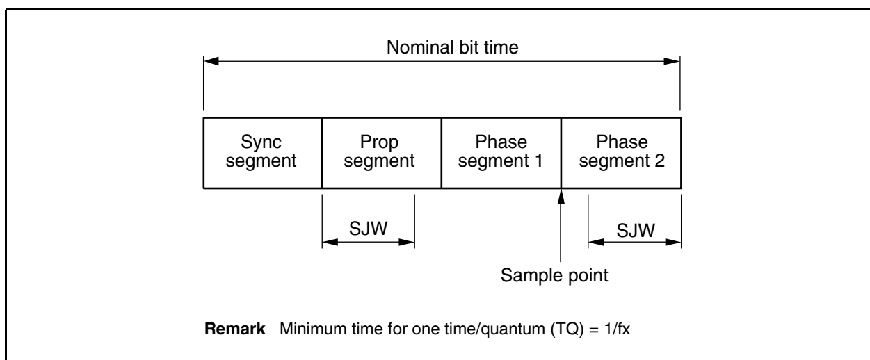
Figure 19-17. Nominal Bit Time (8 to 25 Time Quanta)
