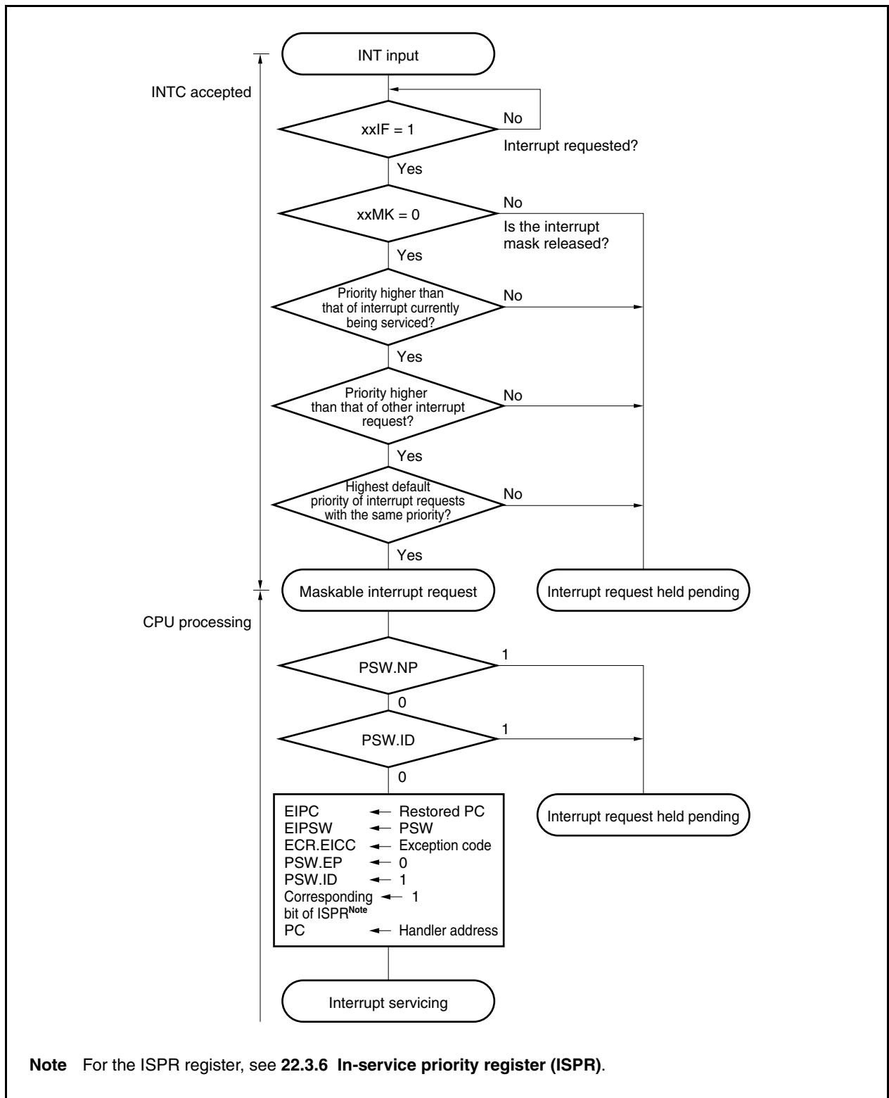
Figure 22-4. Maskable Interrupt Servicing
