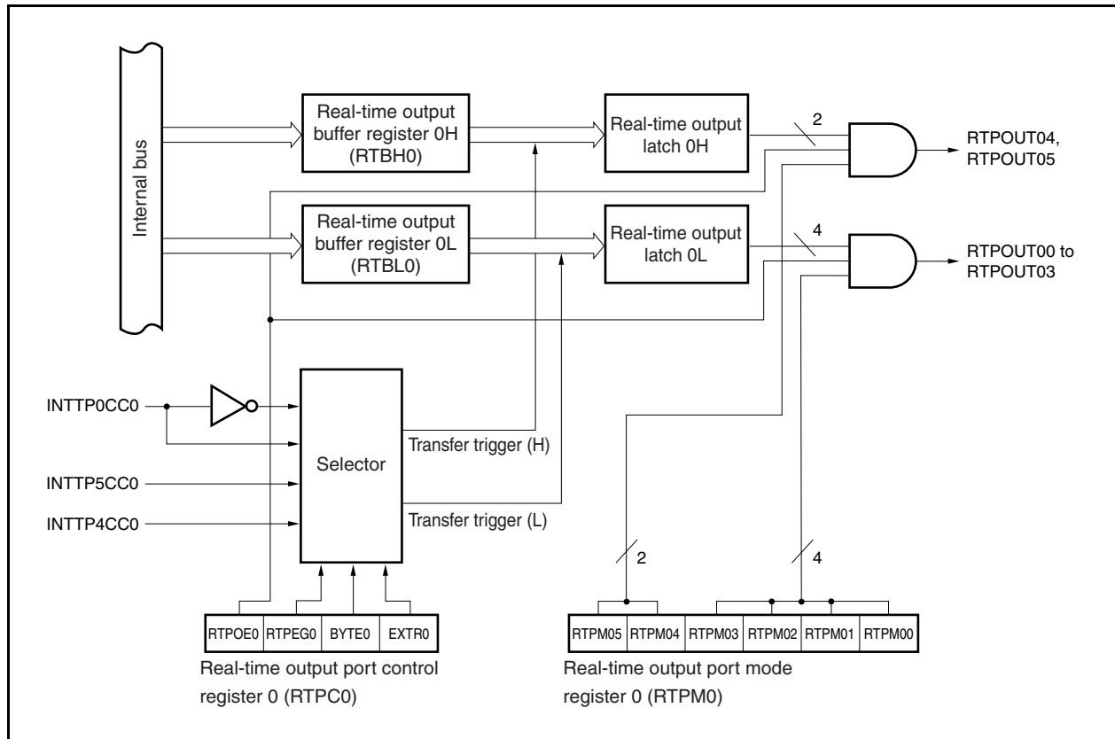
Figure 10-1. Block Diagram of RTO
