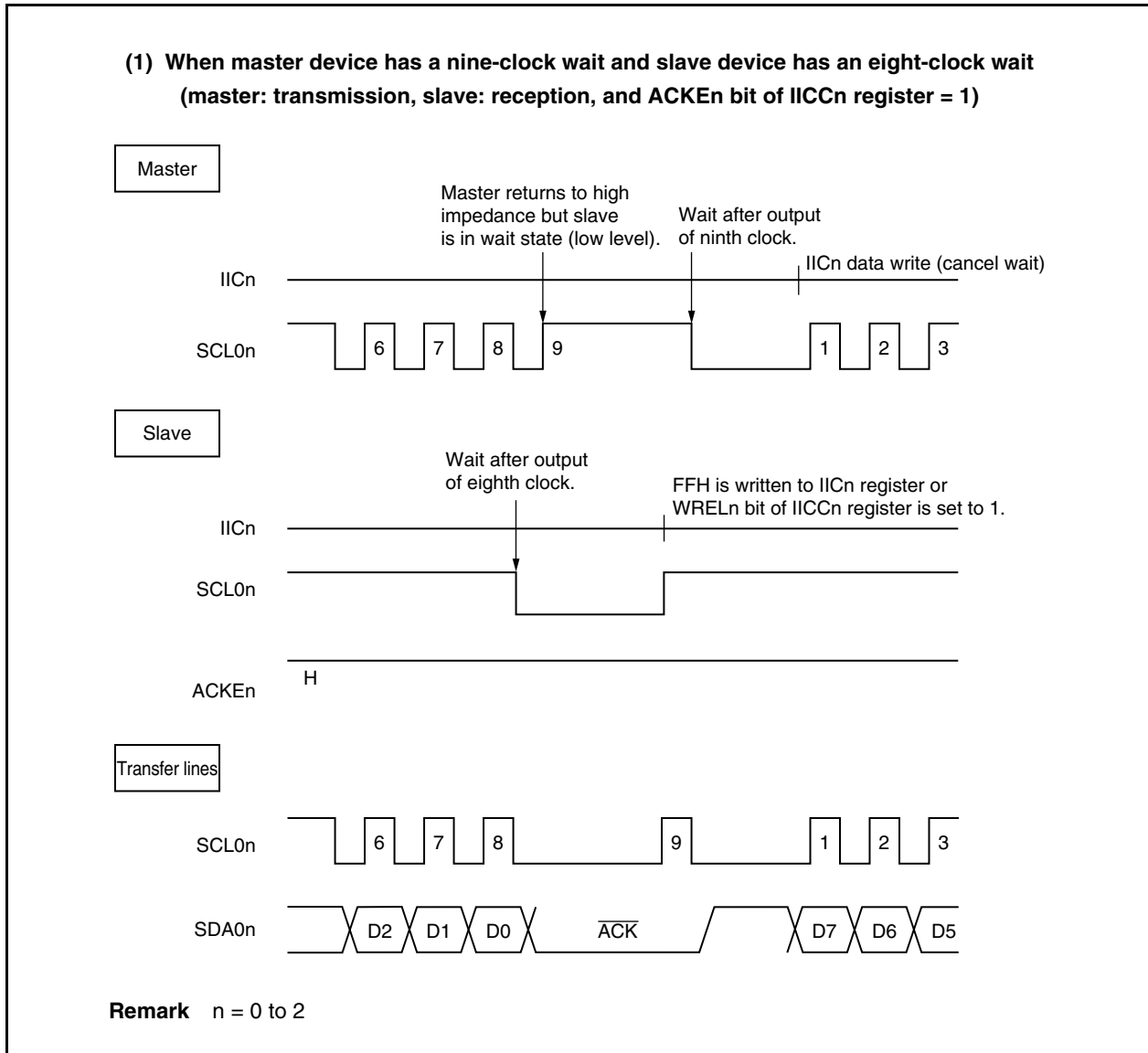
Figure 17-13. Wait Signal (1/2)
