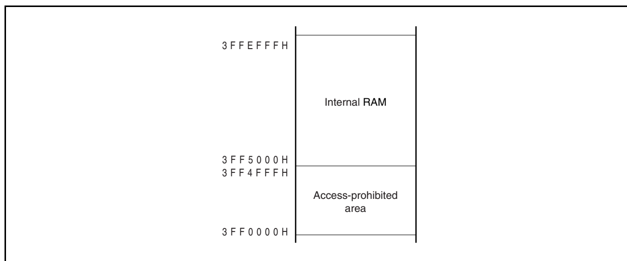
Figure 3-11. Internal RAM Area (40 KB)
