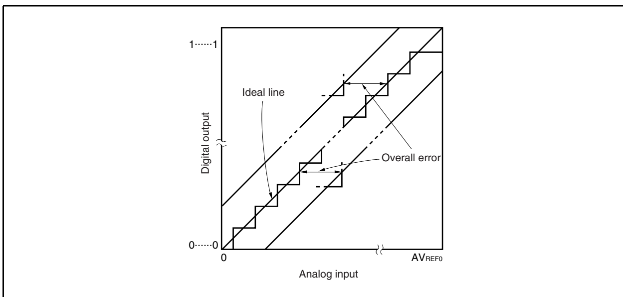
Figure 13-15. Overall Error
