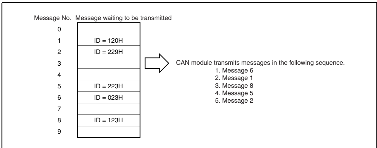
Figure 19-36. Message Processing Example (When PBB Bit = 0)
