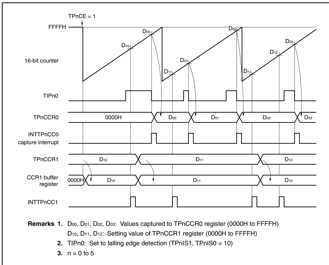
Figure 7-20. Basic Operation Timing in Free-Running Mode (TPnCCS1 = 0, TPnCCS0 = 1)
