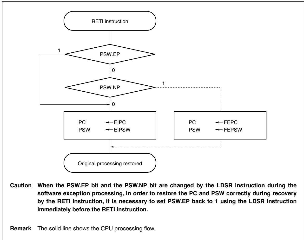
Figure 22-9. RETI Instruction Processing
