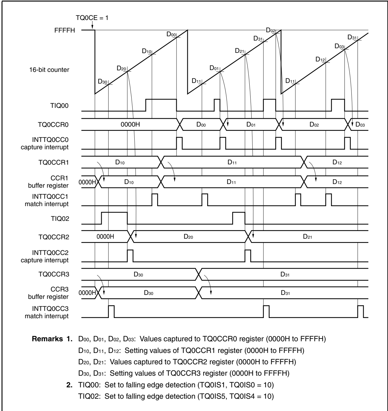
Figure 8-20. Basic Operation Timing in Free-Running Mode (TQ0CCS3 = 1, TQ0CCS2 = 0, TQ0CCS1 = 0, TQ0CCS0 = 1)
