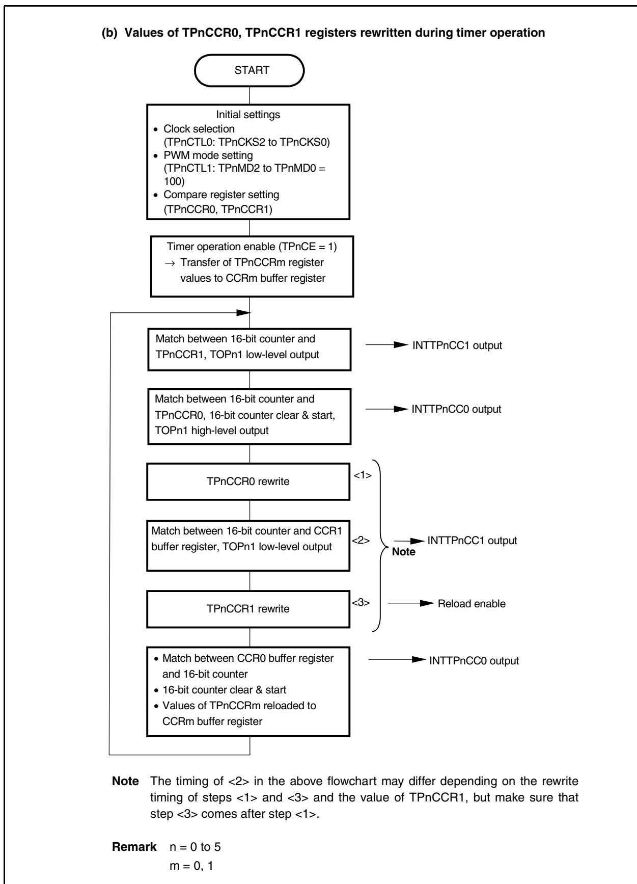
Figure 7-14. Flowchart of Basic Operation in PWM Mode (2/2)
