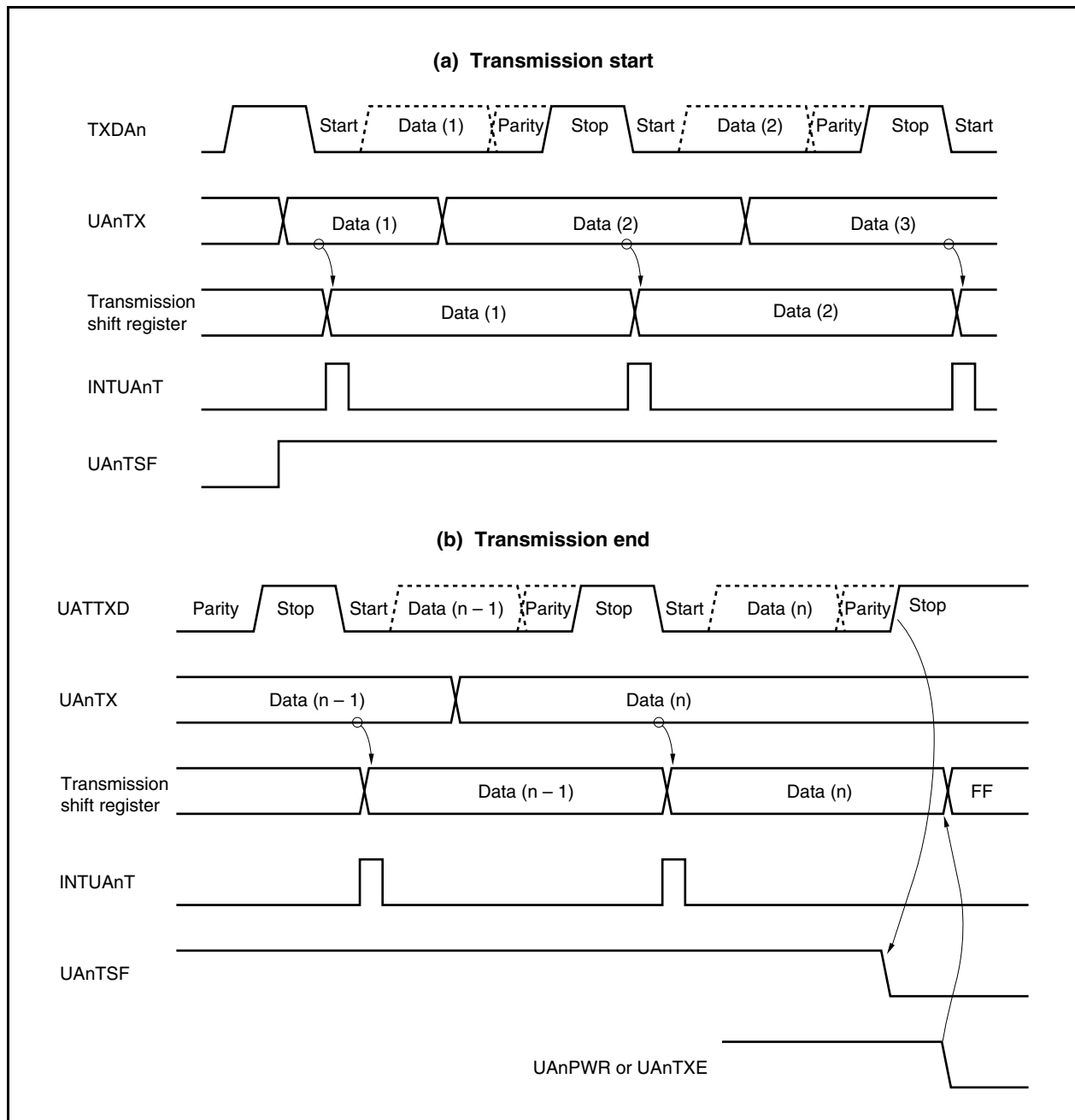
Figure 15-12. Continuous Transfer Operation Timing
