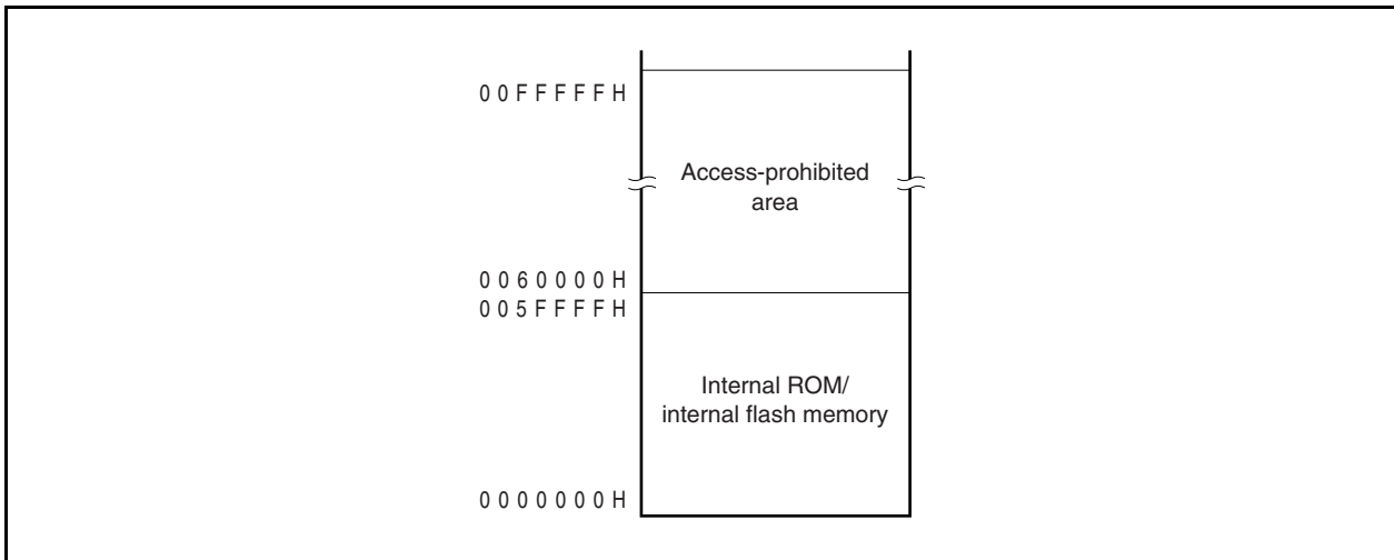
Figure 3-6. Internal ROM/Internal Flash Memory Area (384 KB)
