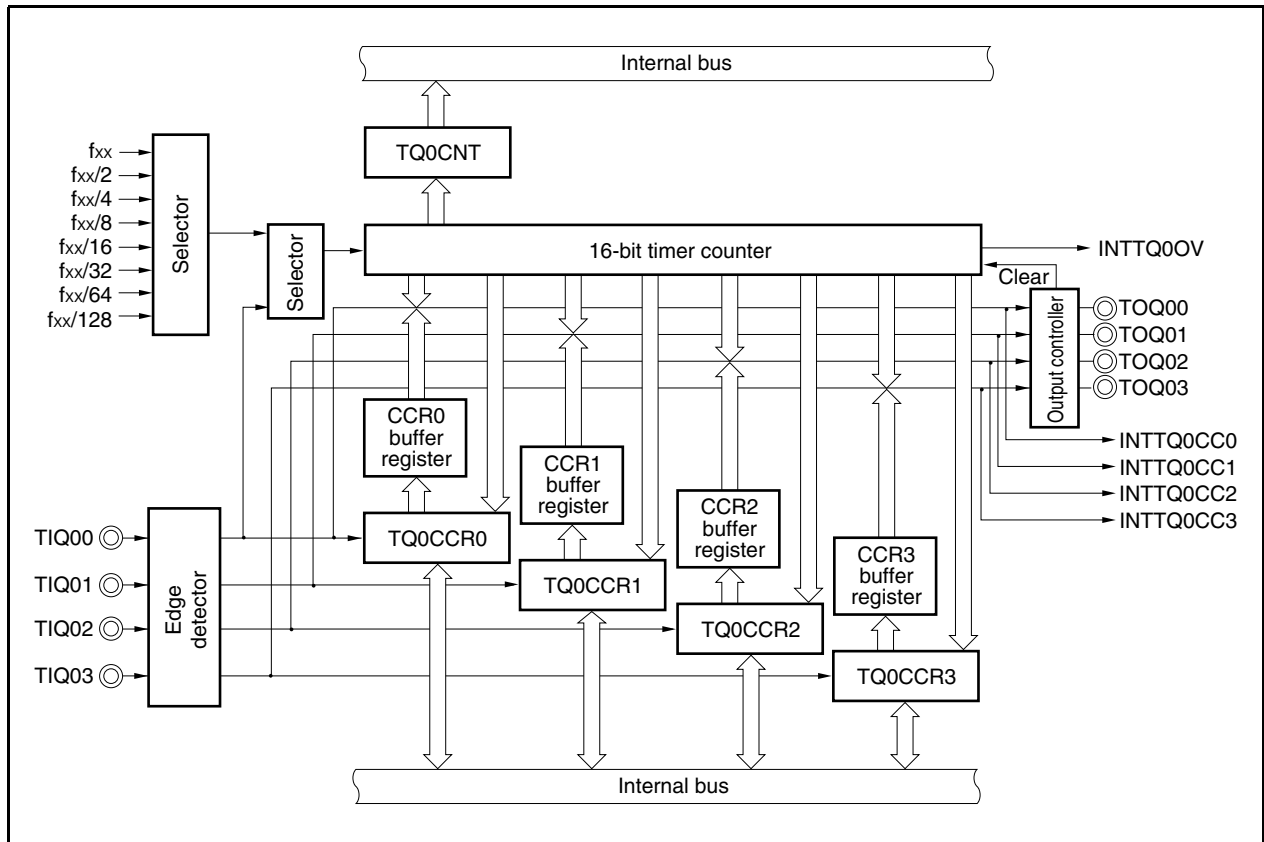
Figure 8-1. Timer Q Block Diagram
