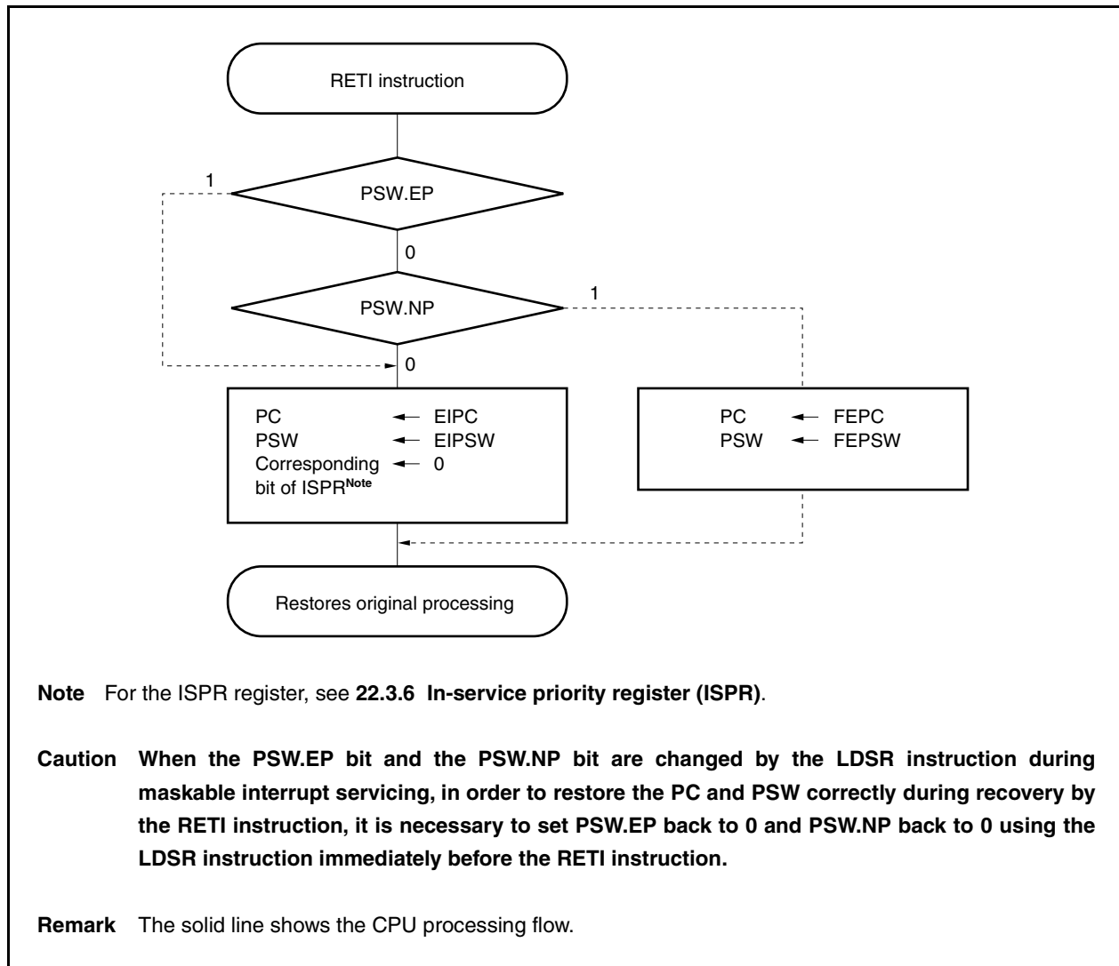
Figure 22-5. RETI Instruction Processing
