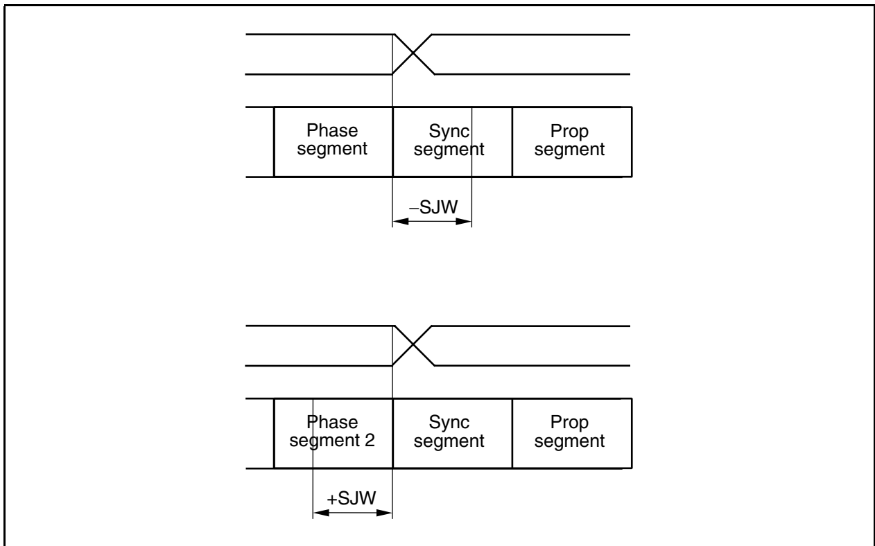
Figure 19-19. Bit Synchronization
