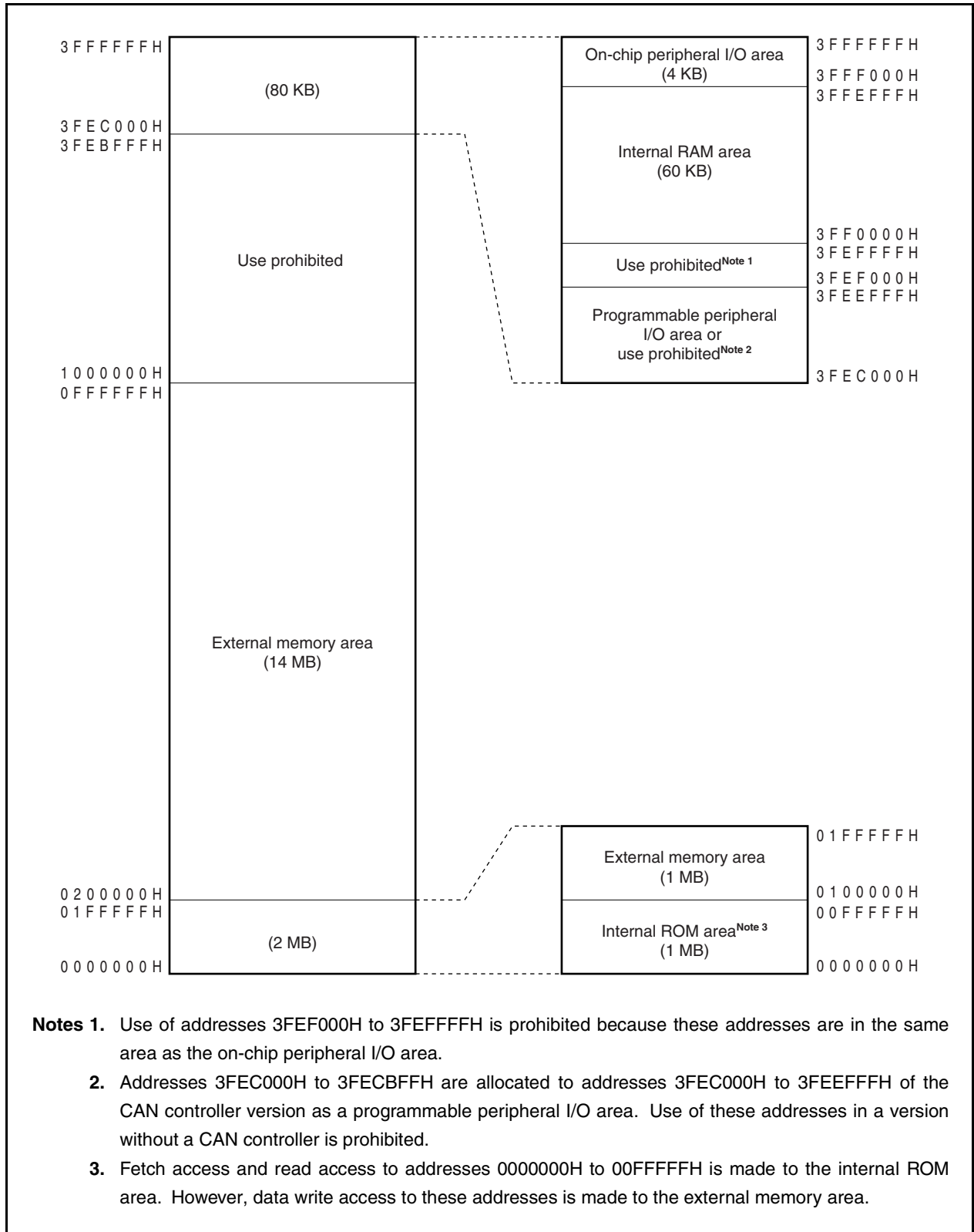
Figure 3-3. Data Memory Map (Physical Addresses)
