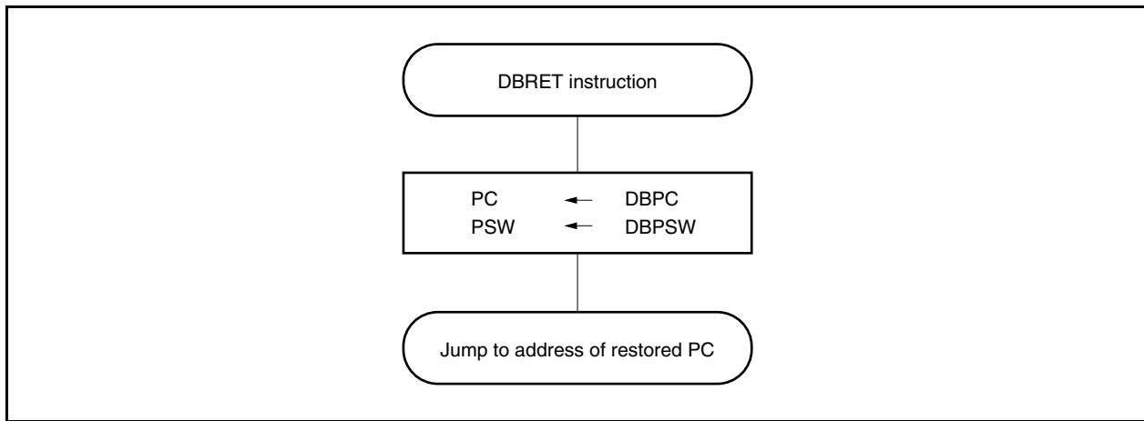
Figure 22-13. Processing Format of Restoration from Debug Trap
