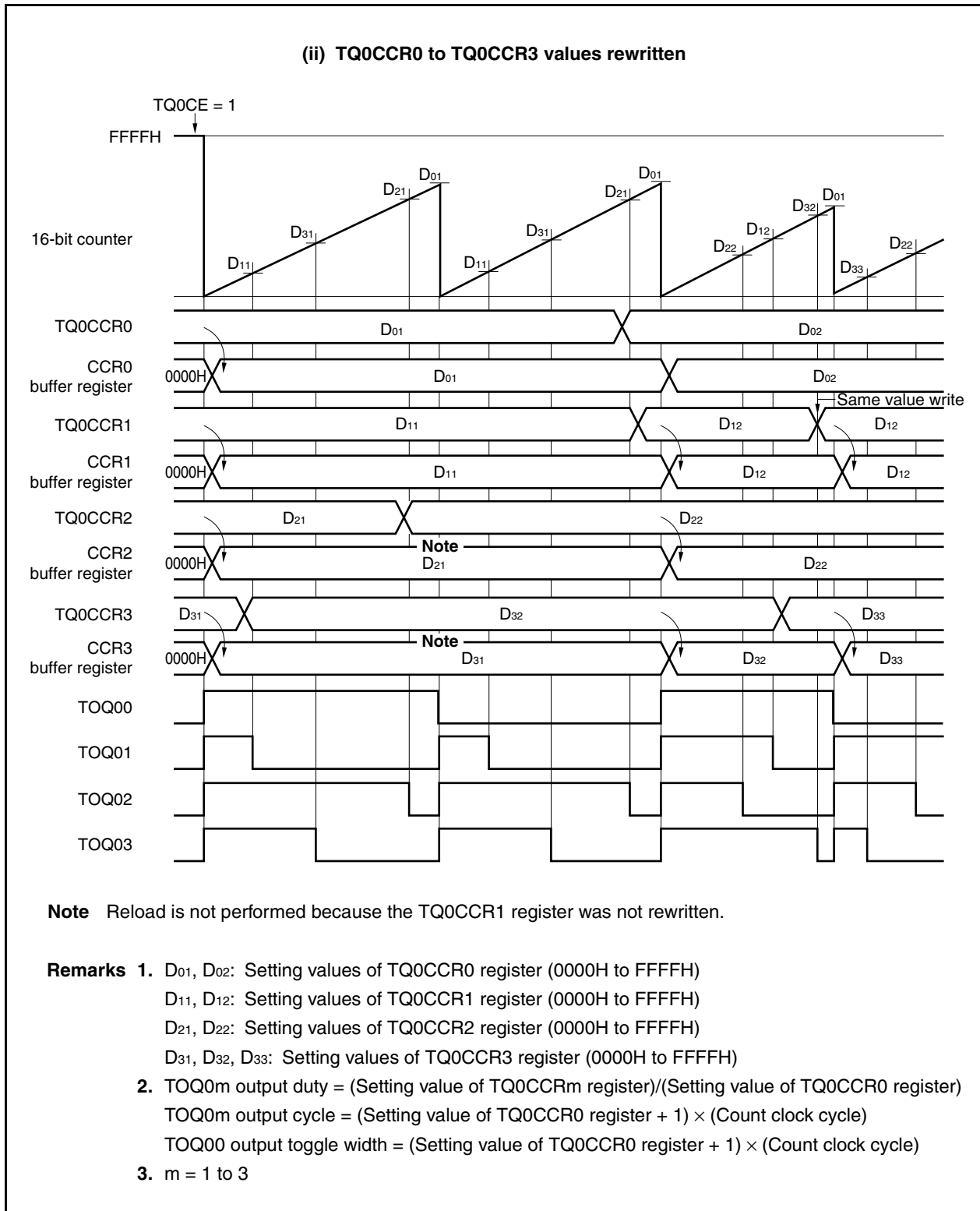
Figure 8-15. Basic Operation Timing in PWM Mode (2/2)
