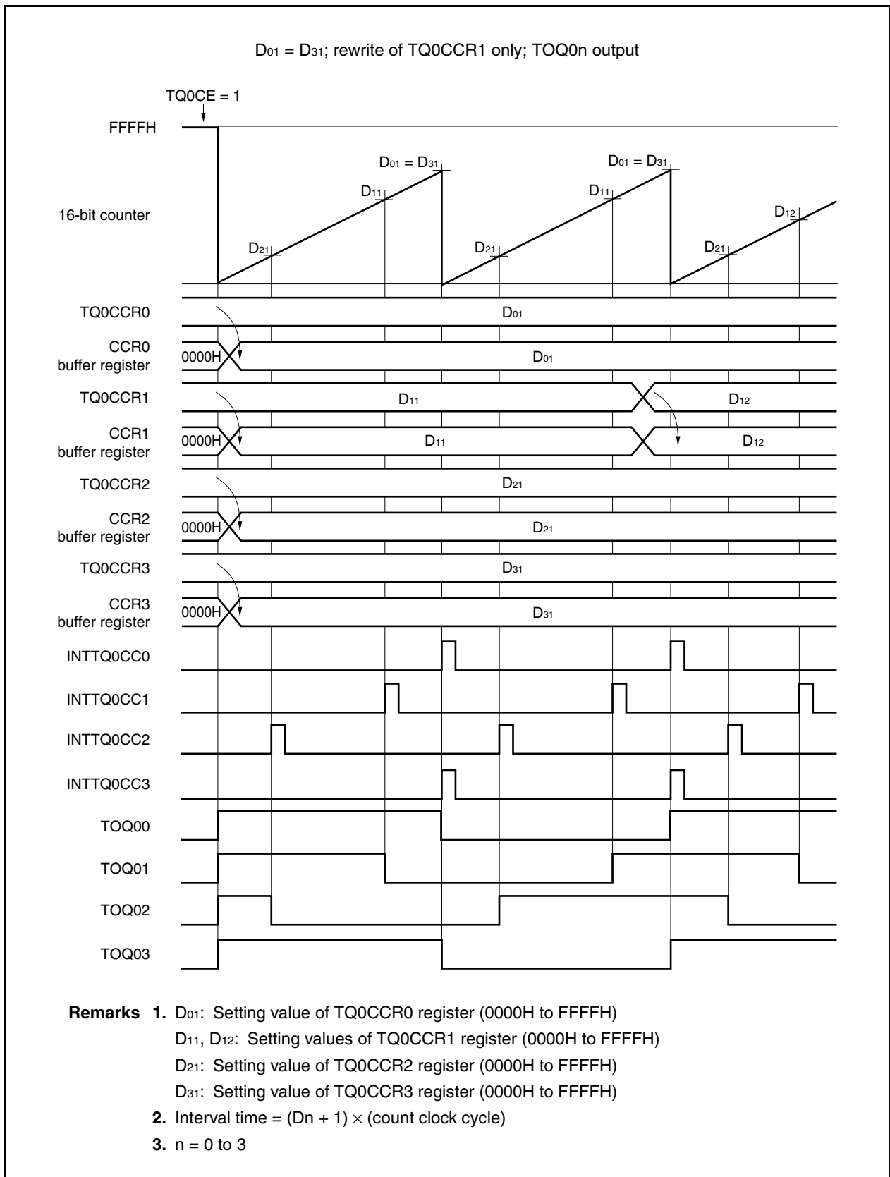
Figure 8-7. Basic Operation Timing in Interval Timer Mode (2/2)
