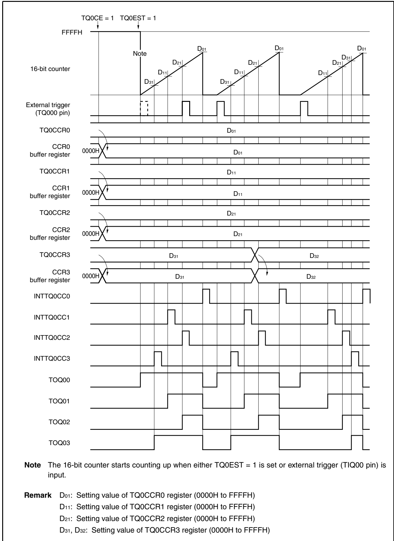
Figure 8-13. Timing of Basic Operation in One-Shot Pulse Mode
