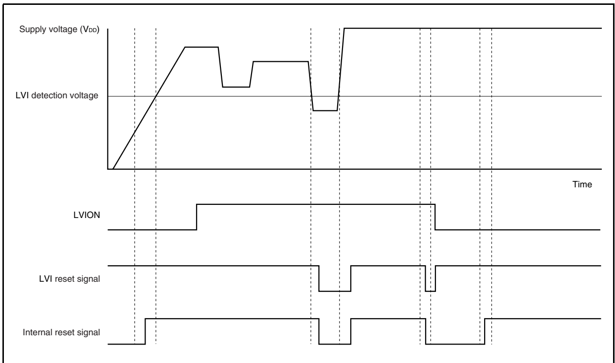
Figure 25-4. Timing of Reset Operation by Low-Voltage Detector
