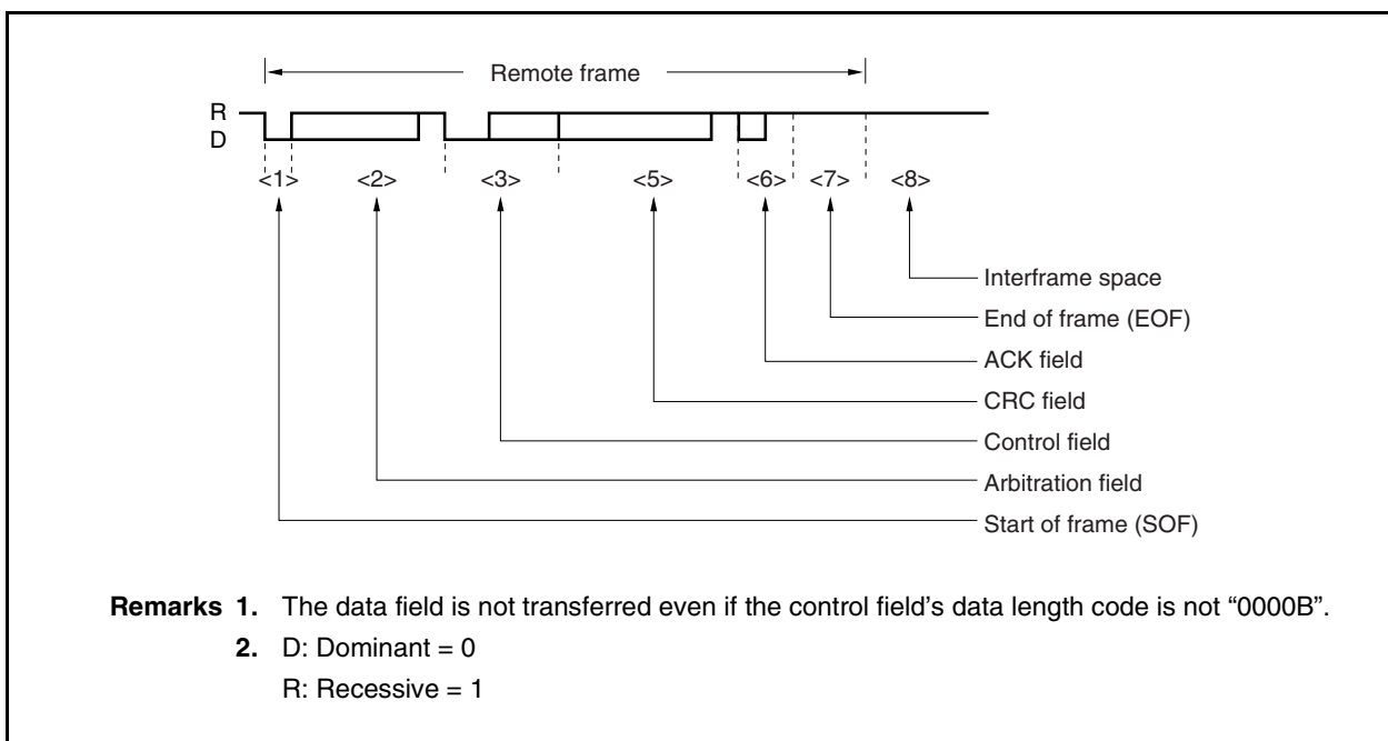
Figure 19-4. Remote Frame
