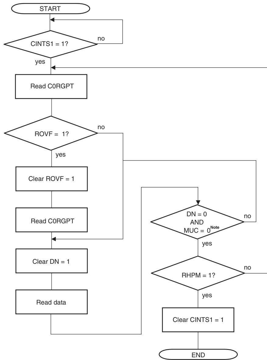
Figure 19-57. Receive Software Polling
