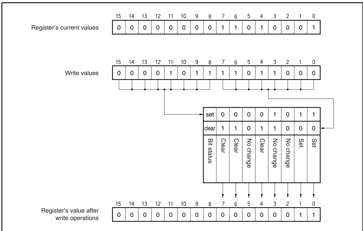
Figure 19-30. Example of Bit Setting/Clearing Operations
