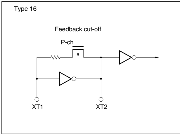
Figure 2-1. Pin I/O Circuits (2/2)
