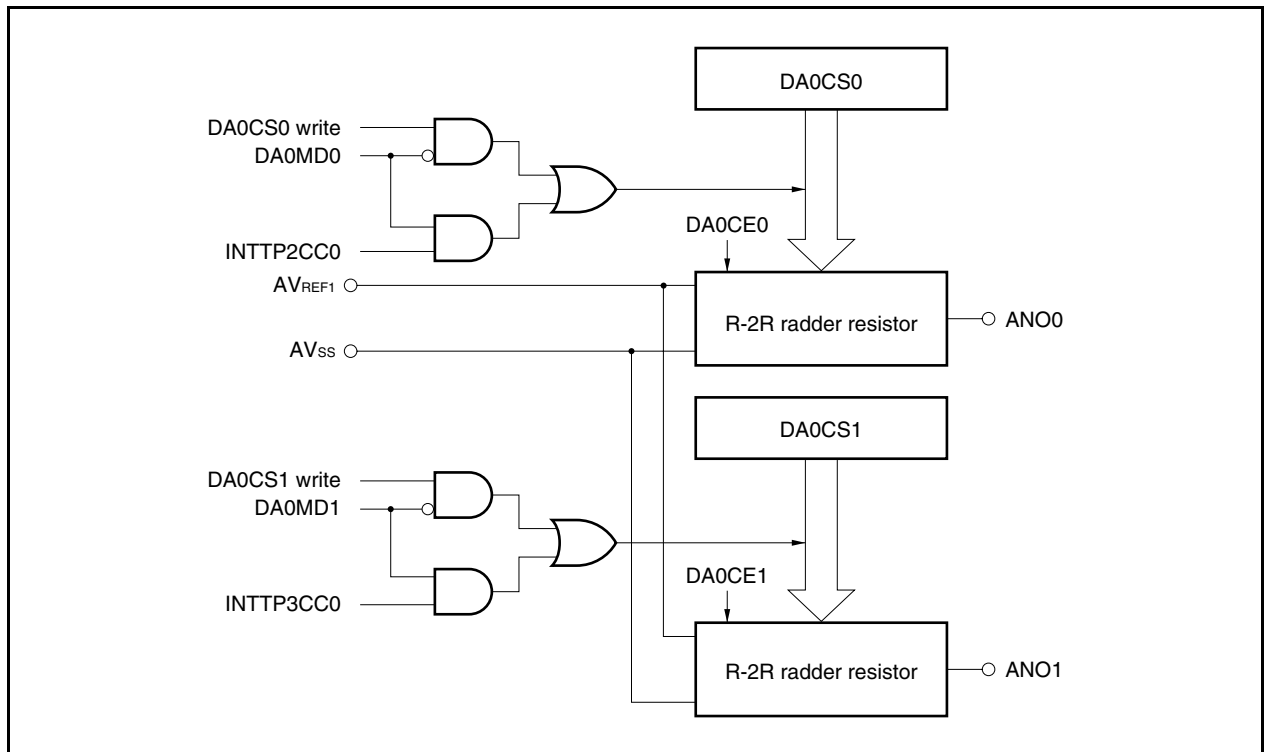
Figure 14-1. Block Diagram of D/A Converter
