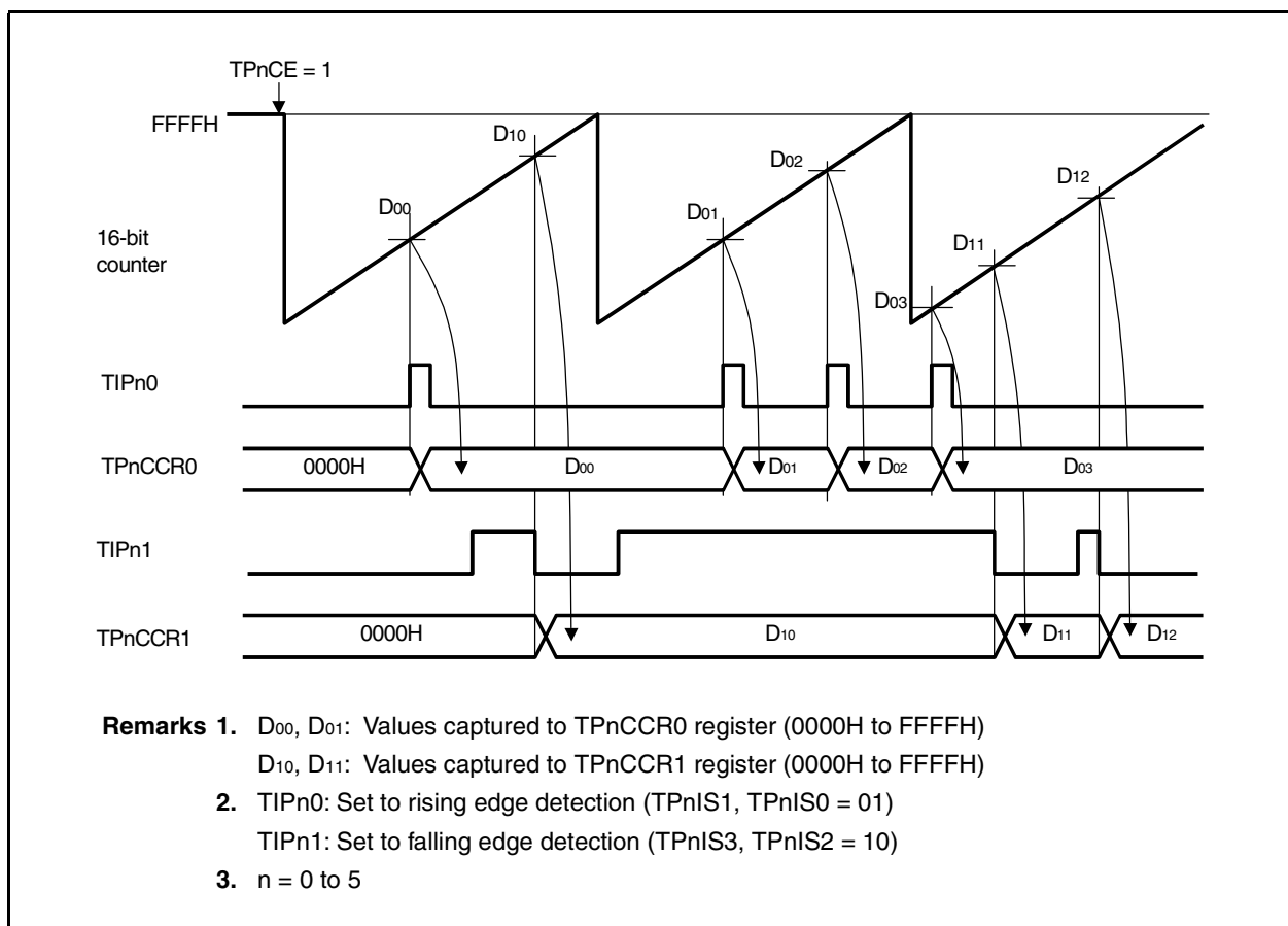
Figure 7-18. Basic Operation Timing in Free-Running Mode (TPnCCS1 = 1, TPnCCS0 = 1)
