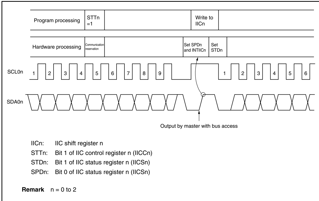
Figure 17-15. Communication Reservation Timing
