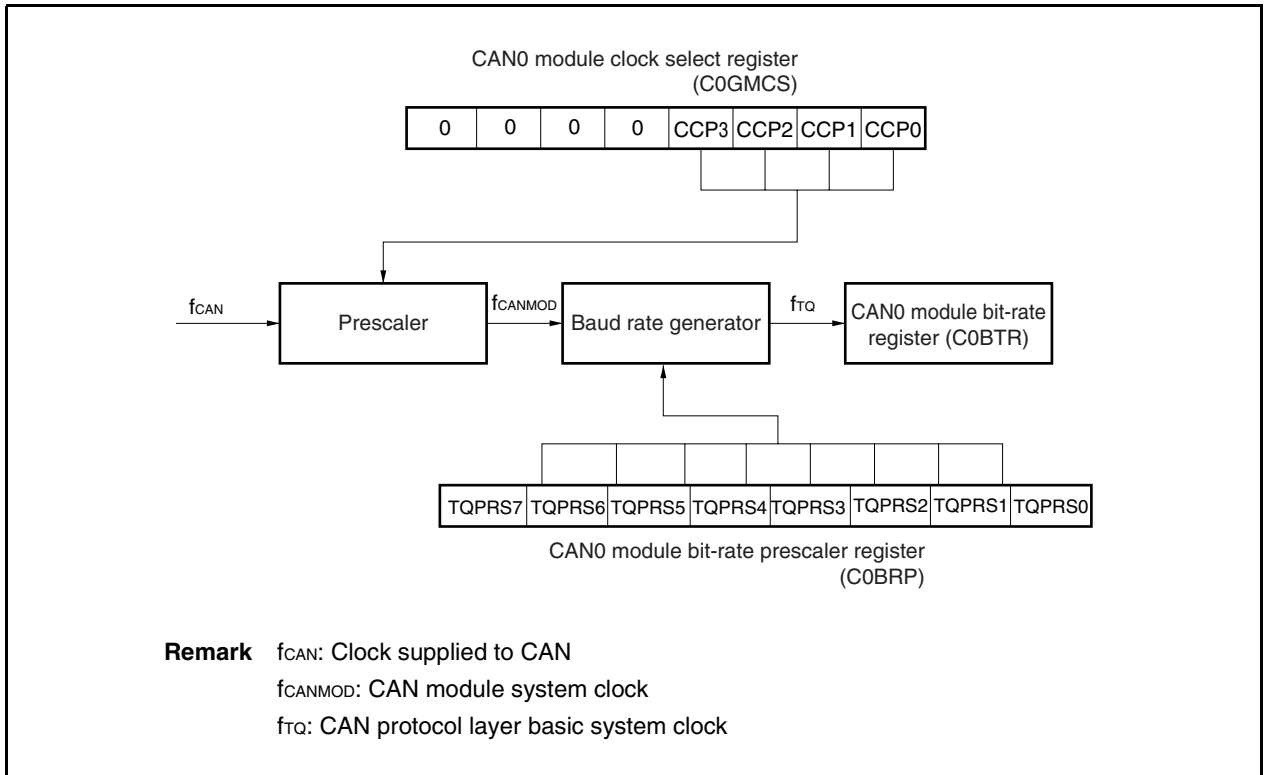
Figure 19-28. CAN Controller Clocks
