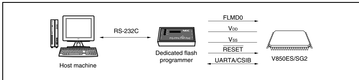
Figure 28-1. Environment Required for Writing Programs to Flash Memory
