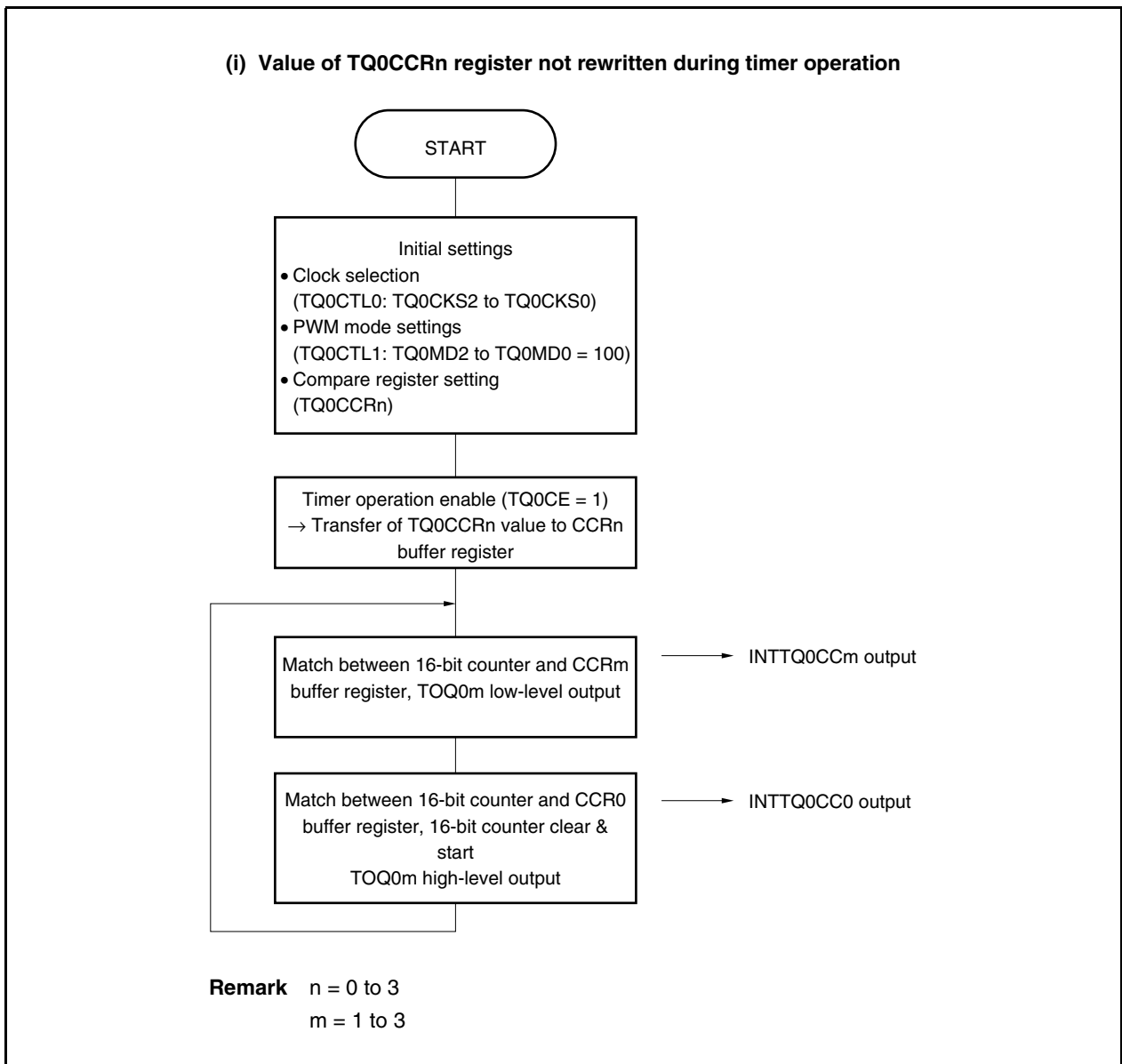
Figure 8-14. Flowchart of Basic Operation in PWM Mode (1/2)
