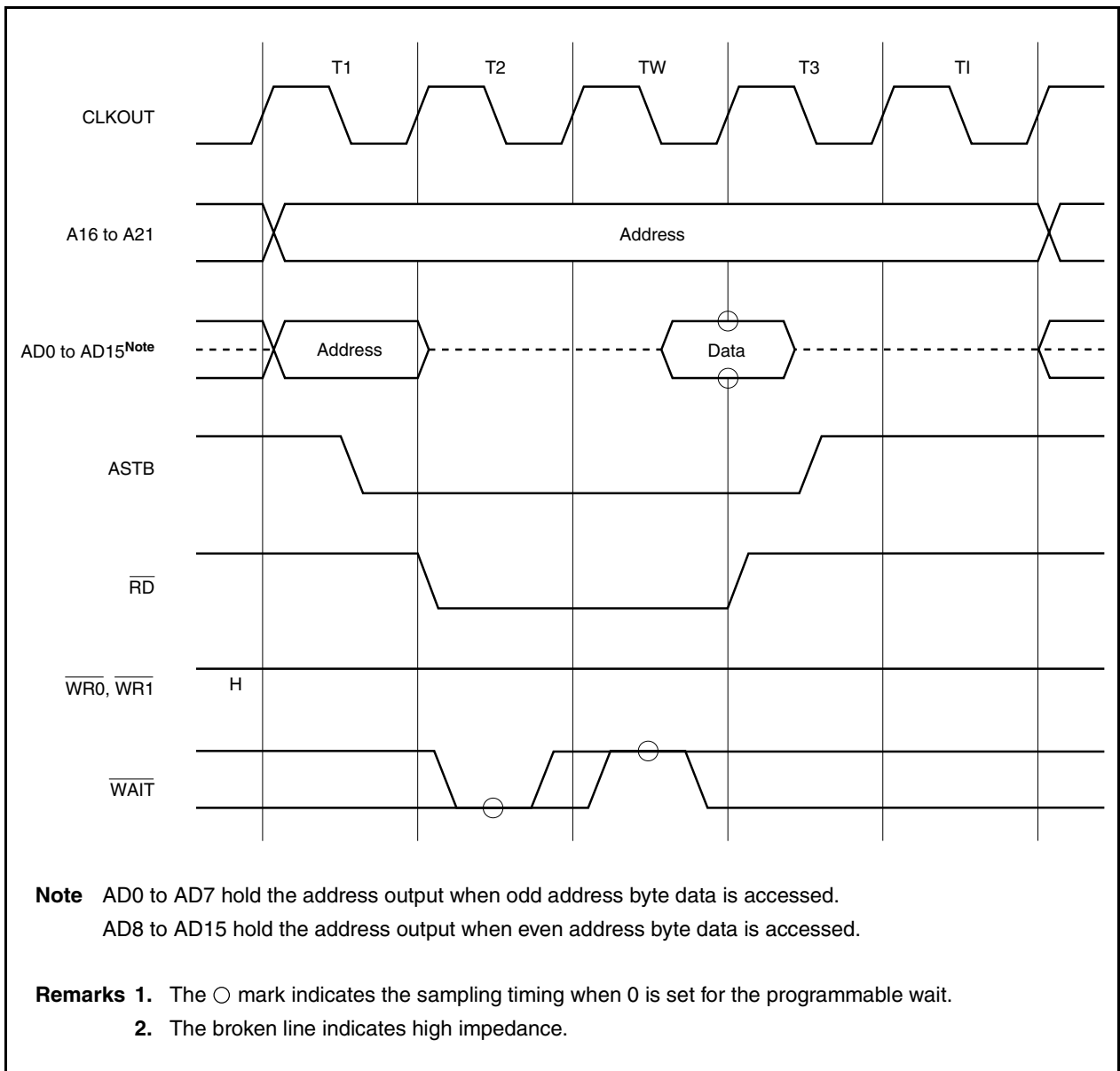
Figure 5-7. When Wait State (1 Wait) and Idle State Are Inserted
