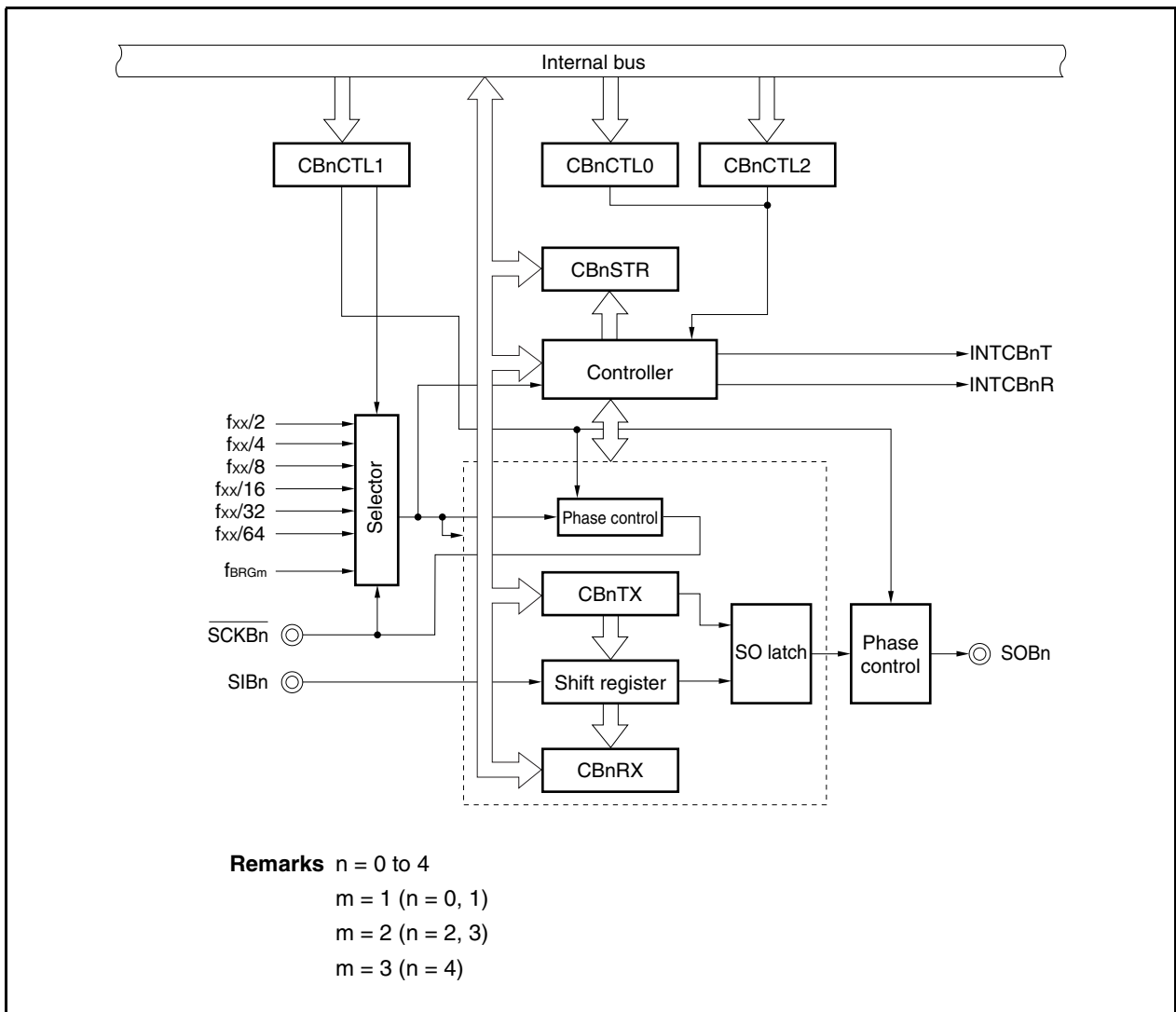
Figure 16-3. Block Diagram of CSIB
