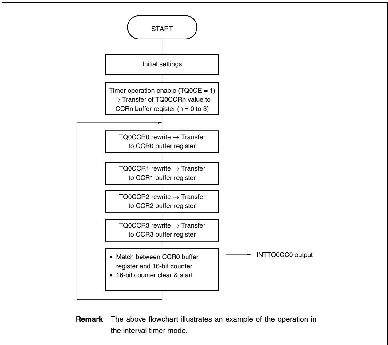
Figure 8-2. Flowchart of Basic Operation for Anytime Write
