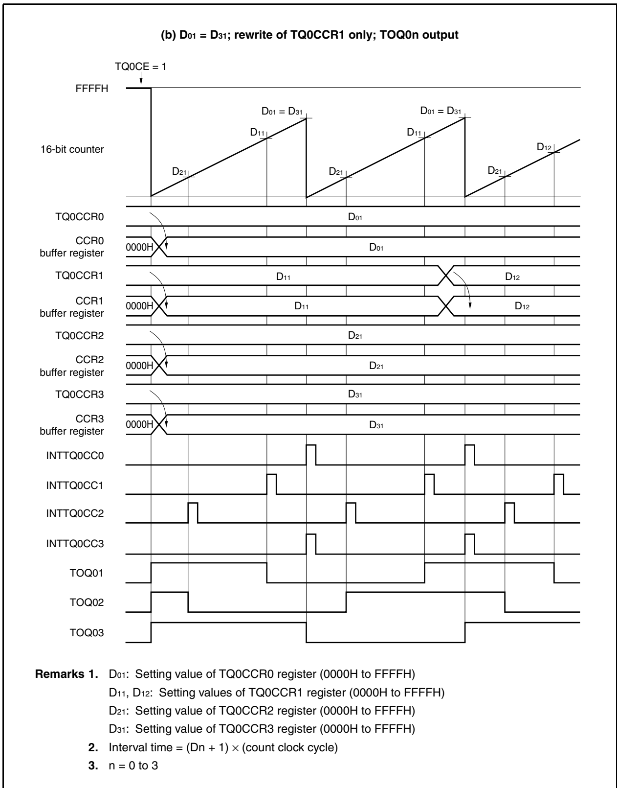
Figure 8-9. Basic Operation Timing in External Event Count Mode (2/2)
