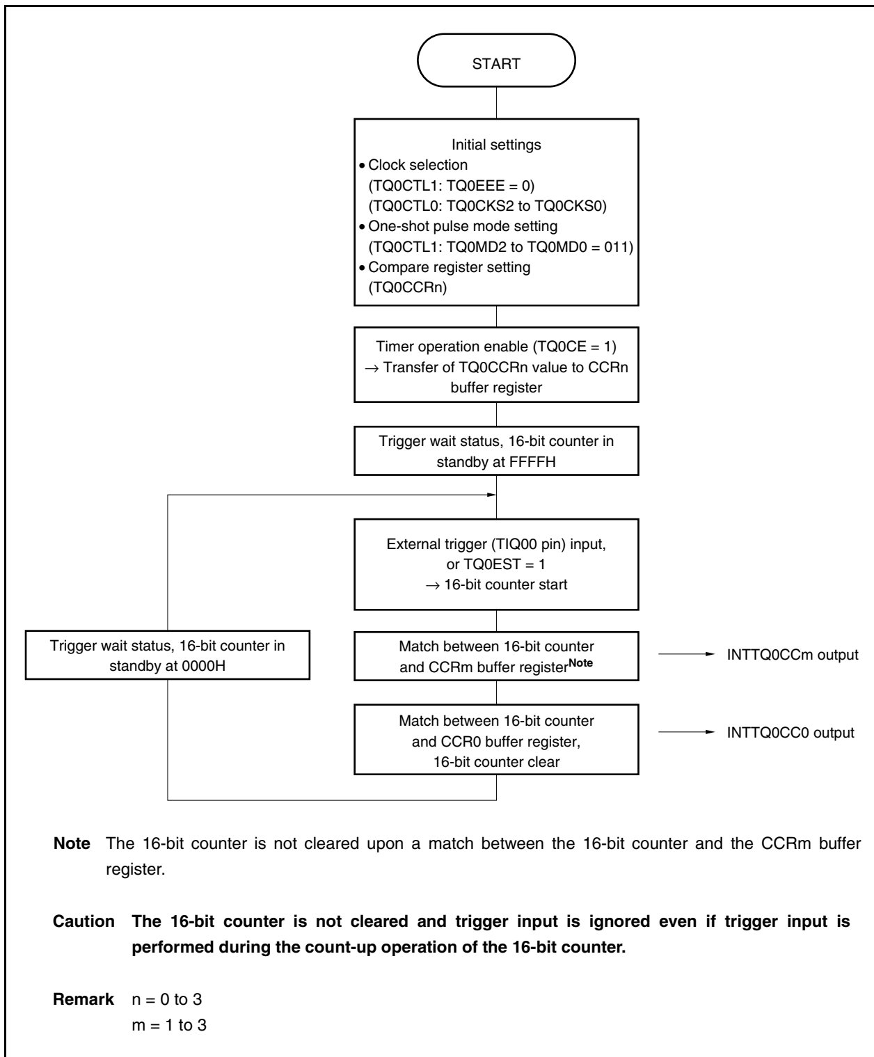
Figure 8-12. Flowchart of Basic Operation in One-Shot Pulse Mode
