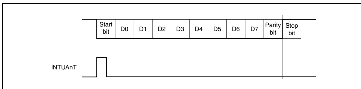
Figure 15-10. UART Transmission
