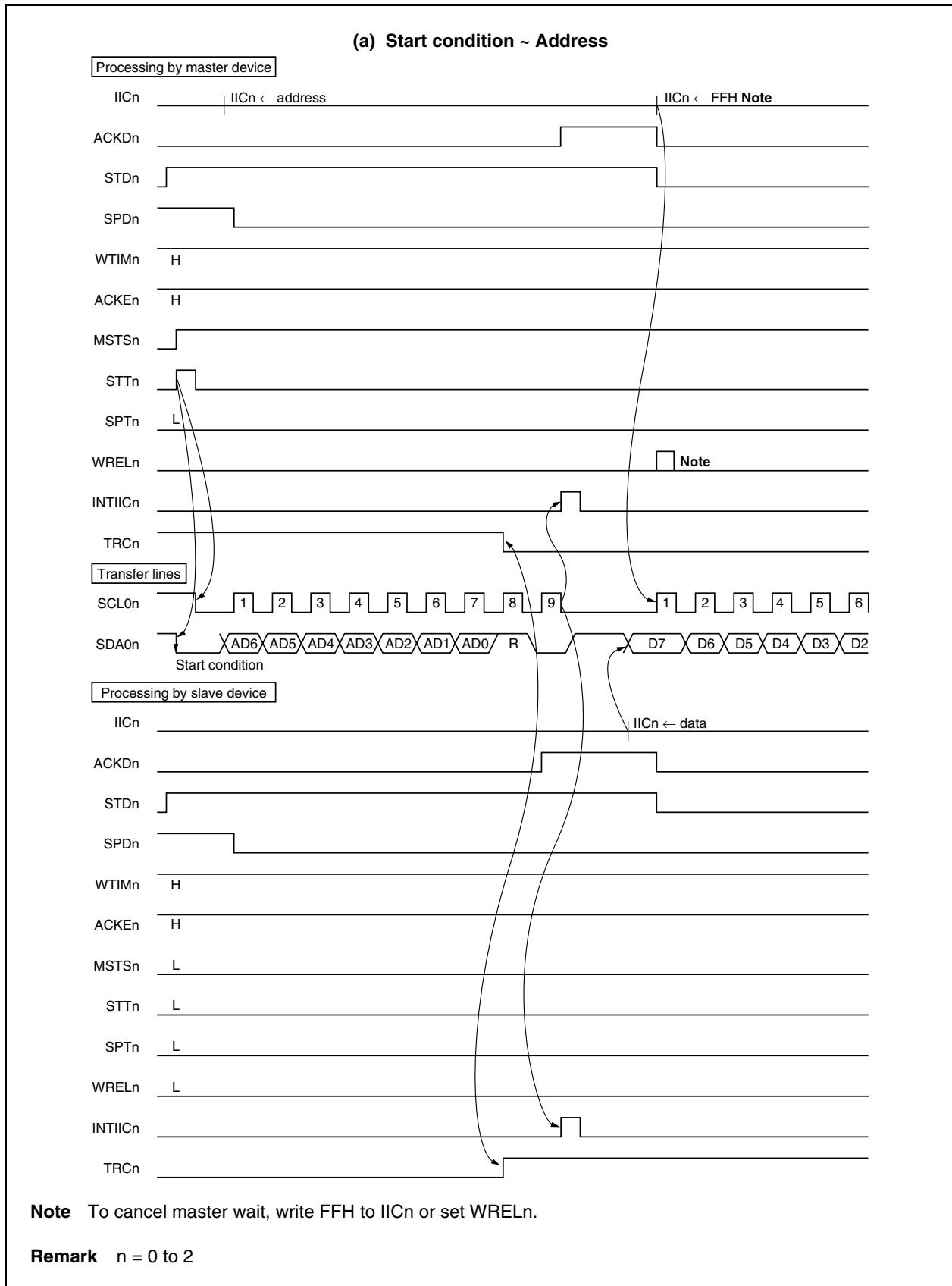
Figure 17-22. Example of Slave to Master Communication (When 9-Clock Wait Is Selected for Both Master and Slave) (1/3)
