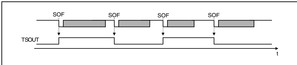
Figure 19-42. Timing Diagram of Capture Output Signal TSOUT
