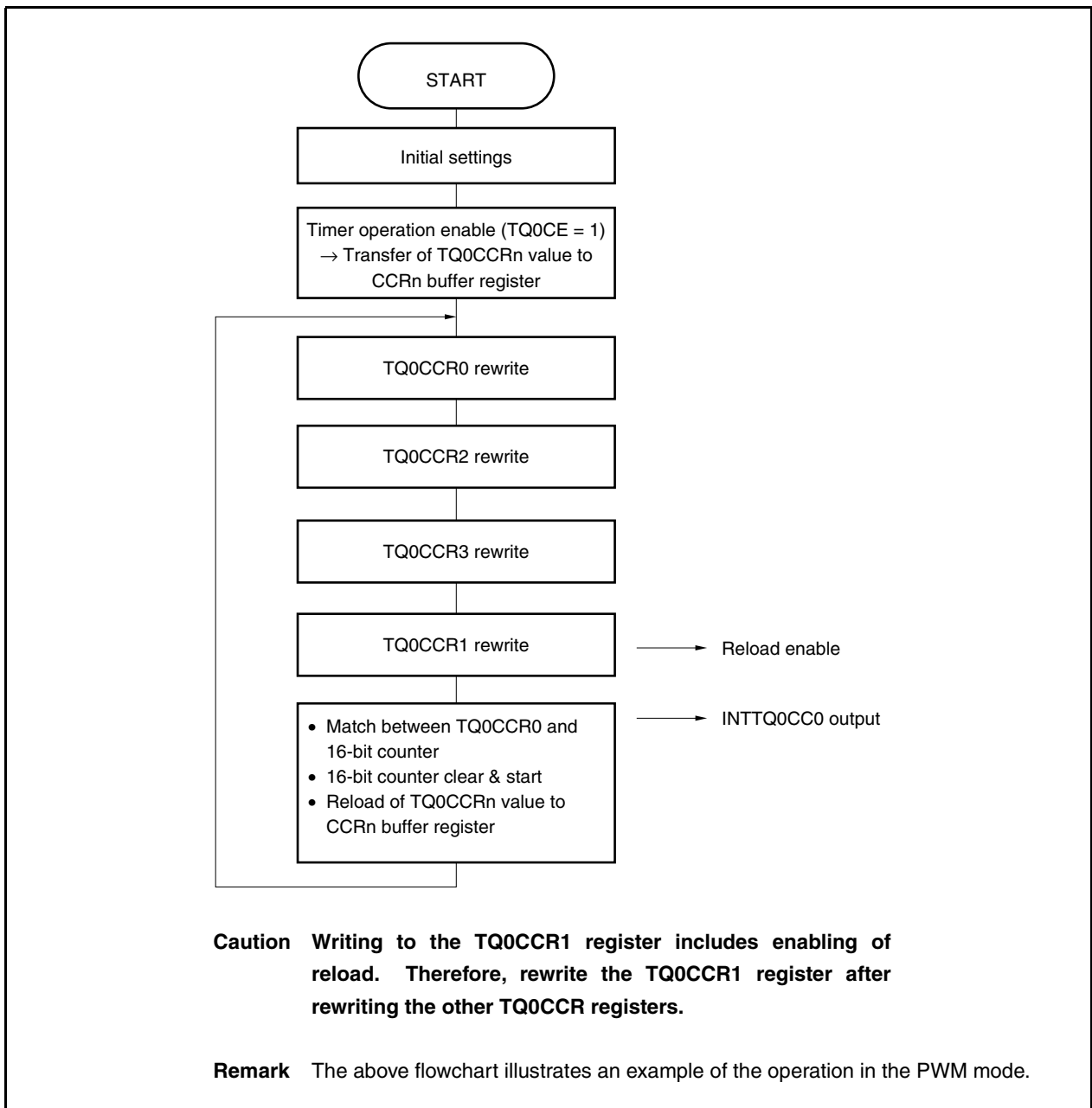
Figure 8-4. Flowchart of Basic Operation for Reload
