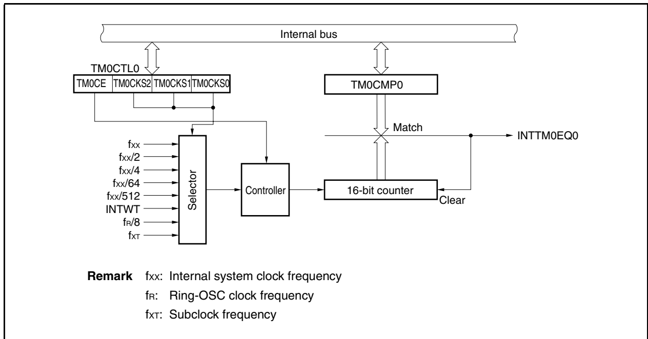
Figure 9-1. Block Diagram of TMM
