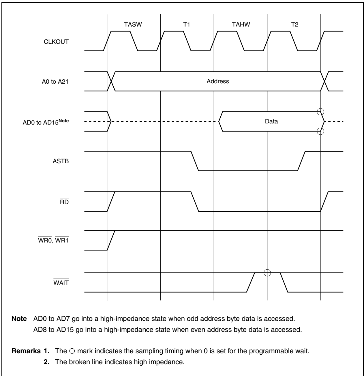
Figure 5-17. When Address Wait State Is Inserted
