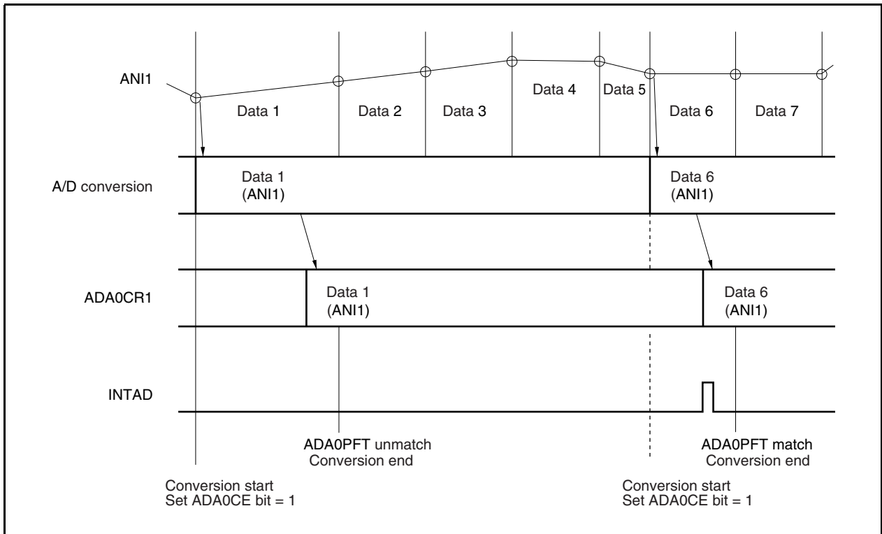
Figure 13-10. Timing Example of One-Shot Select Mode Operation (When Power-Fail Compare Is Made: ADA0S Register = 01H)
