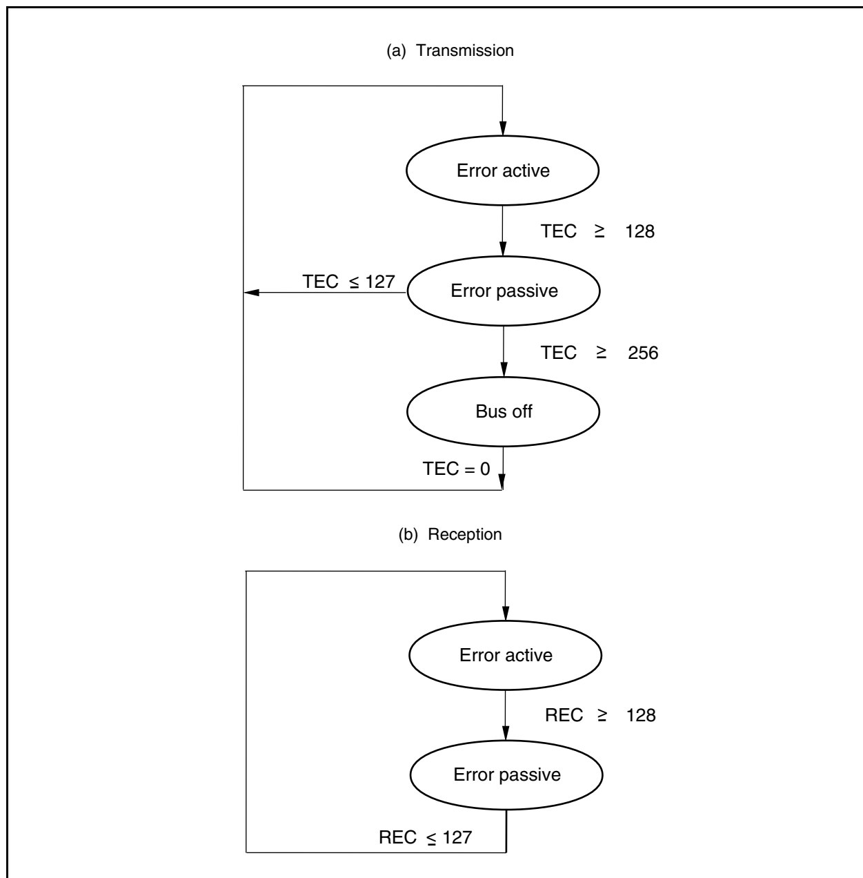
Figure 19-22. Error State Transition Chart
