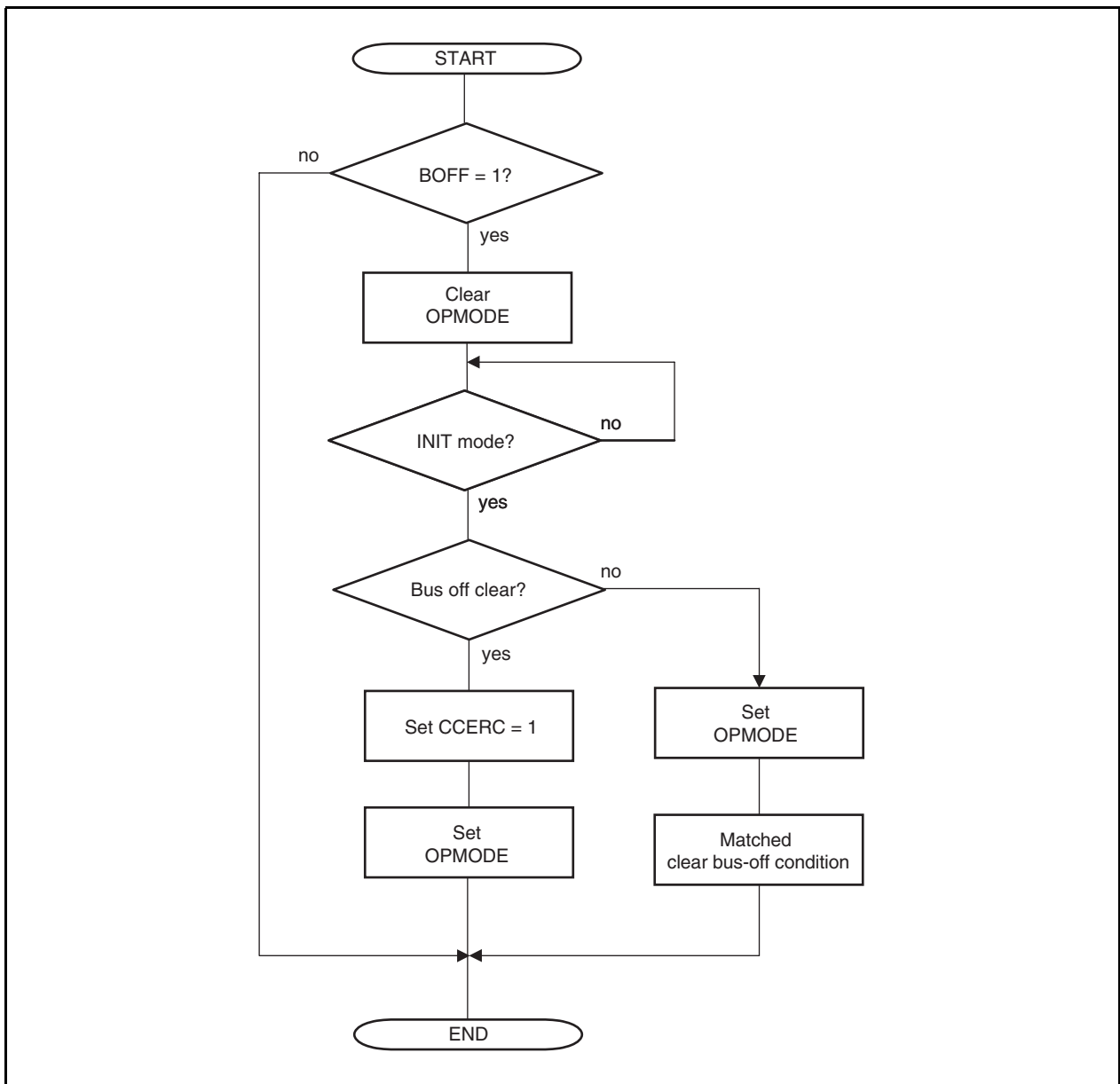
Figure 19-60. Bus-Off Recovery
