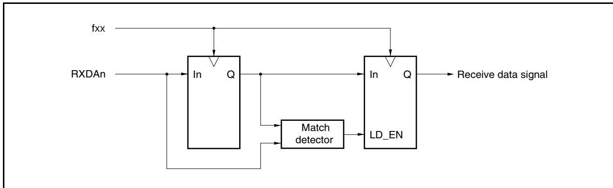
Figure 15-14. Noise Filter Circuit
