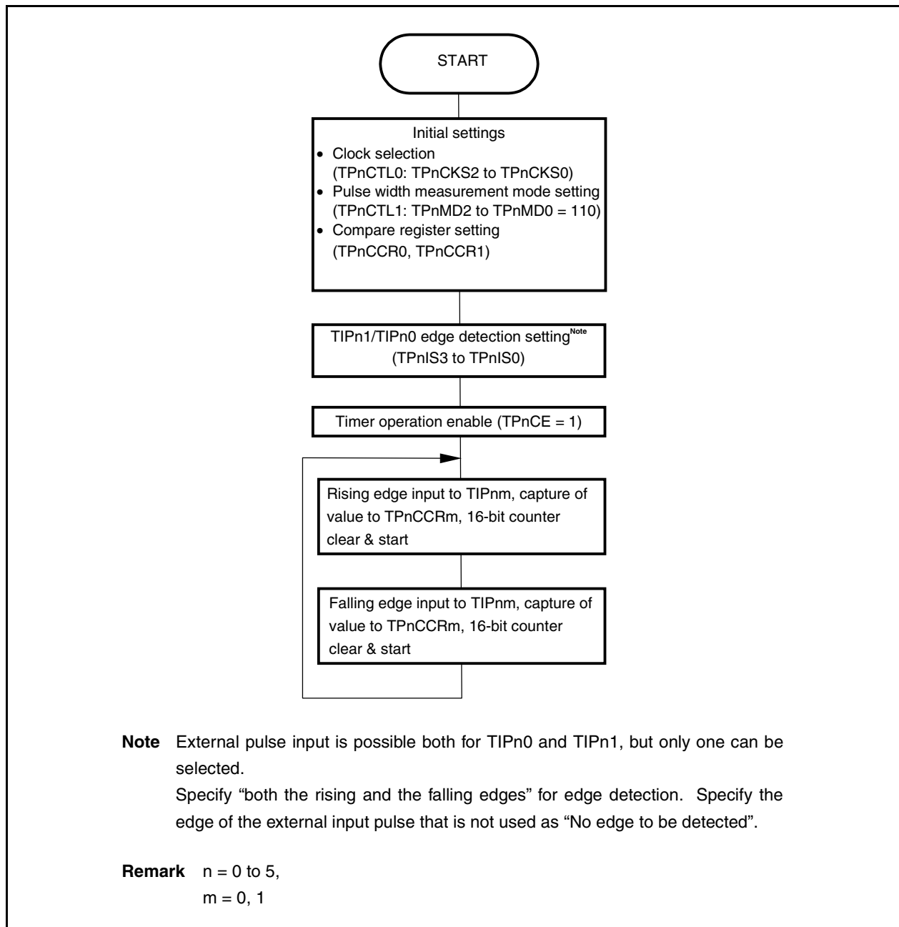
Figure 7-21. Flowchart of Basic Operation in Pulse Width Measurement Mode
