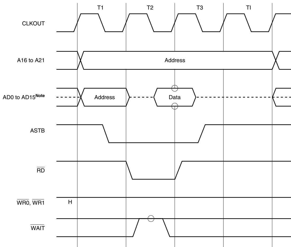
Figure 5-6. When Idle State Is Inserted
