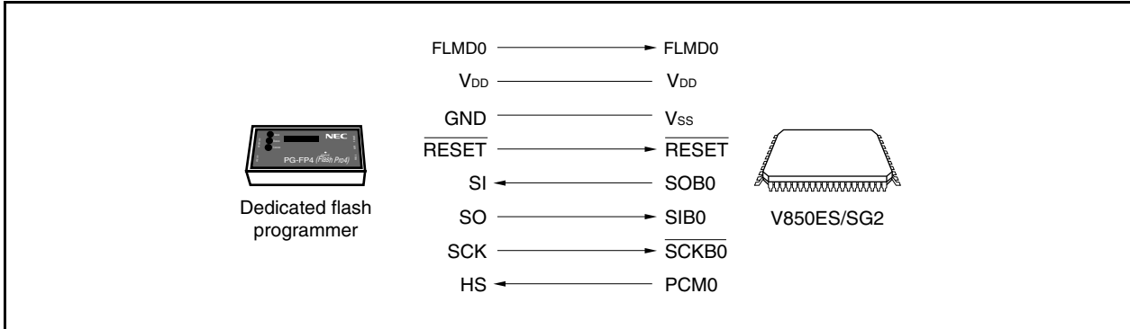
Figure 28-4. Communication with Dedicated Flash Programmer (CSIB0 + HS)
