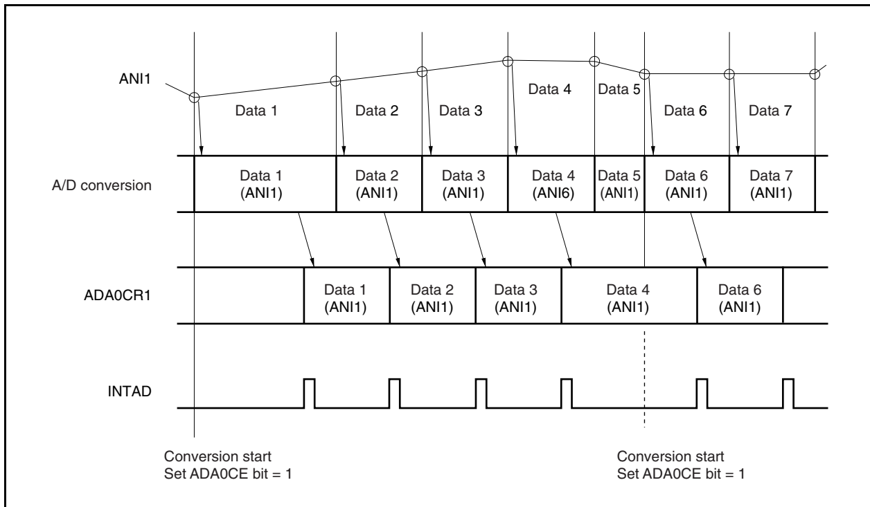
Figure 13-4. Timing Example of Continuous Select Mode Operation (ADA0S = 01H)
