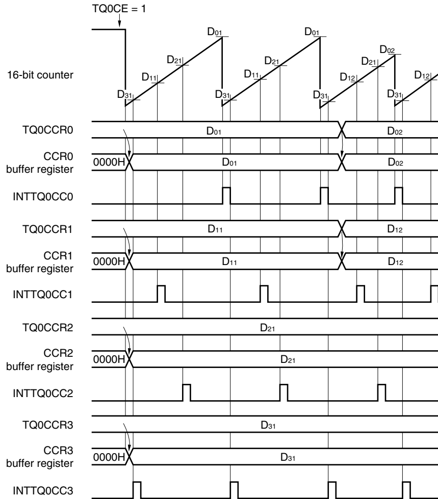
Figure 8-3. Timing Diagram for Anytime Write
