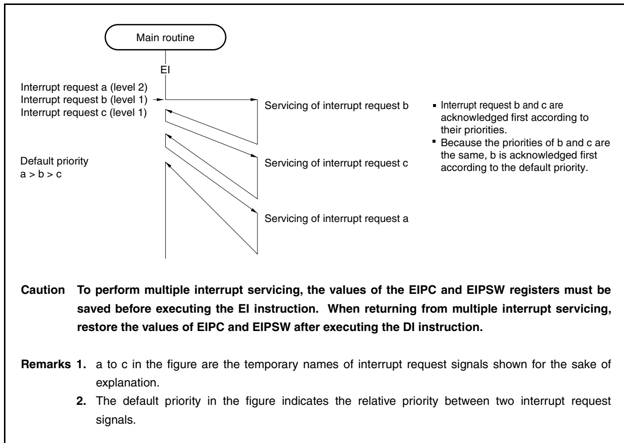
Figure 22-7. Example of Servicing Interrupt Request Signals Simultaneously Generated
