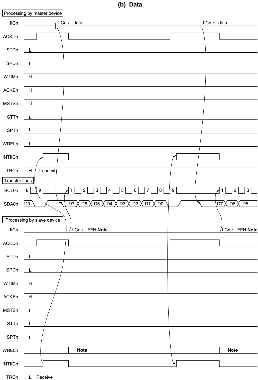
Figure 17-21. Example of Master to Slave Communication (When 9-Clock Wait Is Selected for Both Master and Slave) (2/3)
