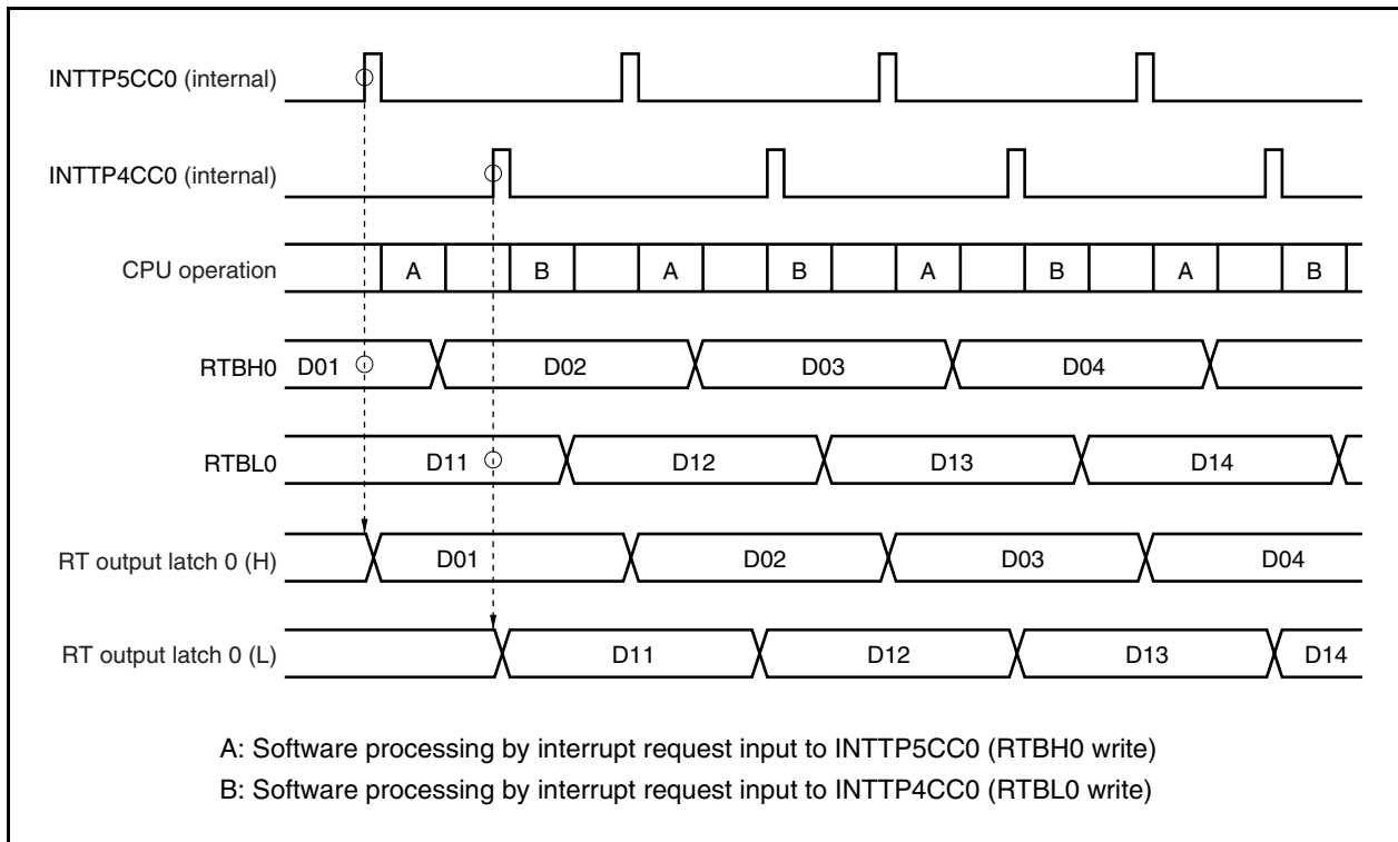
Figure 10-2. Example of Operation Timing of RTO0 (When EXTR0 Bit = 0, BYTE0 Bit = 0)
