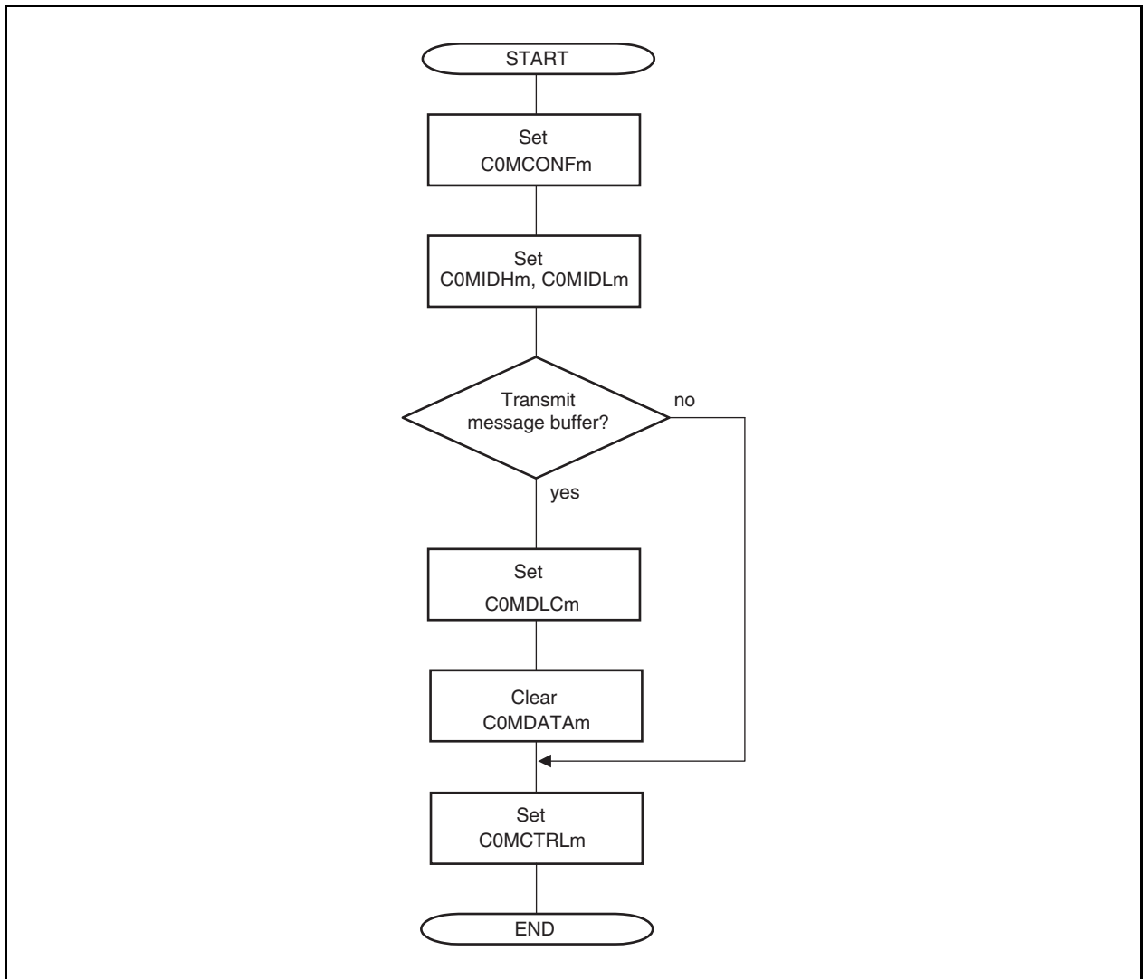
Figure 19-46. Message Buffer Initialization
