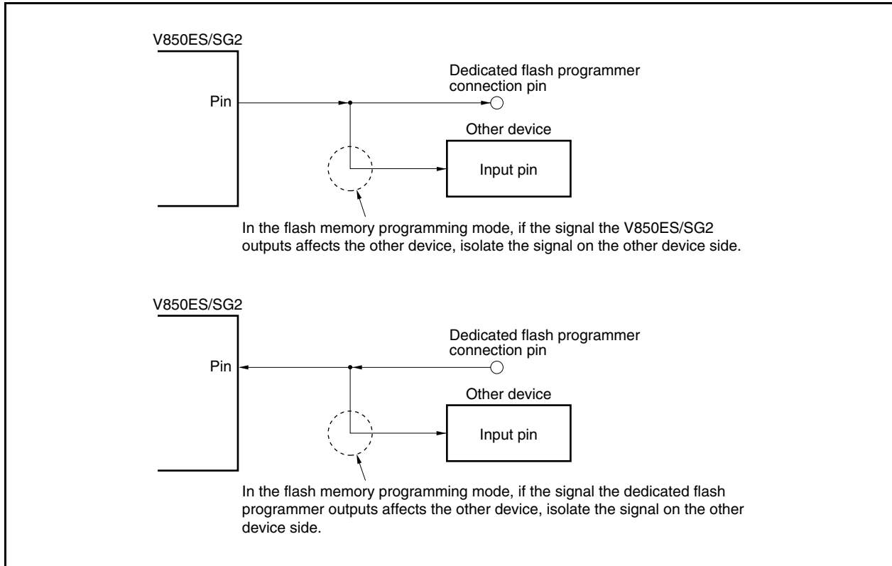
Figure 28-8. Malfunction of Other Device
