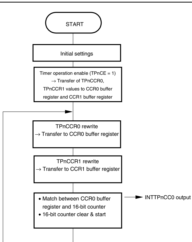
Figure 7-2. Flowchart of Basic Operation for Anytime Write
