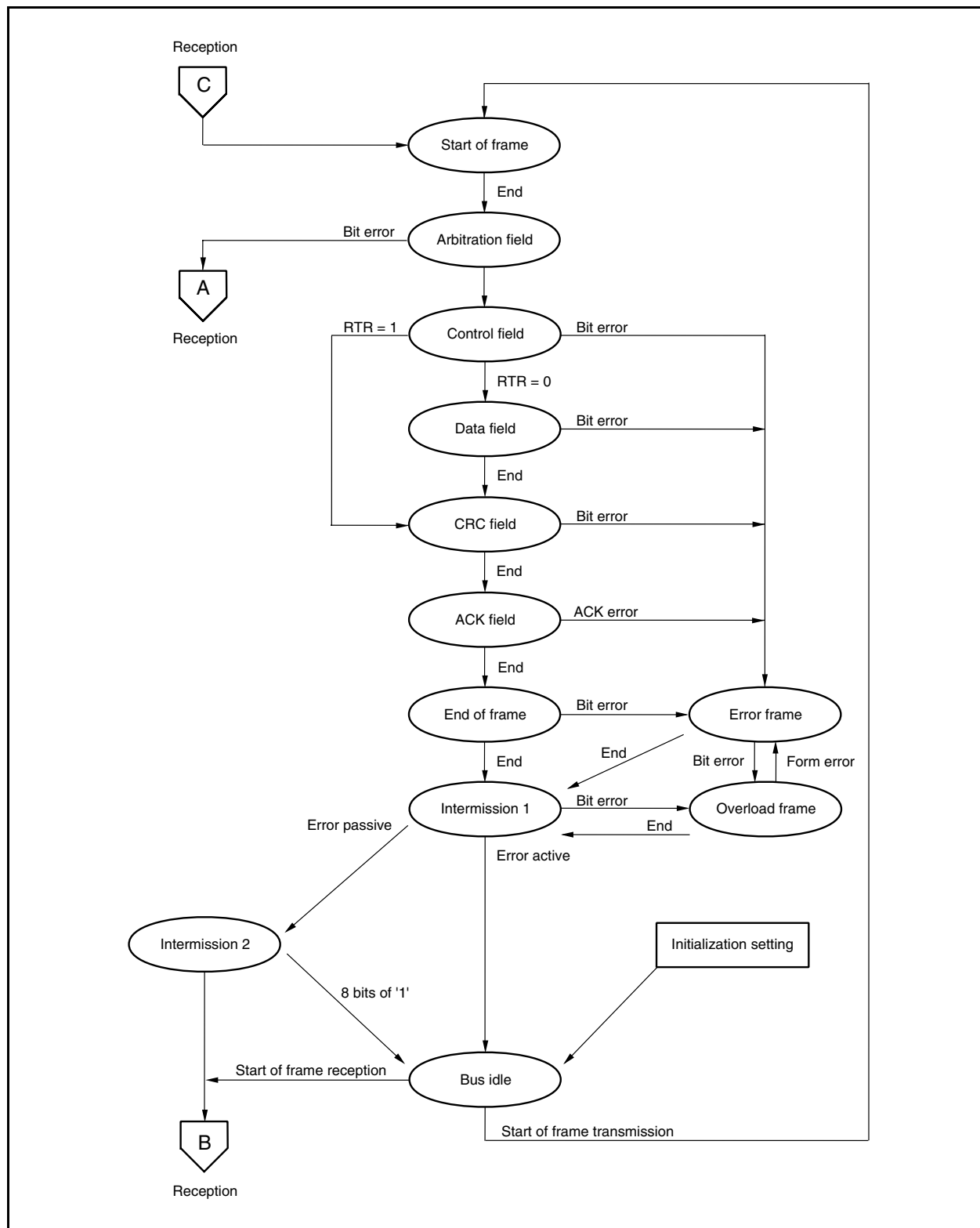
Figure 19-20. Transmission State Transition Chart
