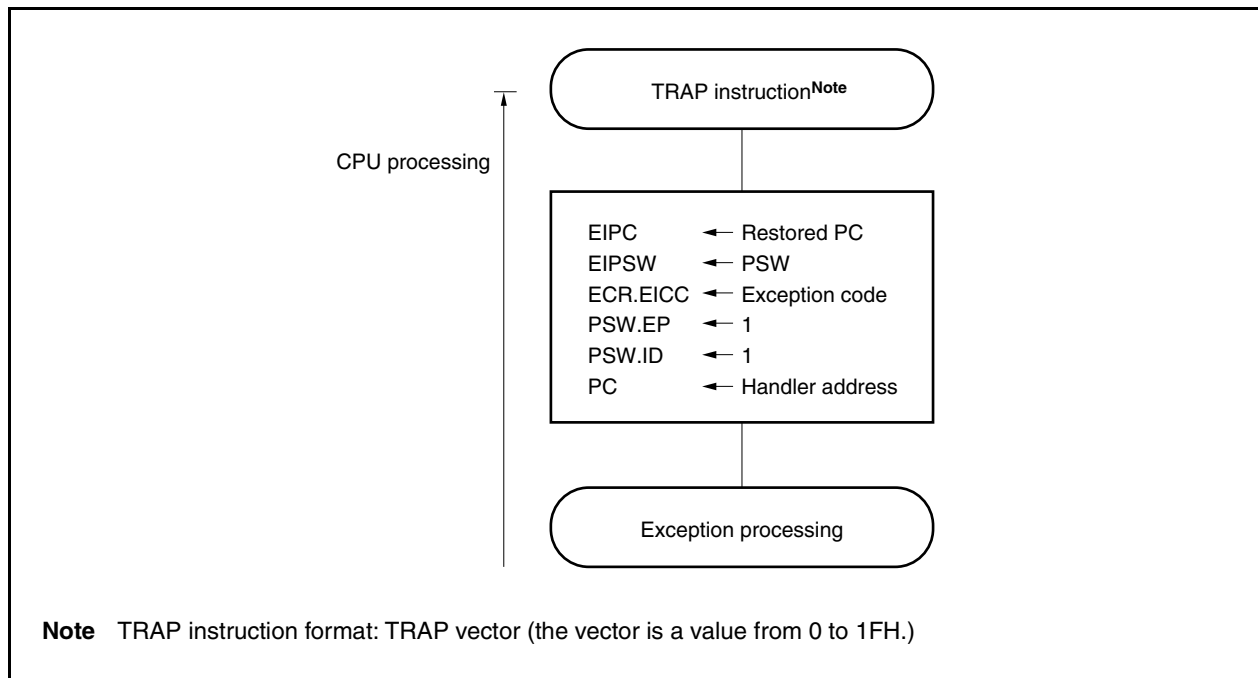
Figure 22-8. Software Exception Processing
