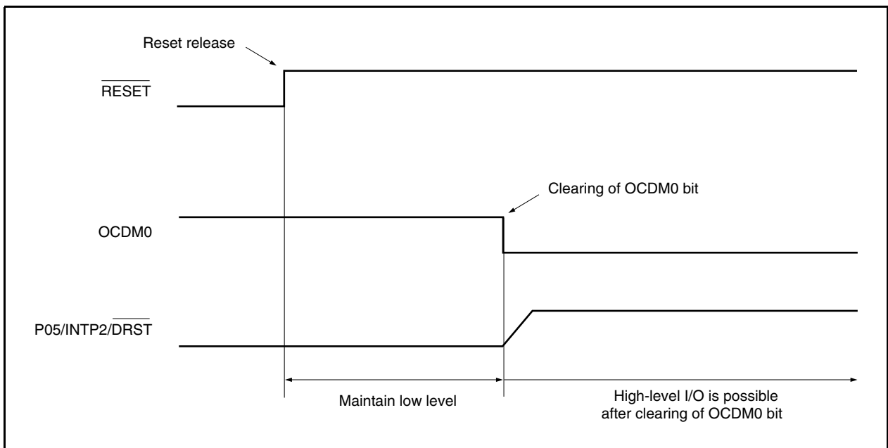
Figure 3-15. Timing When On-Chip Debug Function Is Not Used
