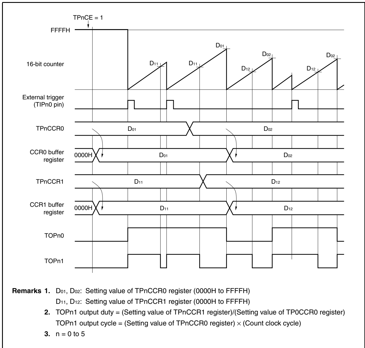
Figure 7-11. Basic Operation Timing in External Trigger Pulse Output Mode
