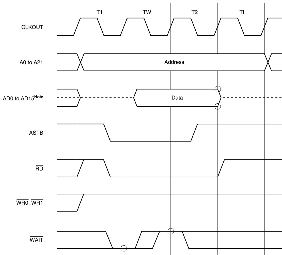
Figure 5-16. When Wait State (1 Wait) and Idle State Are Inserted
