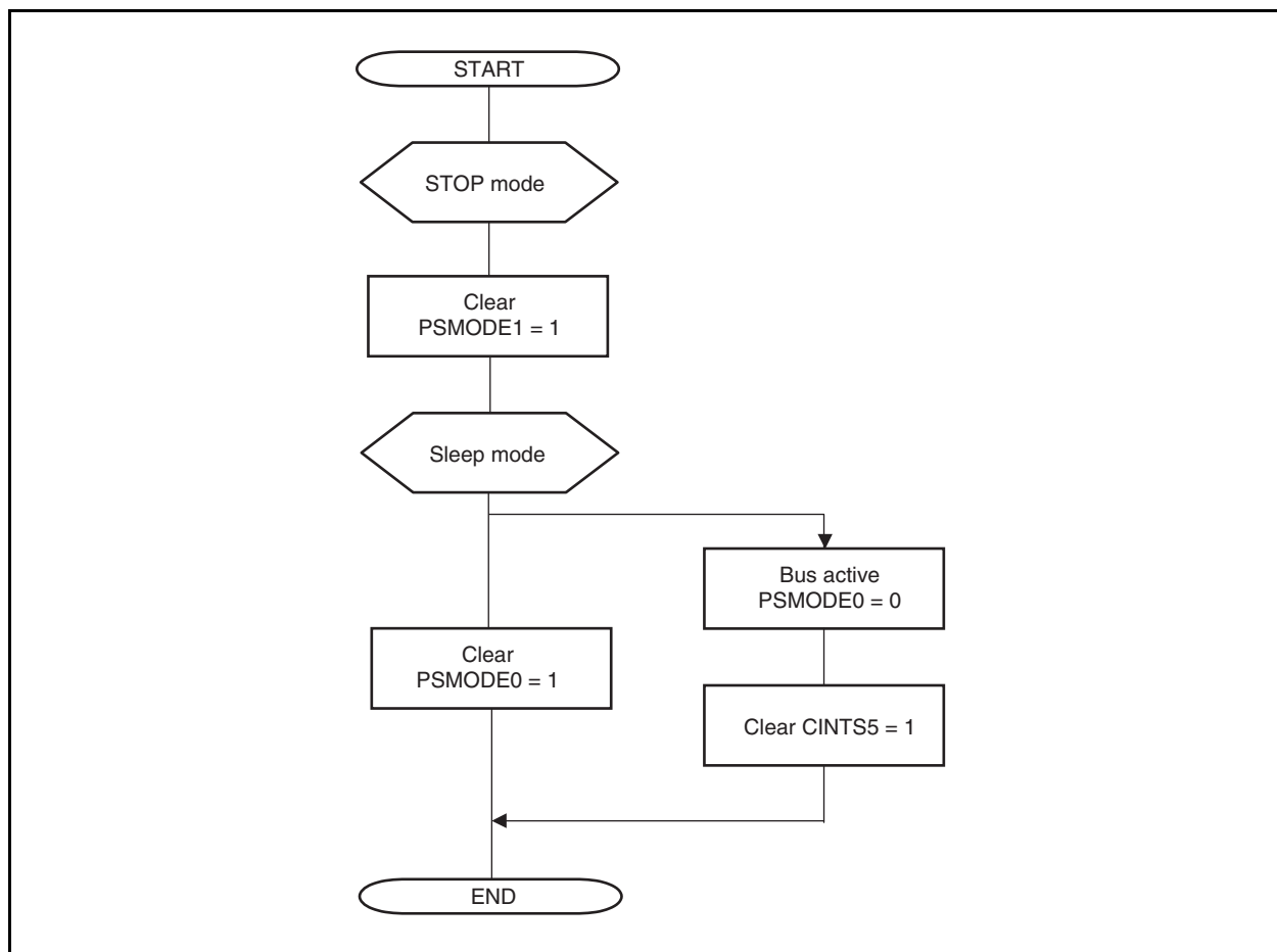
Figure 19-59. Clear CAN Sleep/Stop Mode
