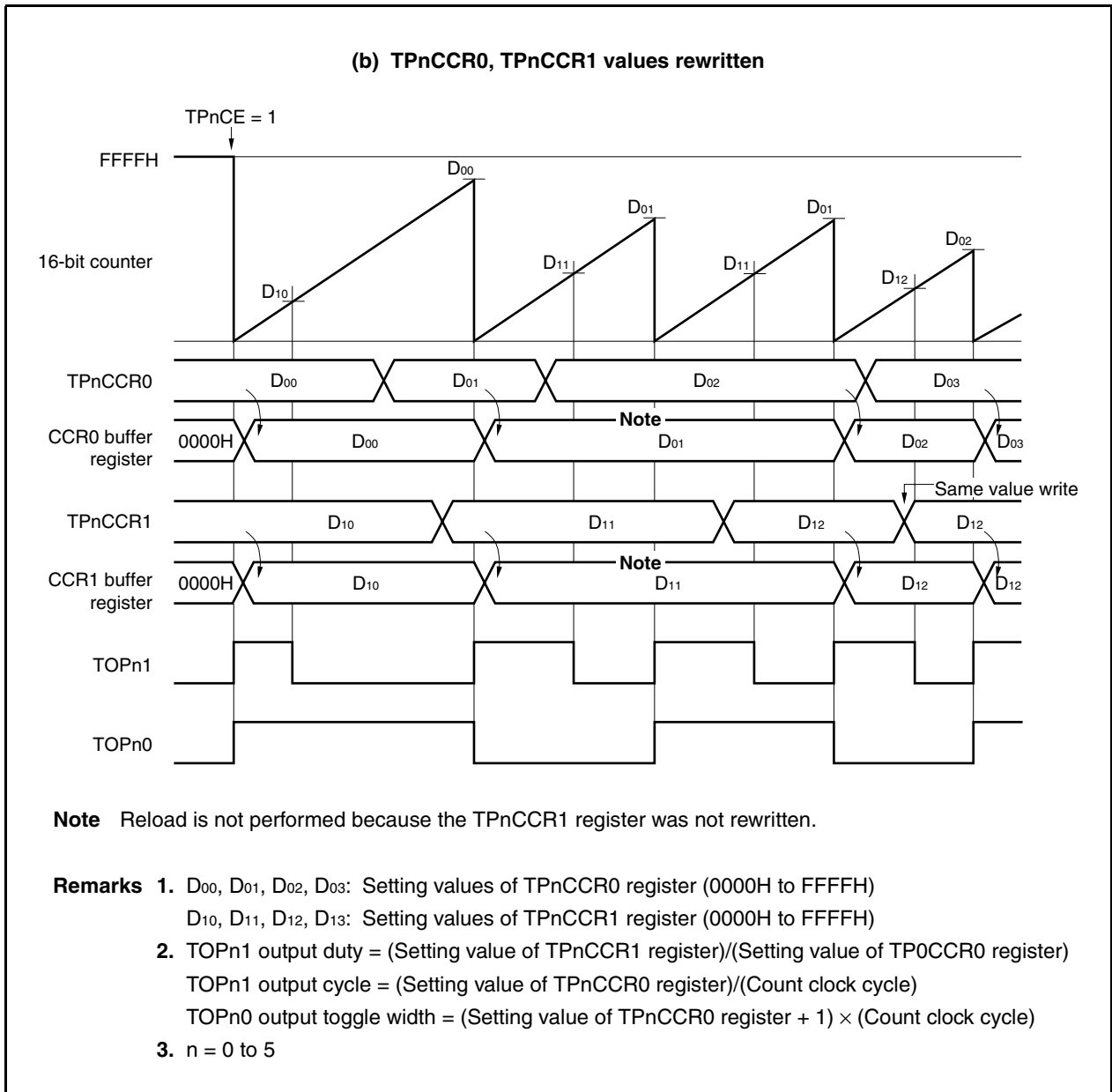
Figure 7-15. Basic Operation Timing in PWM Mode (2/2)
