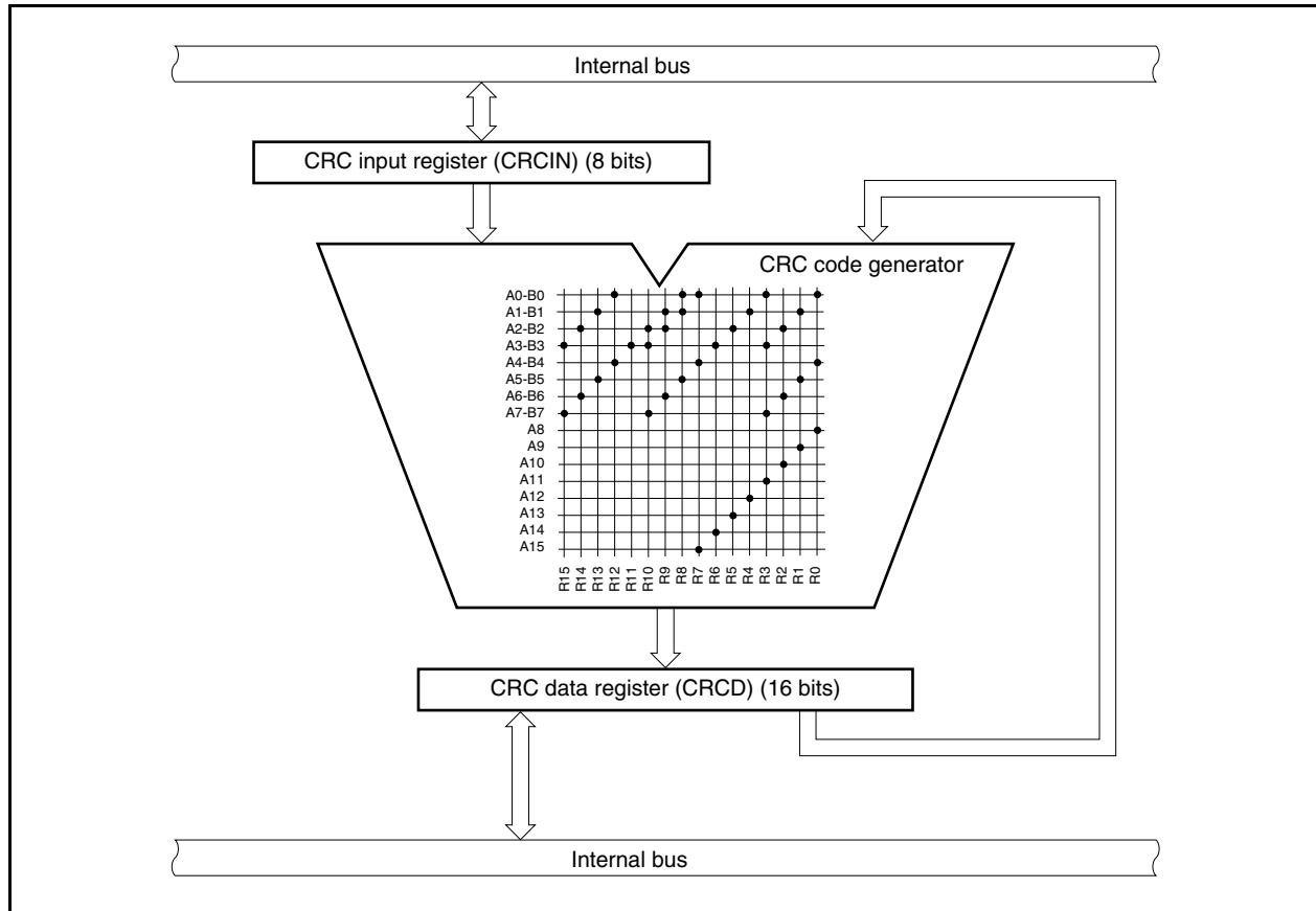
Figure 21-1. Block Diagram of CRC Register
