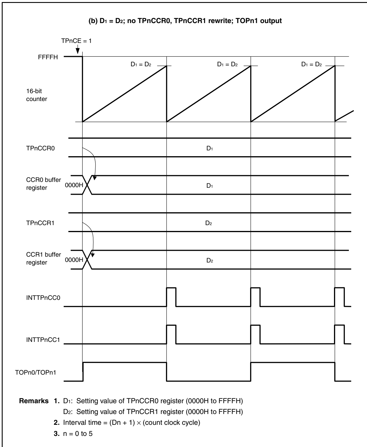
Figure 7-7. Basic Operation Timing in Interval Timer Mode (2/2)
