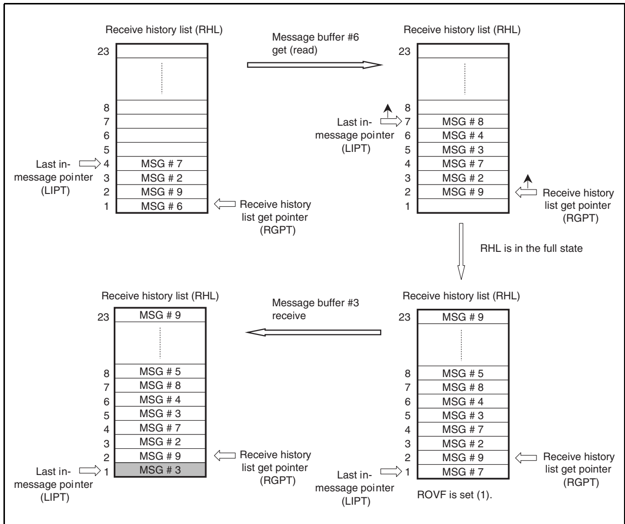
Figure 19-33. Receive History List
