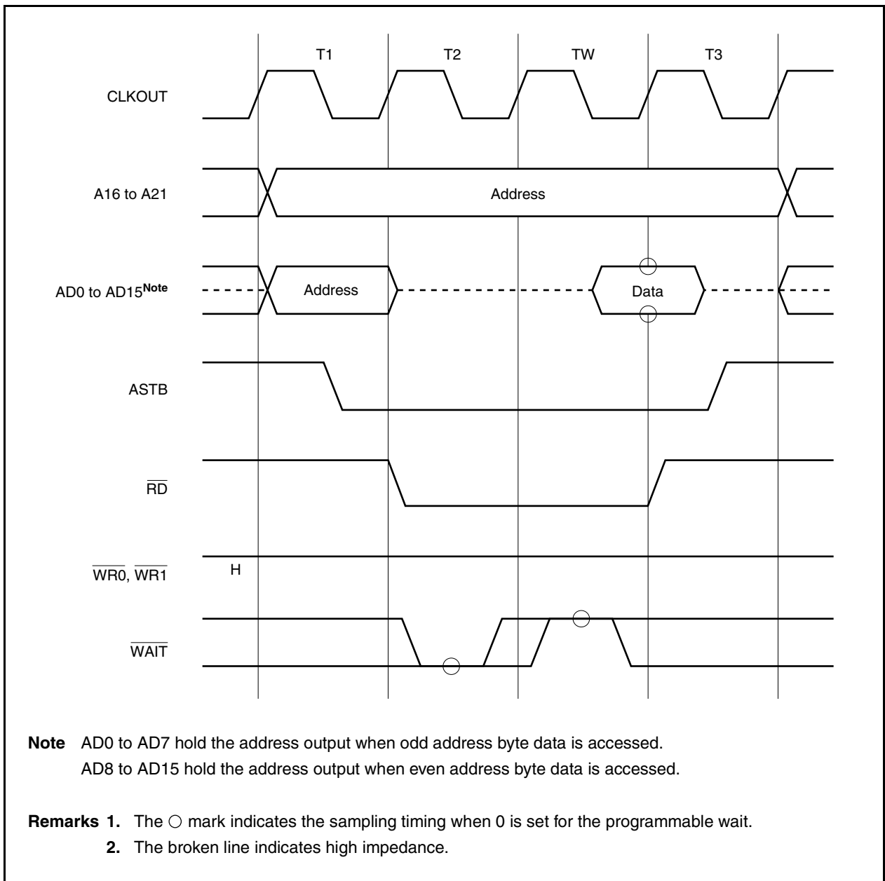
Figure 5-5. When Wait State (1 Wait) Is Inserted
