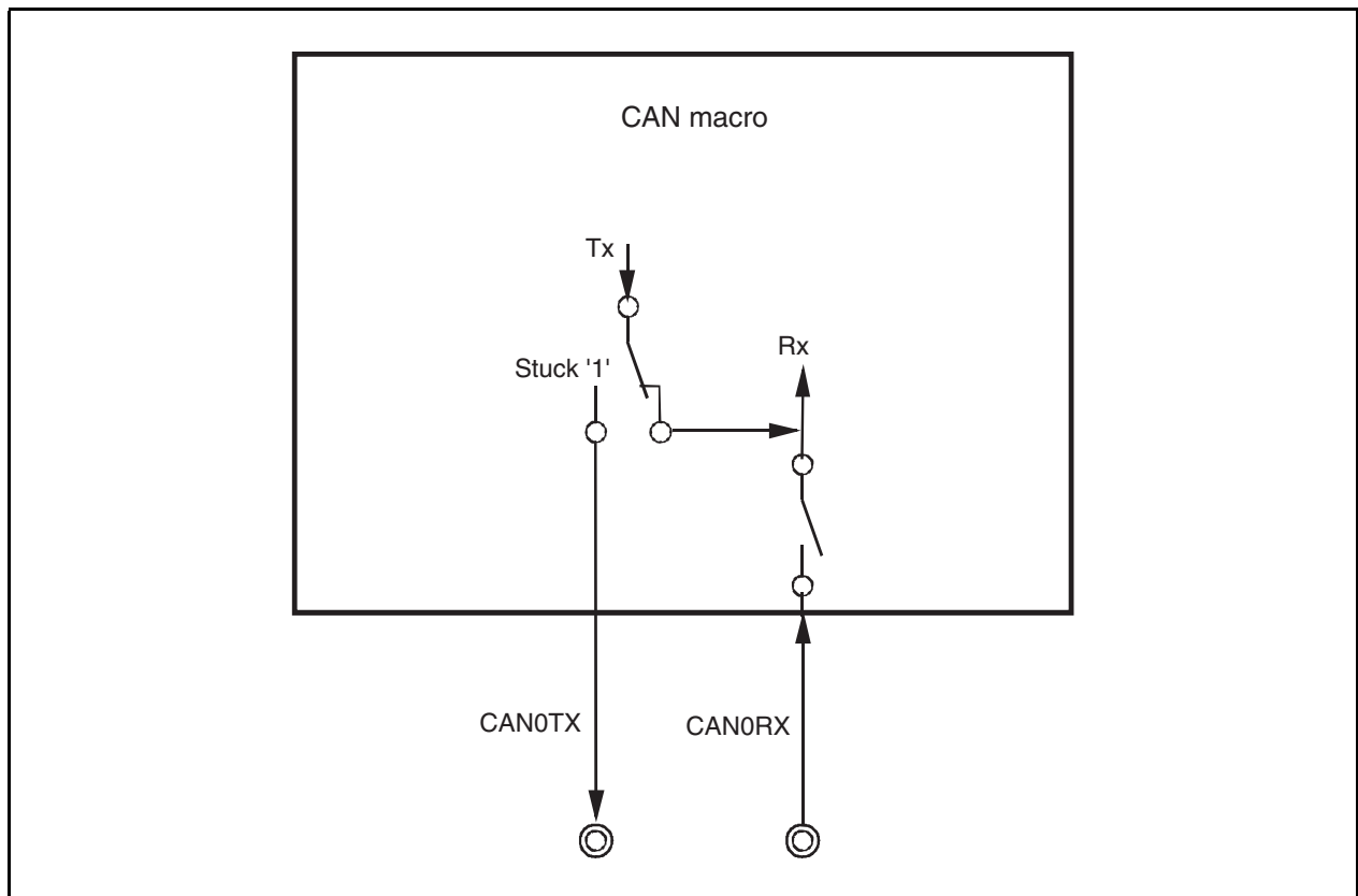
Figure 19-41. CAN Module Terminal Connection in Self-Test Mode
