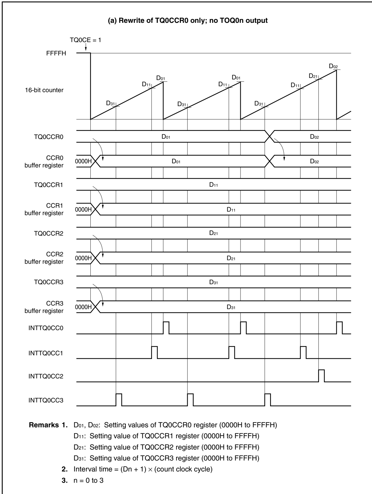
Figure 8-9. Basic Operation Timing in External Event Count Mode (1/2)
