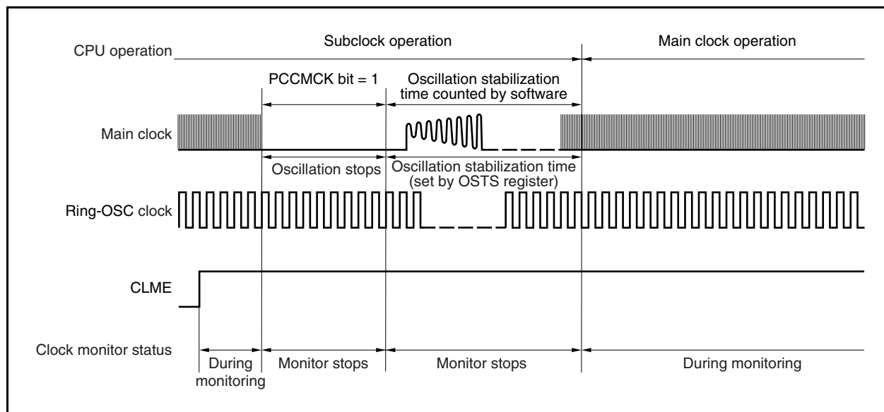
Figure 25-7. Operation When Main Clock Is Stopped
