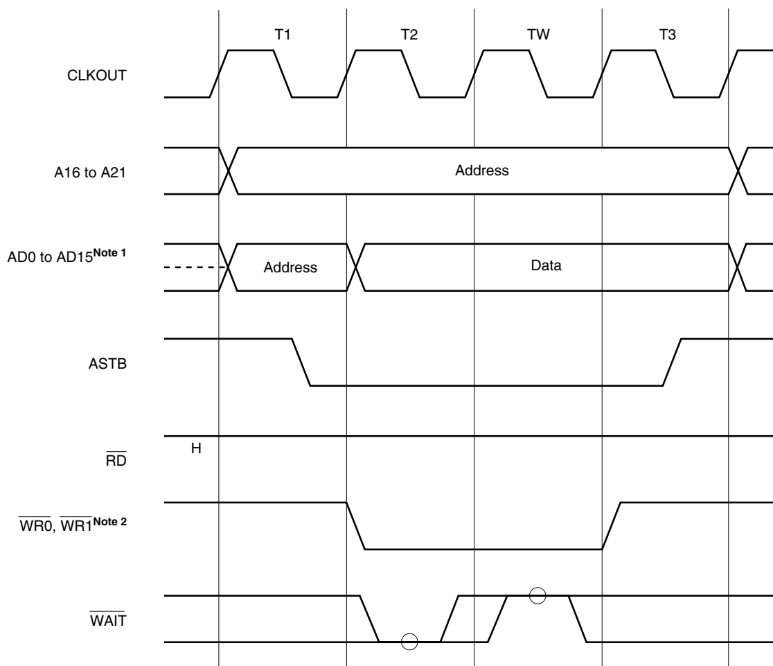
Figure 5-10. When Wait State (1 Wait) Is Inserted
