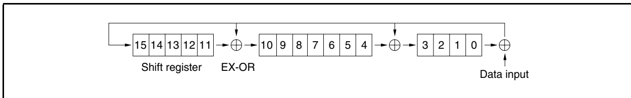
Figure 21-3. Operation Circuit Configuration (CRC Data Register)
