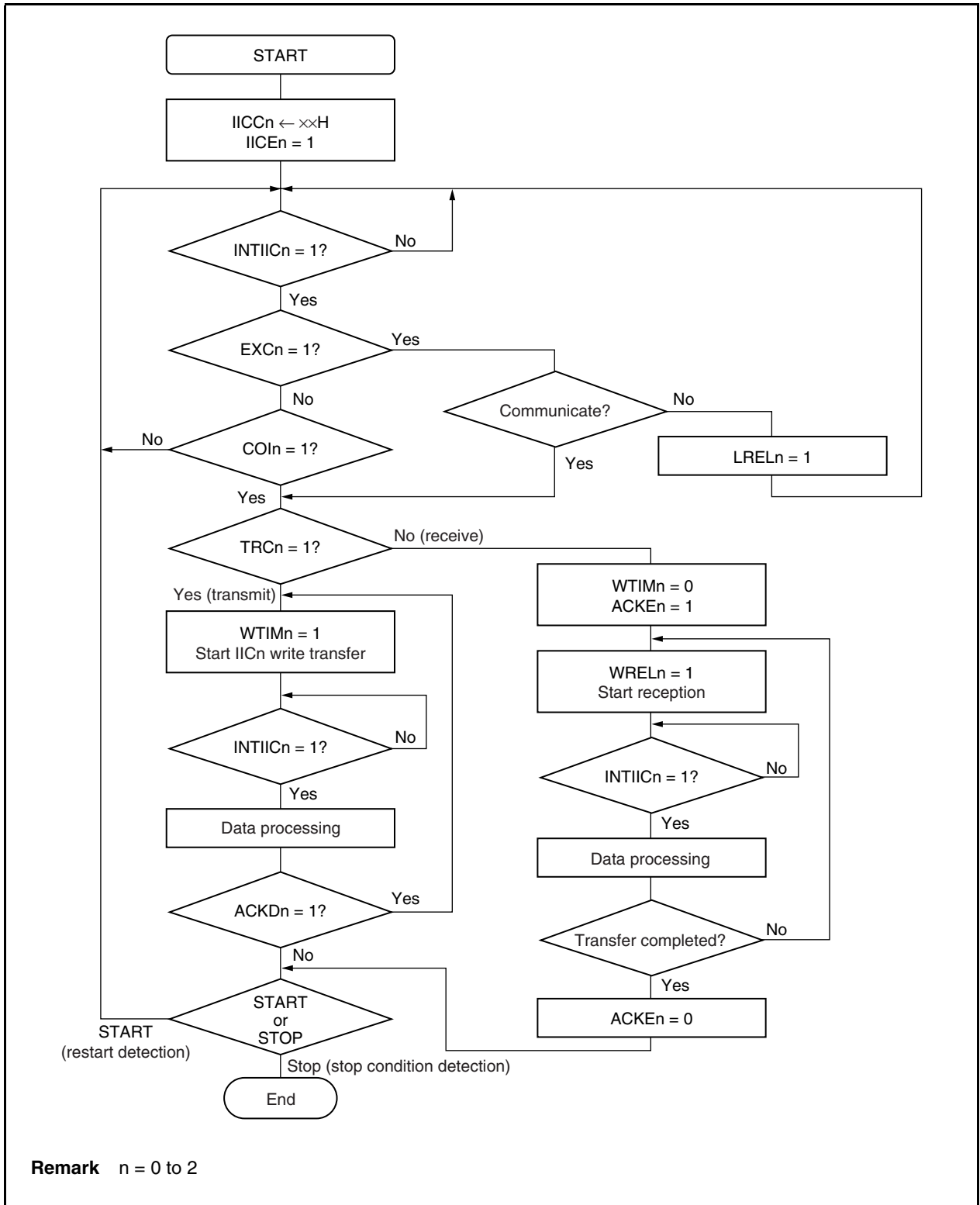
Figure 17-20. Slave Operation Flowchart
