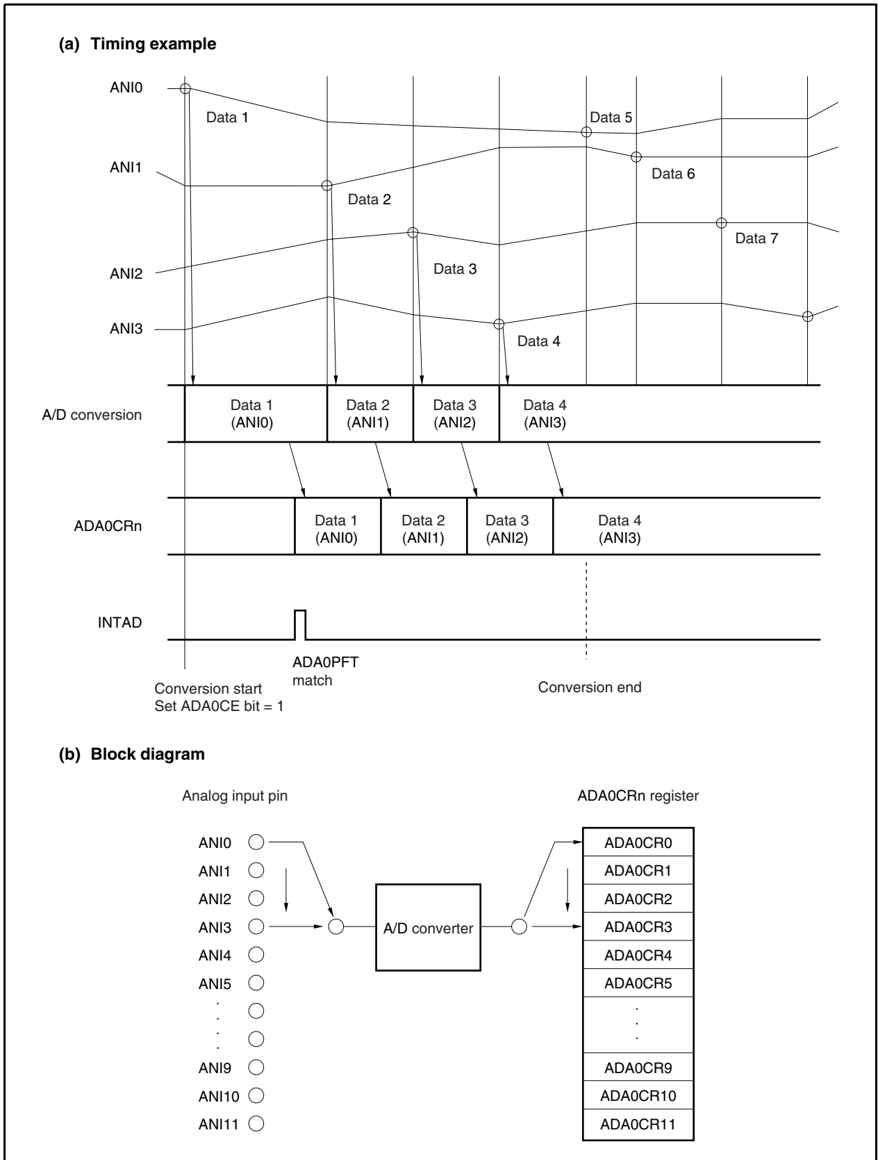
Figure 13-11. Timing Example of One-Shot Scan Mode Operation (When Power-Fail Compare Is Made: ADA0S Register = 03H)
