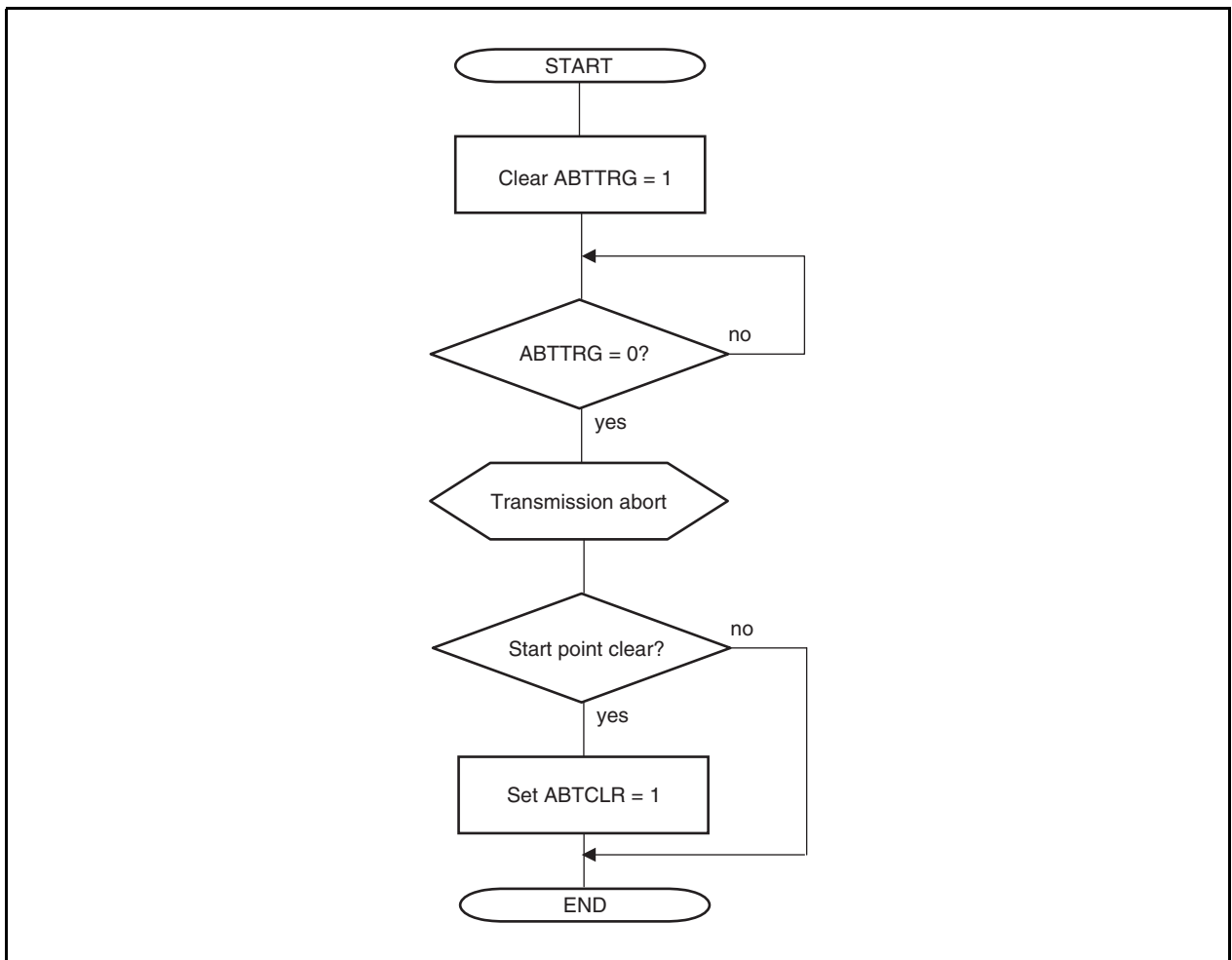
Figure 19-54. Transmission Request Abort Process (ABT Mode)
