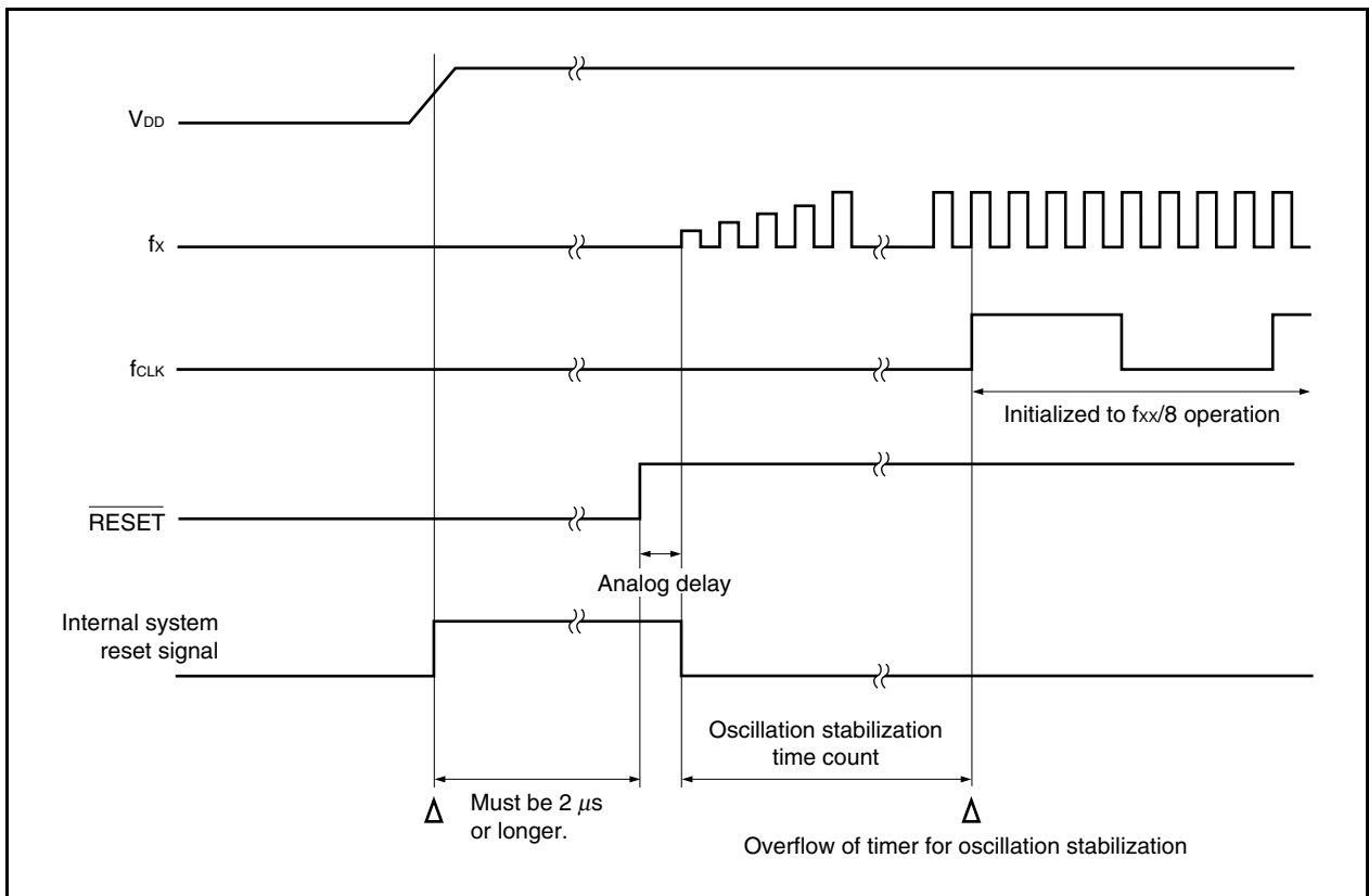
Figure 25-2. Timing of Power-on Reset Operation
