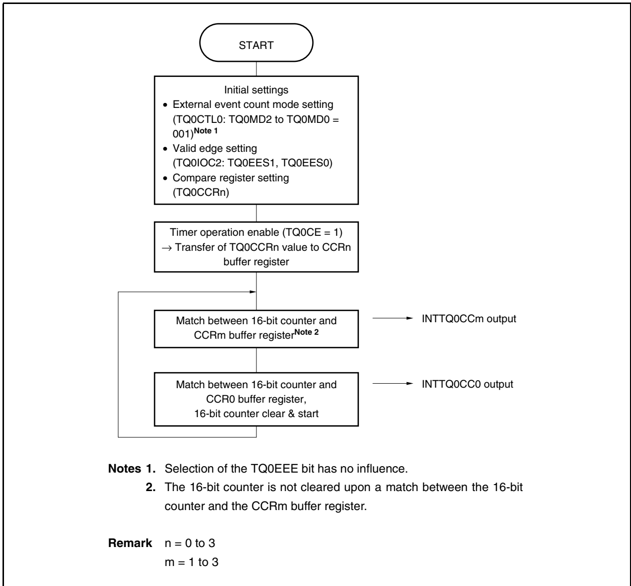
Figure 8-8. Flowchart of Basic Operation in External Event Count Mode
