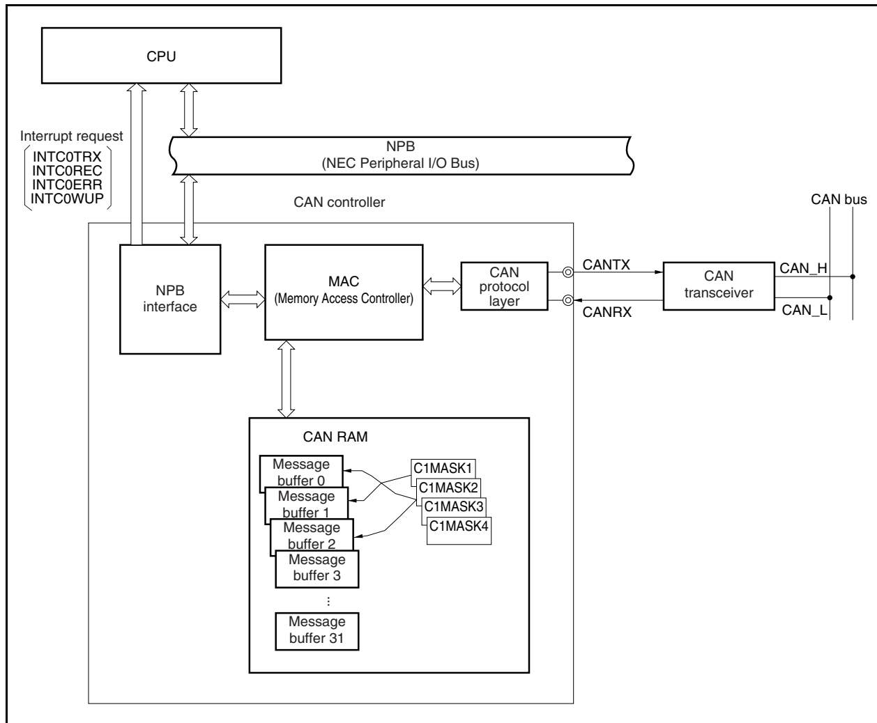
Figure 19-1. Block Diagram of CAN Module
