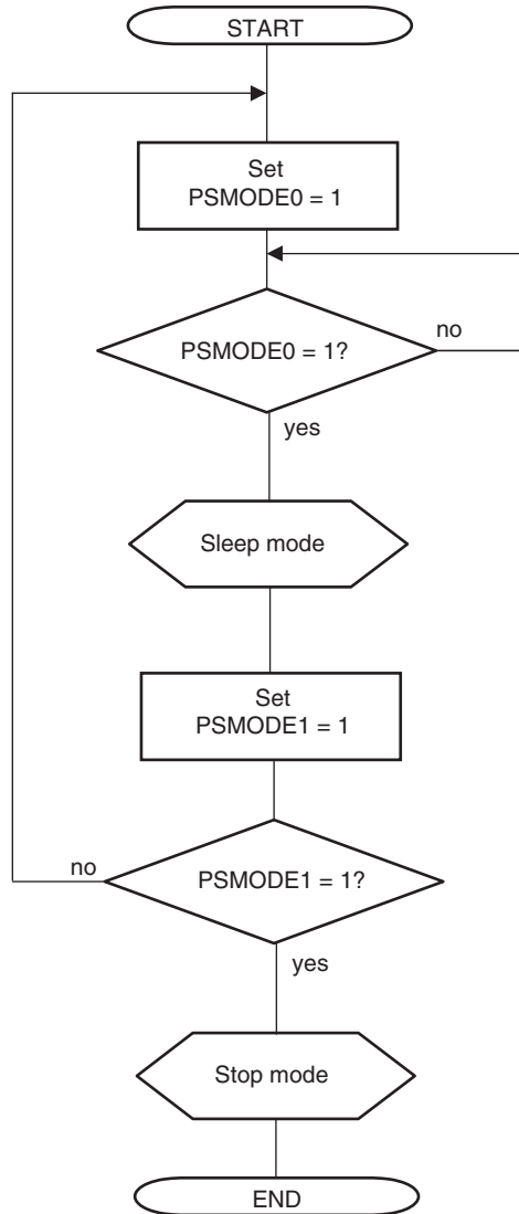
Figure 19-58. Setting CAN Sleep/Stop Mode
