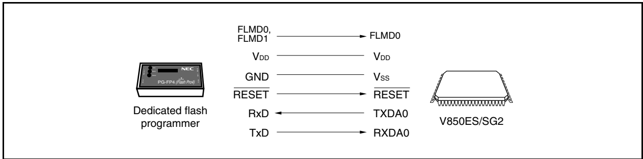
Figure 28-2. Communication with Dedicated Flash Programmer (UARTA0)
