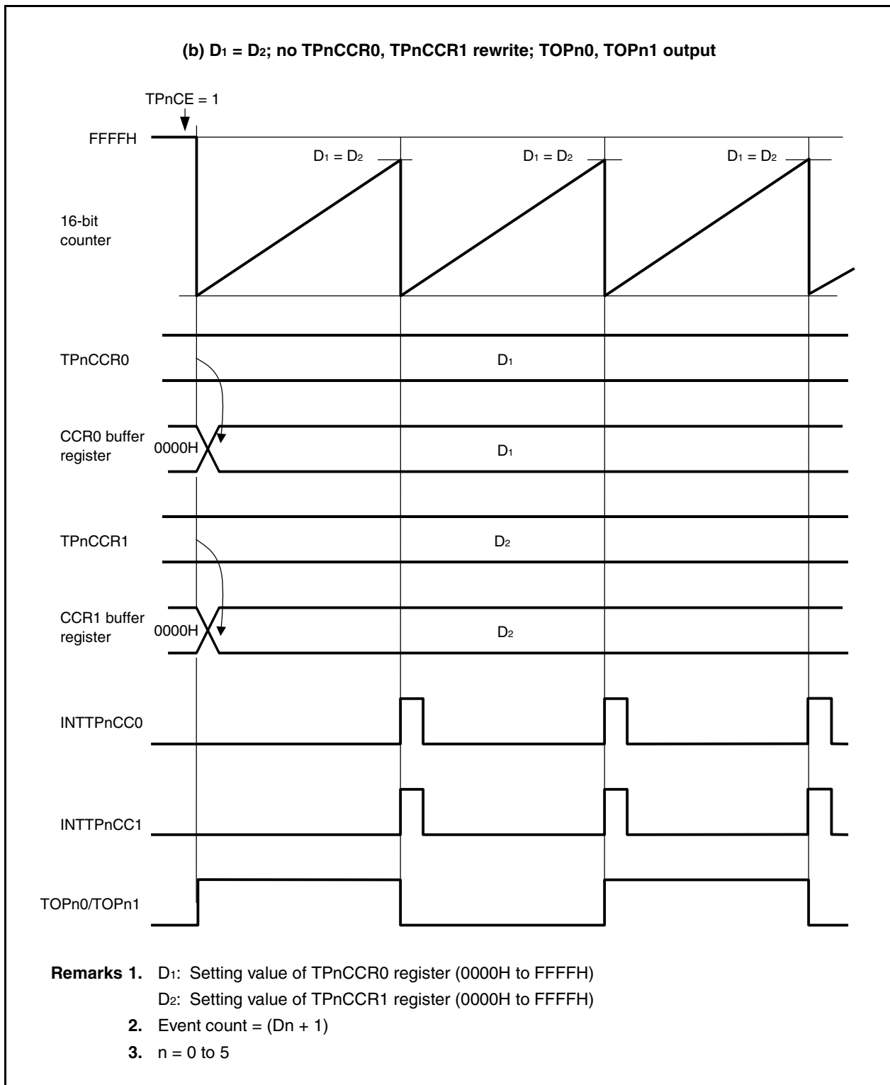
Figure 7-9. Basic Operation Timing in External Event Count Mode (2/2)
