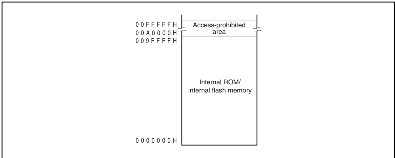
Figure 3-8. Internal ROM/Internal Flash Memory Area (640 KB)
