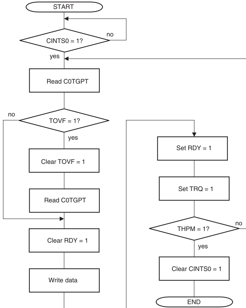
Figure 19-52. Transmit Software Polling
