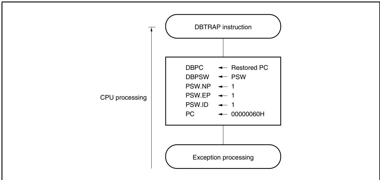
Figure 22-12. Debug Trap Processing Format
