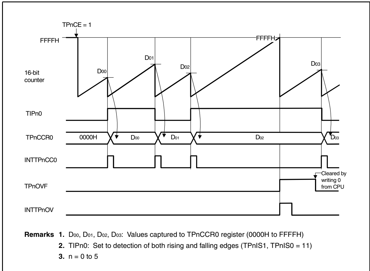
Figure 7-22. Basic Operation Timing in Pulse Width Measurement Mode
