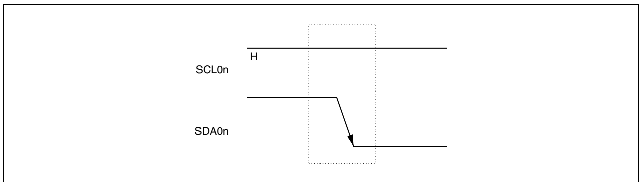
Figure 17-8. Start Conditions
