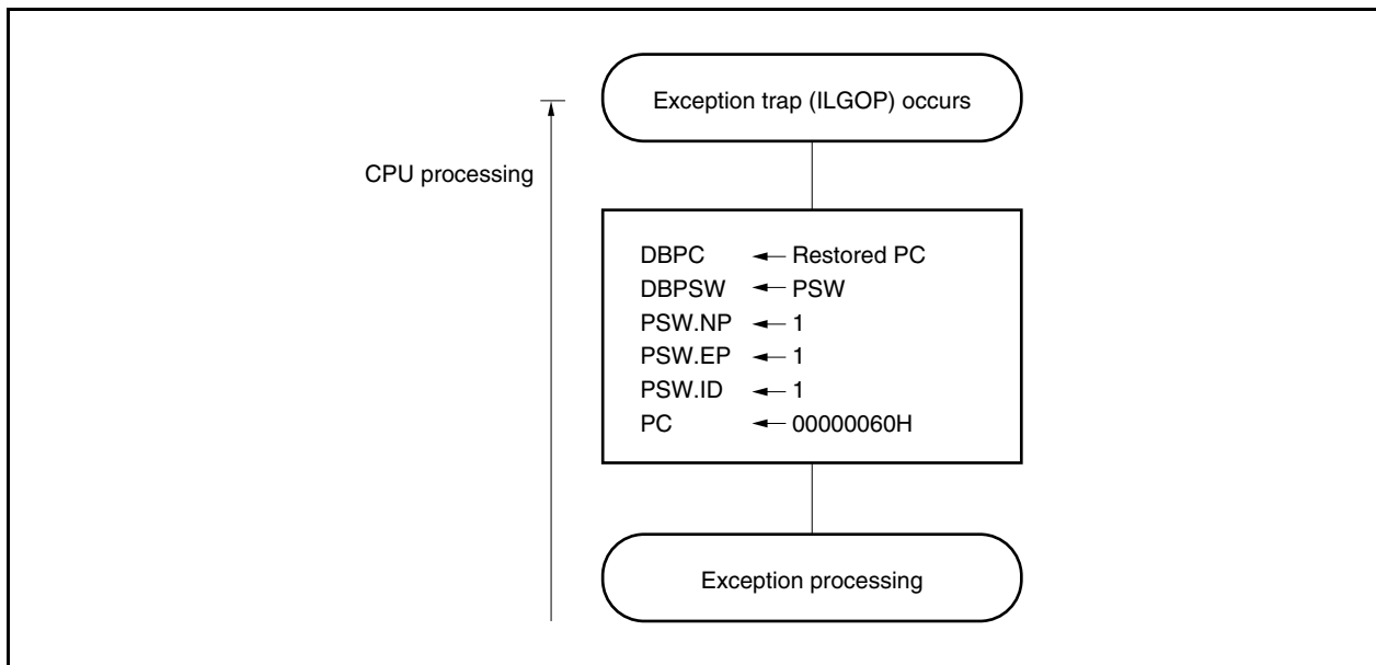
Figure 22-10. Exception Trap Processing
