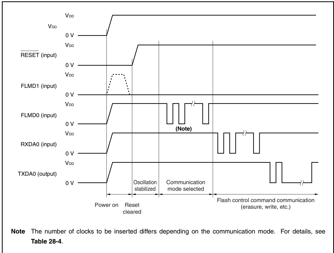
Figure 28-11. Flash Memory Programming Mode
