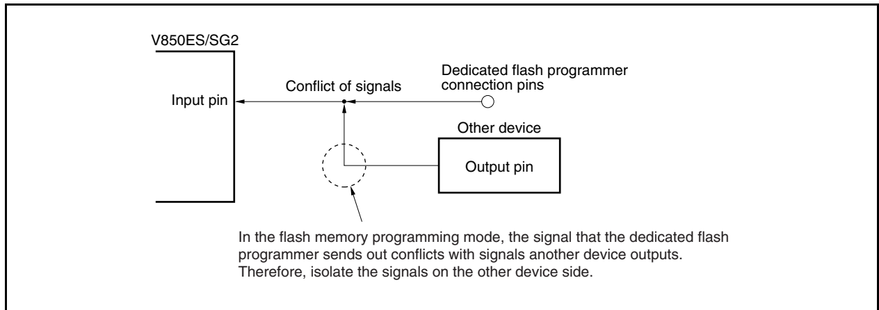
Figure 28-7. Conflict of Signals (Serial Interface Input Pin)
