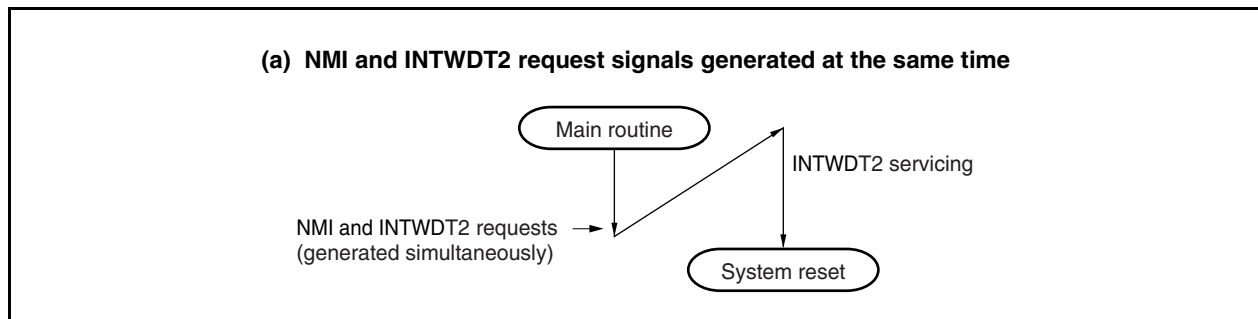
Figure 22-1. Non-Maskable Interrupt Request Signal Acknowledgment Operation (1/2)
