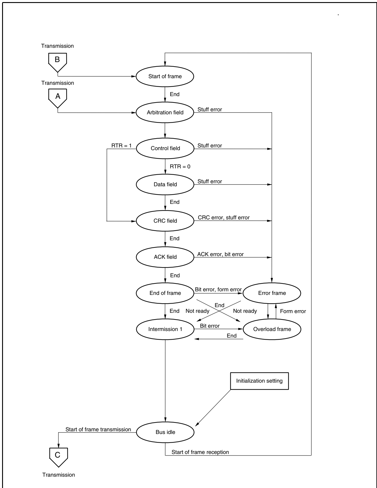
Figure 19-21. Reception State Transition Chart
