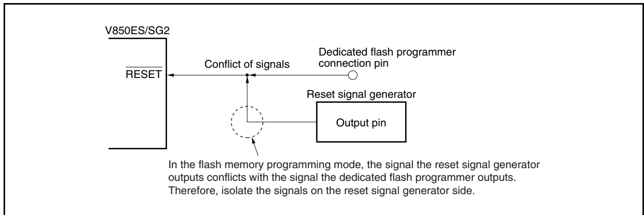
Figure 28-9. Conflict of Signals ( \overline{\text{RESET}} Pin)
