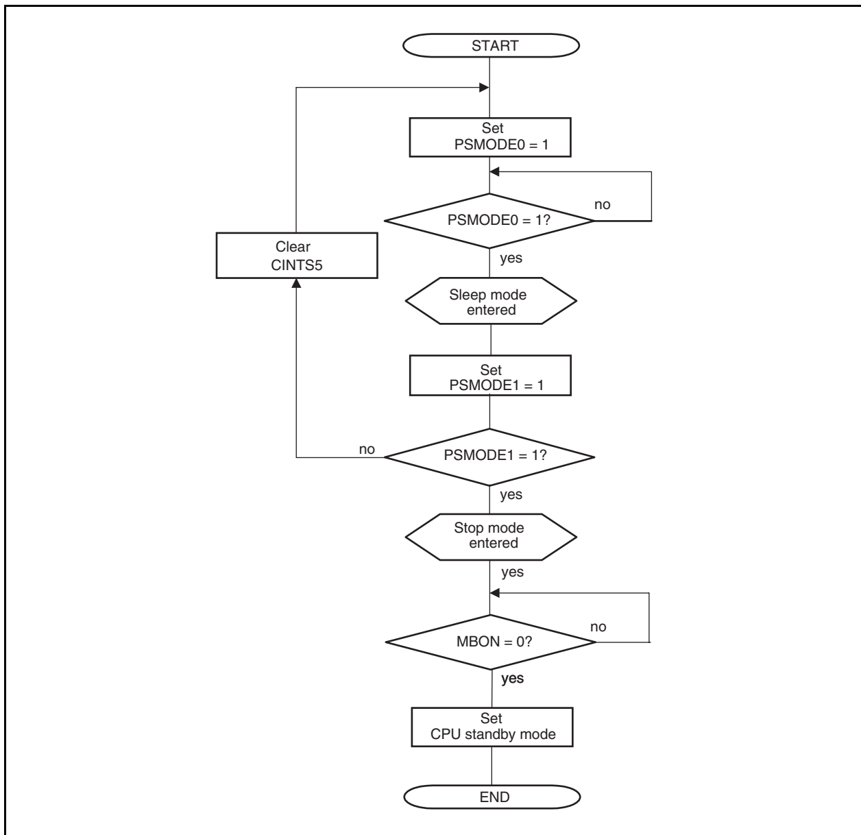
Figure 19-65. Setting CPU Standby (from CAN Stop Mode)
