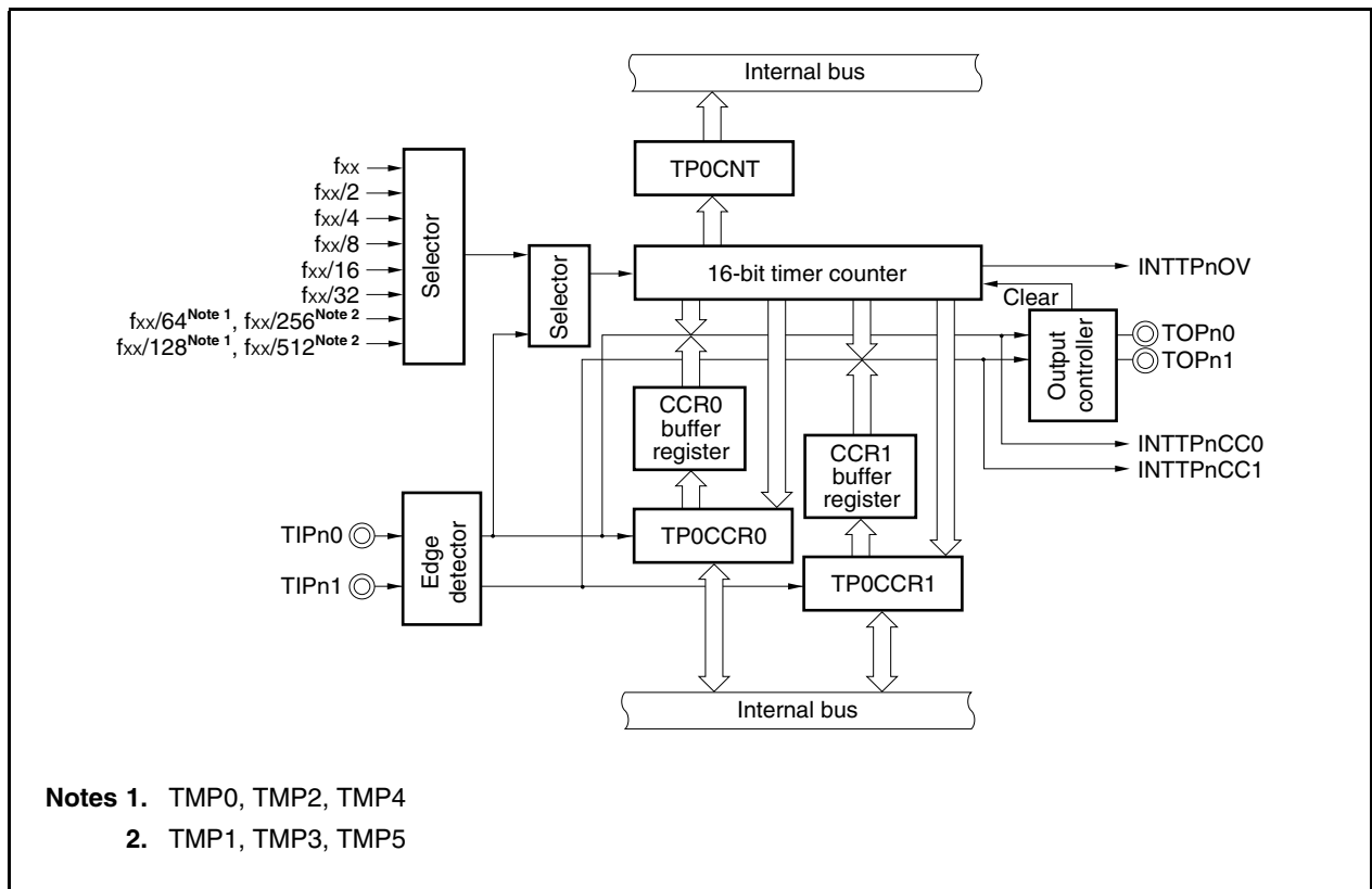
Figure 7-1. Block Diagram of Timer P
