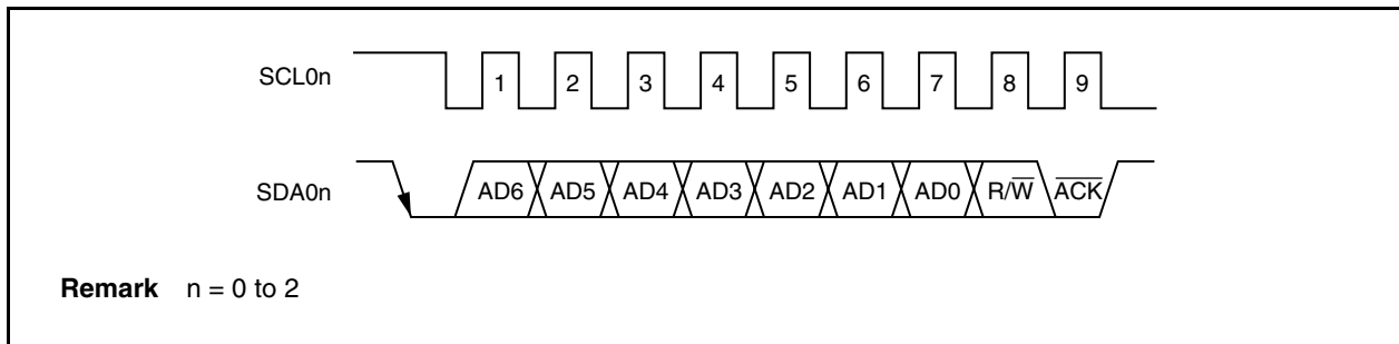
Figure 17-11. \overline{\text{ACK}} Signal
