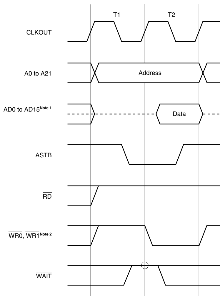
Figure 5-18. Basic Bus Cycle
