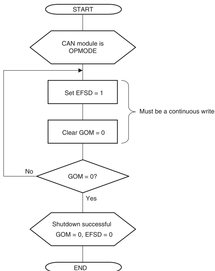
Figure 19-62. Shutdown Process (Forcible Shutdown)
