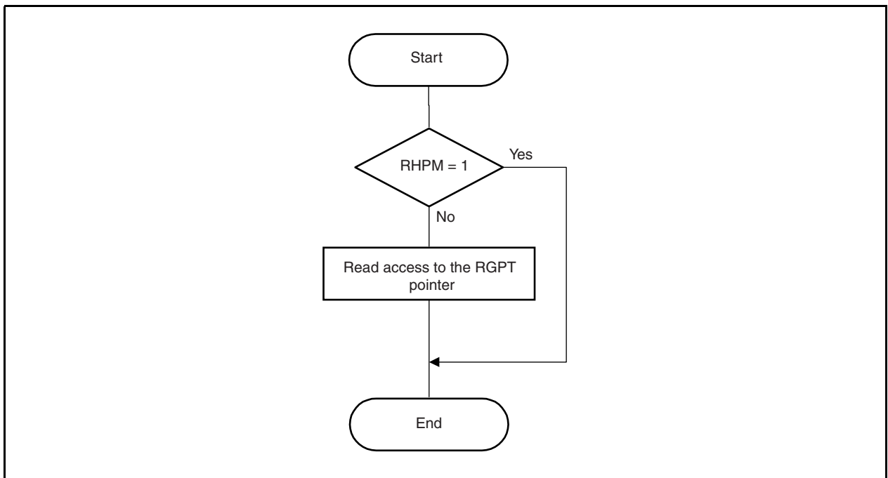
Figure 19-35. C0RGPT Pointer Handling with Respect to RHPM Bit
