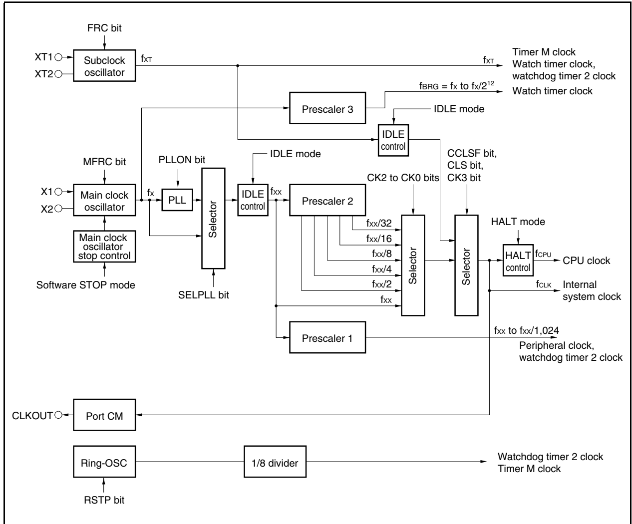
Figure 6-1. Clock Generator
