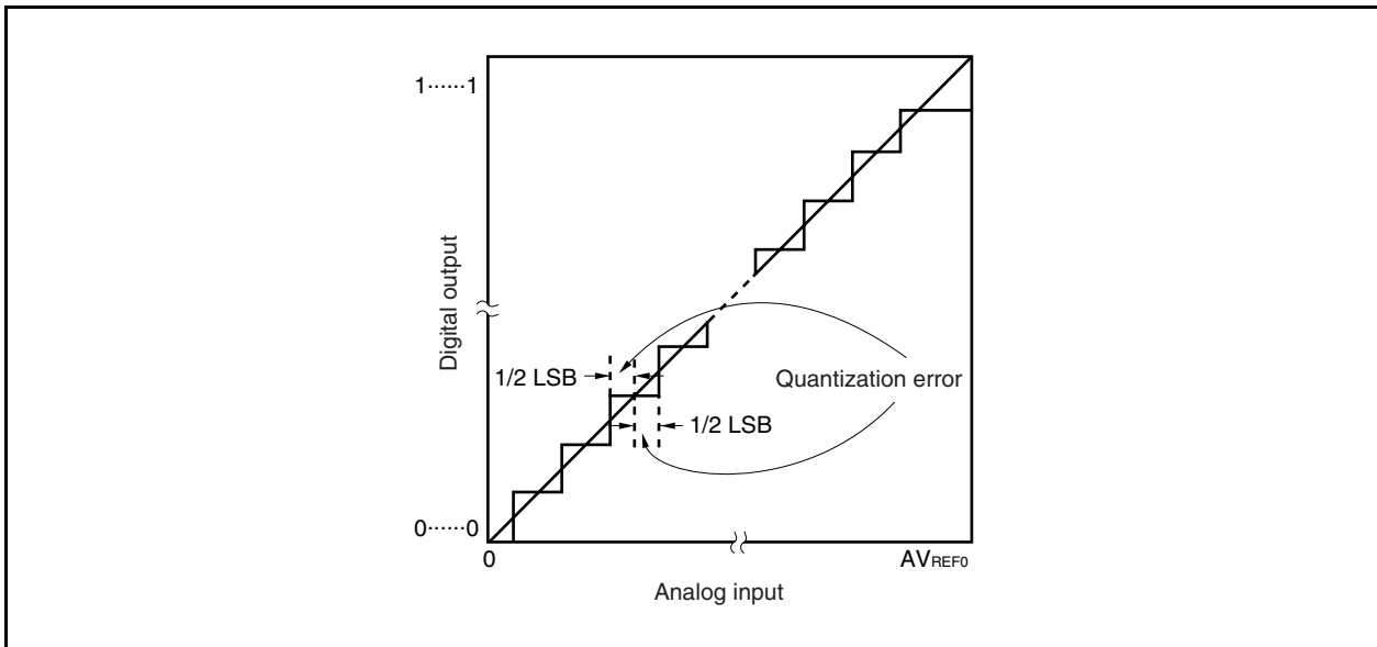
Figure 13-16. Quantization Error
