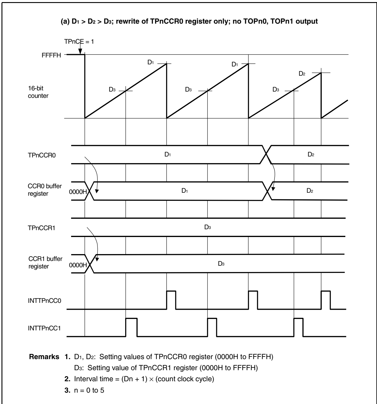
Figure 7-7. Basic Operation Timing in Interval Timer Mode (1/2)
