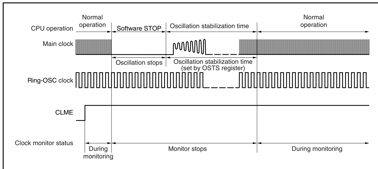
Figure 25-6. Operation in Software STOP Mode and After Software STOP Mode Is Released
