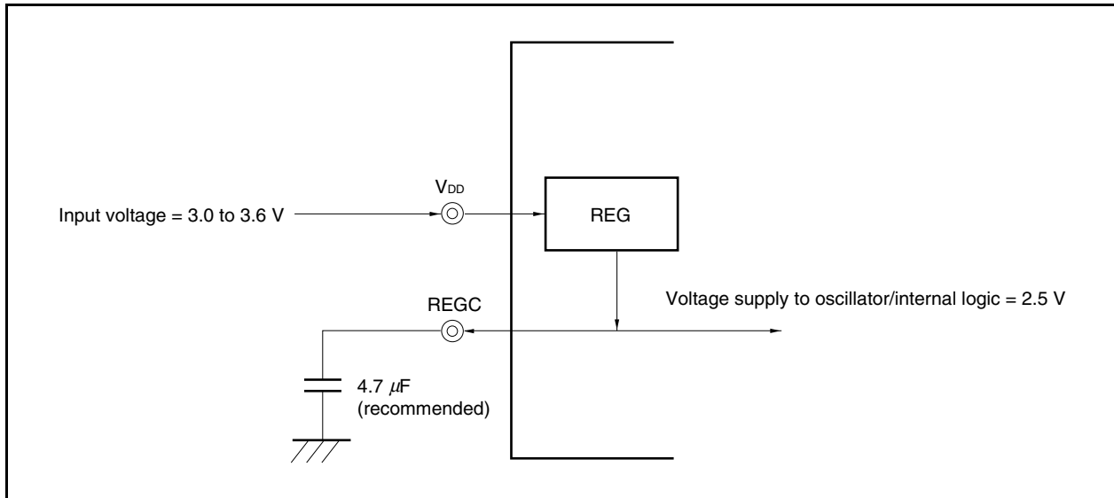
Figure 26-2. REGC Pin Connection (REGC = Capacity)
