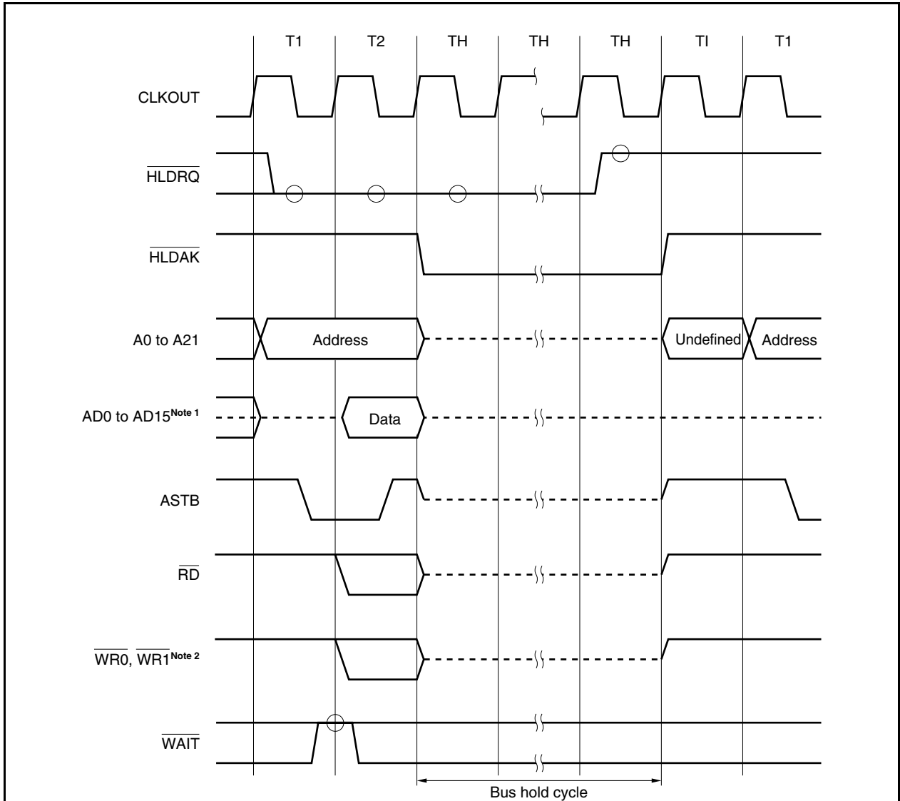
Figure 5-21. Bus Hold Cycle
