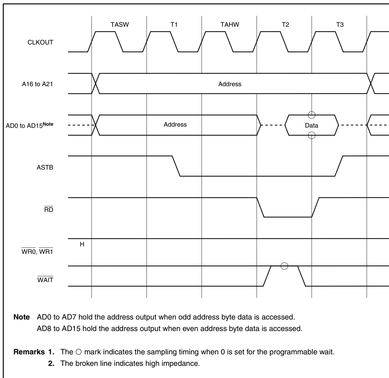
Figure 5-8. When Address Wait State Is Inserted
