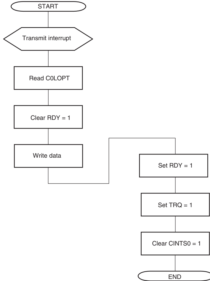
Figure 19-50. Transmission via Interrupt (C0LOPT)
