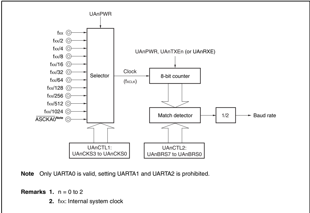
Figure 15-15. Configuration of Baud Rate Generator
