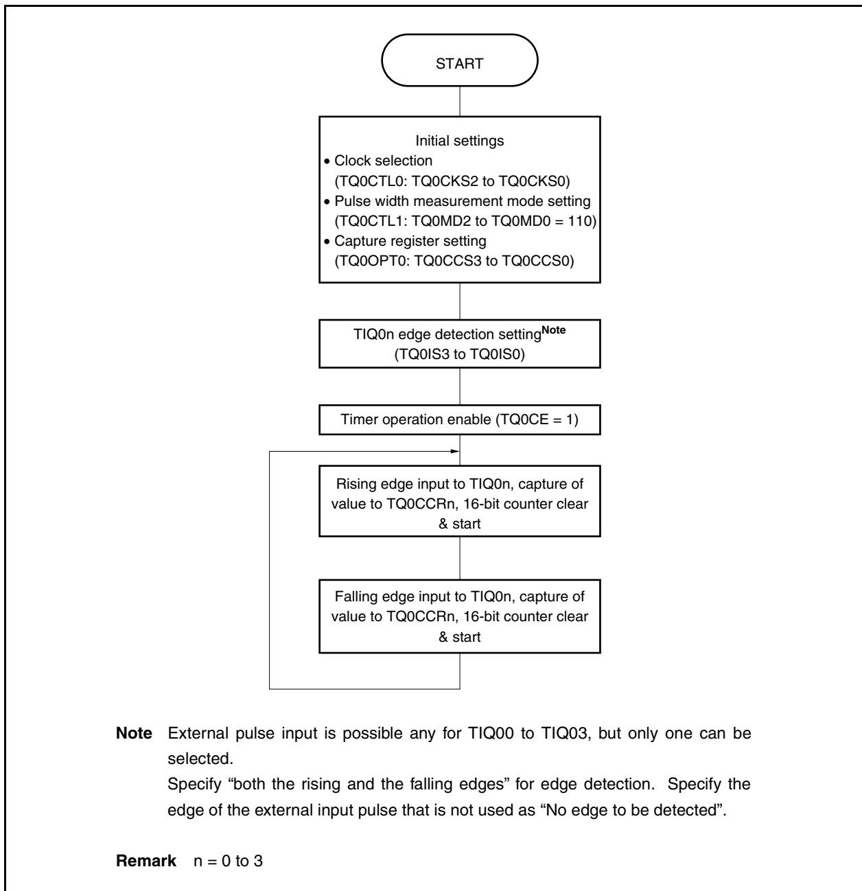
Figure 8-21. Flowchart of Basic Operation in Pulse Width Measurement Mode
