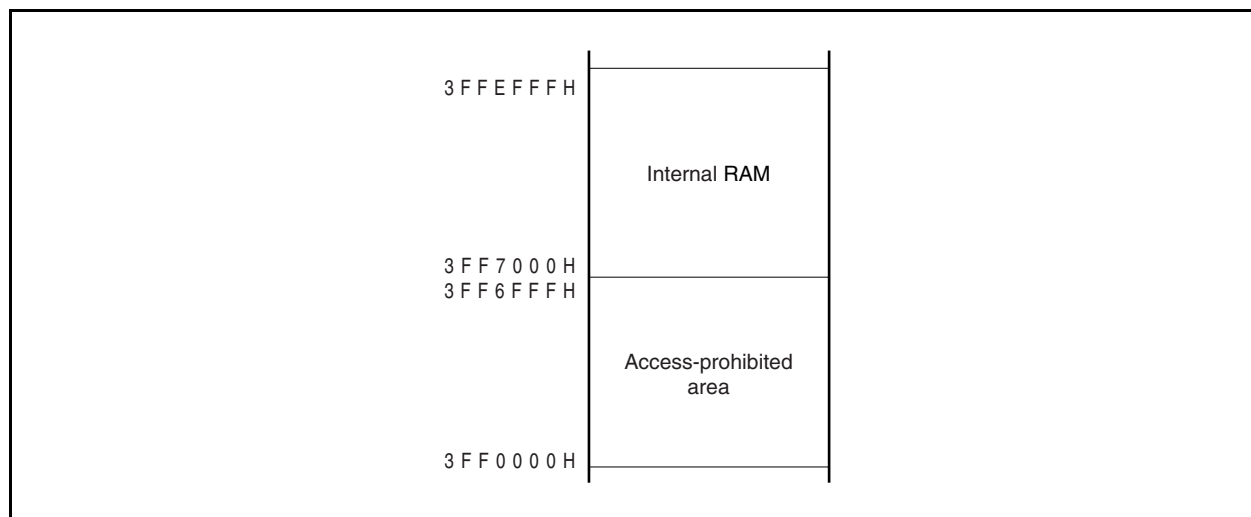
Figure 3-10. Internal RAM Area (32 KB)
