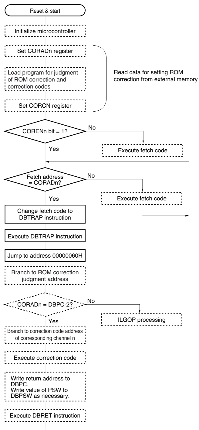
Figure 27-2. ROM Correction Operation and Program Flow
