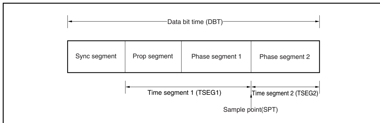
Figure 19-29. Data Bit Time
