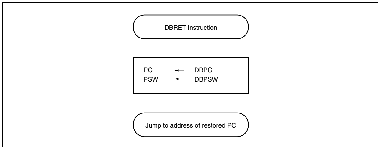
Figure 22-11. Restore Processing from Exception Trap
