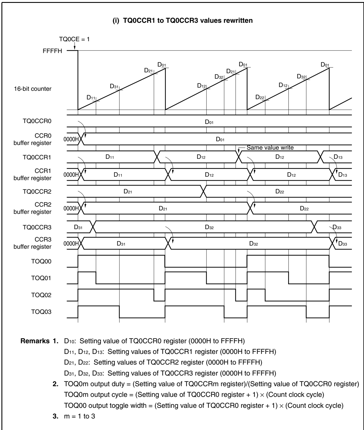
Figure 8-15. Basic Operation Timing in PWM Mode (1/2)
