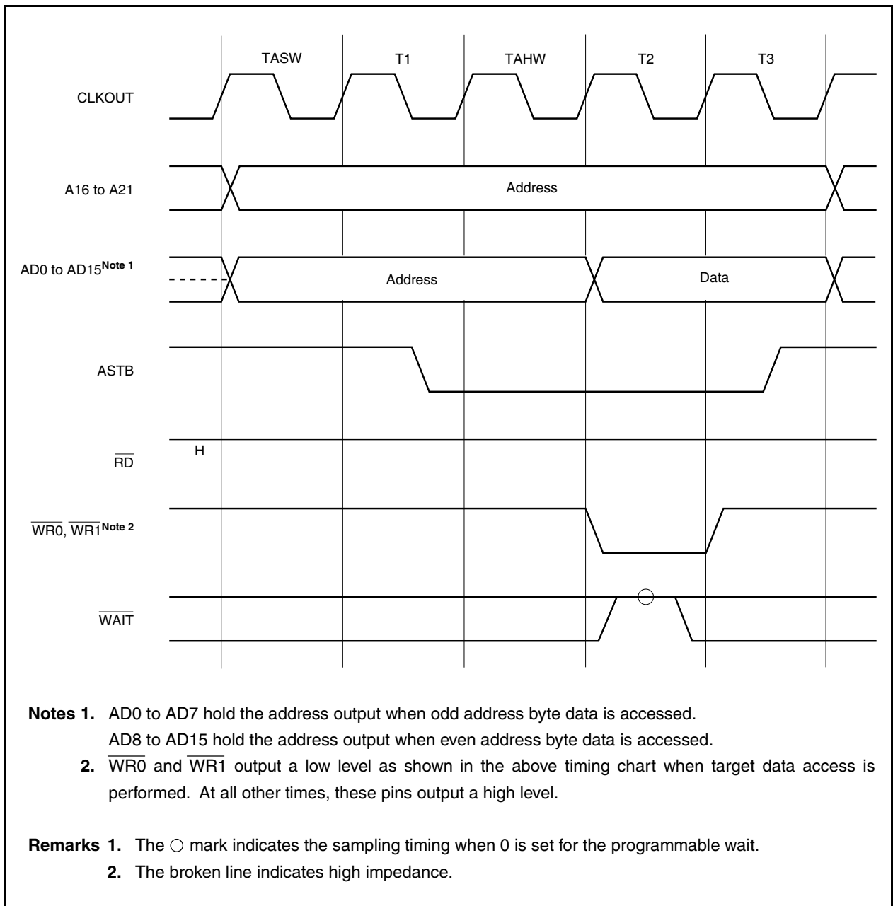
Figure 5-11. When Address Wait State Is Inserted
