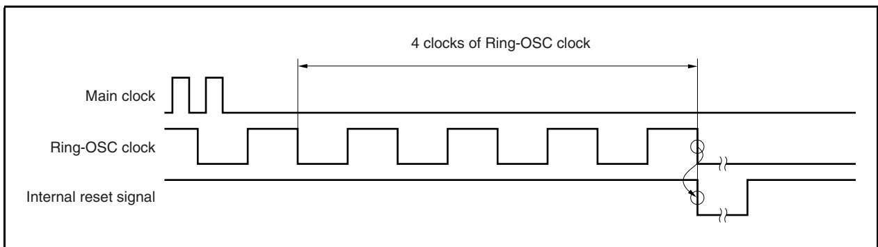
Figure 25-5. When Oscillation of Main Clock Is Stopped
