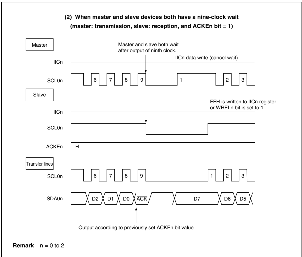
Figure 17-13. Wait Signal (2/2)
