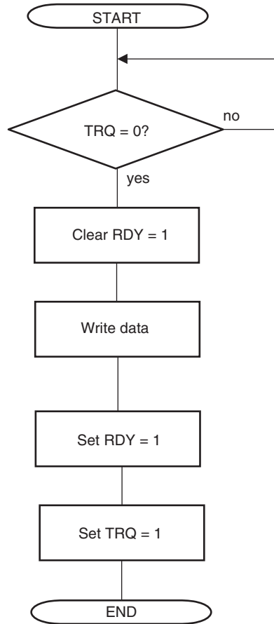
Figure 19-48. Transmit Preparation (Normal Mode)
