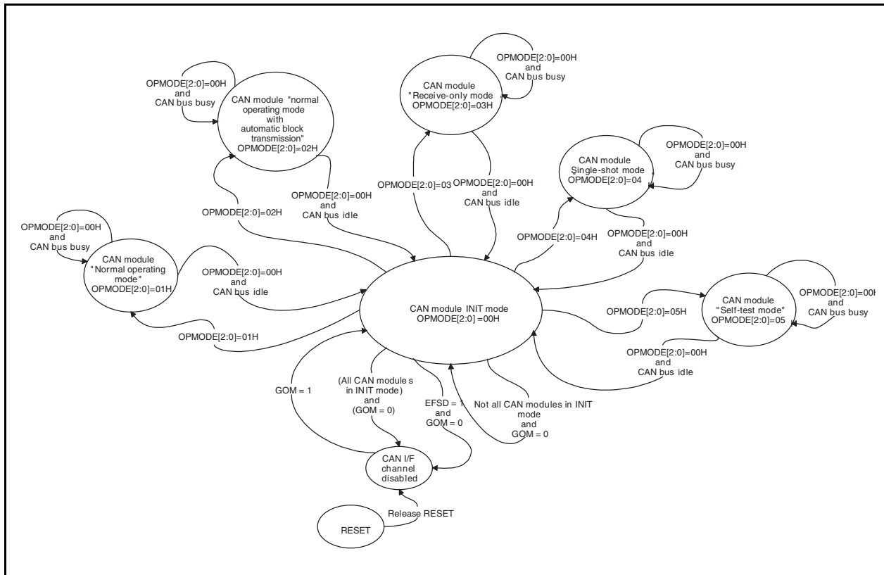
Figure 19-32. Transition to CAN Module Operational Modes
