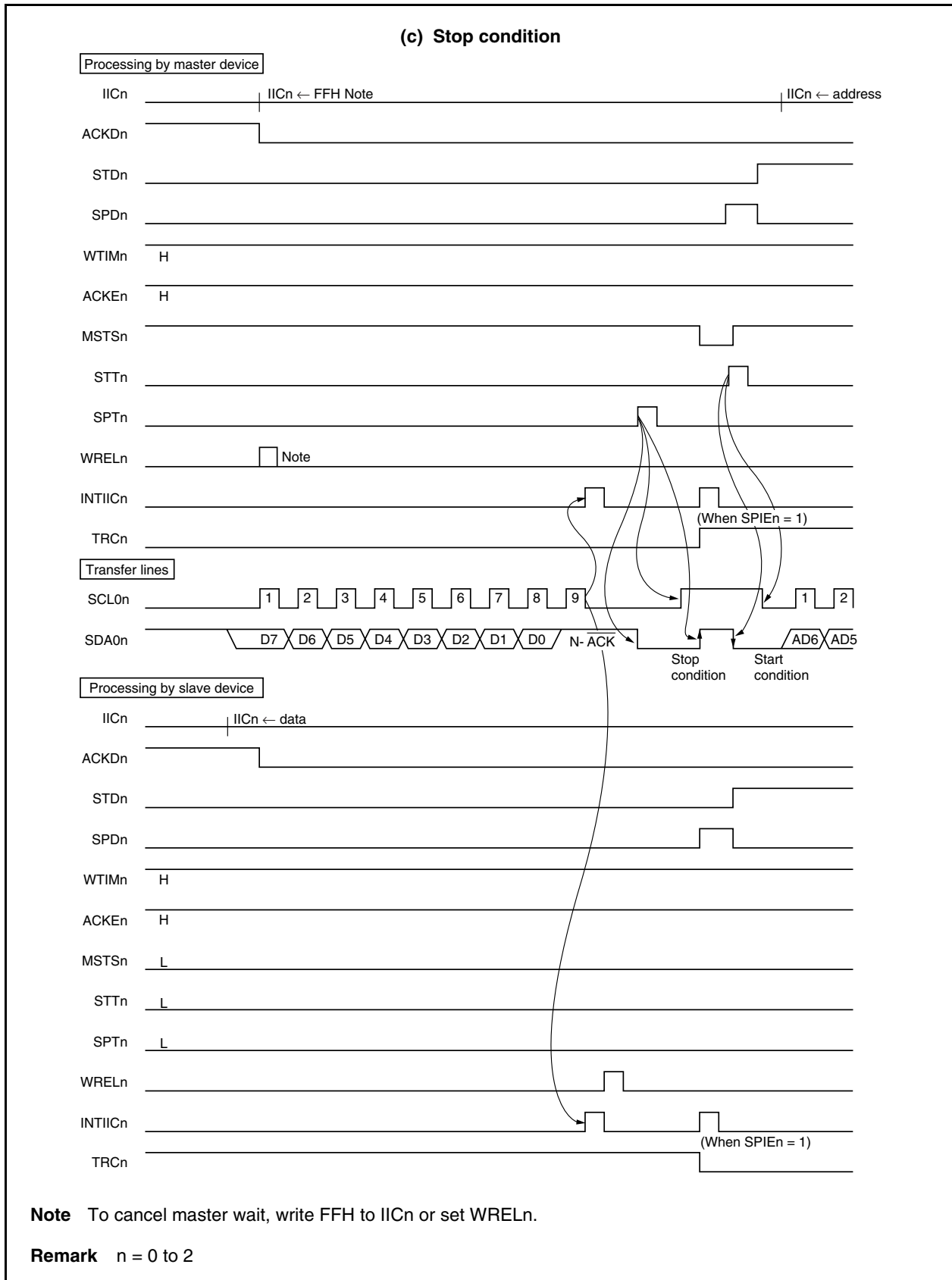
Figure 17-22. Example of Slave to Master Communication (When 9-Clock Wait Is Selected for Both Master and Slave) (3/3)
