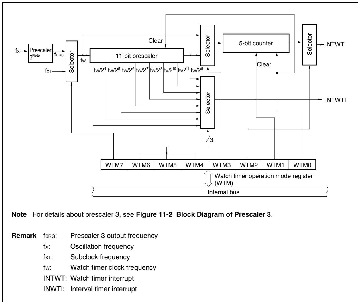
Figure 11-1. Block Diagram of Watch Timer
