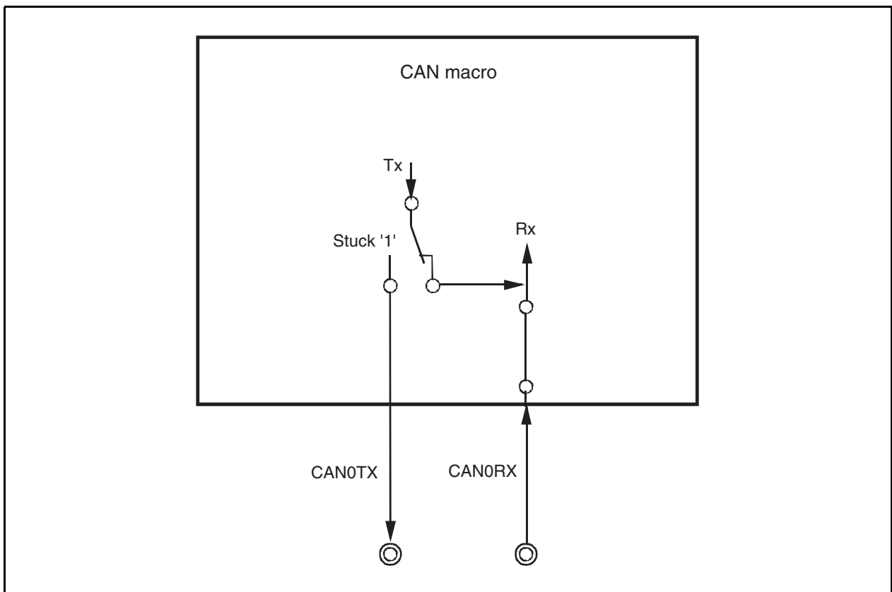
Figure 19-40. CAN Module Terminal Connection in Receive-Only Mode
