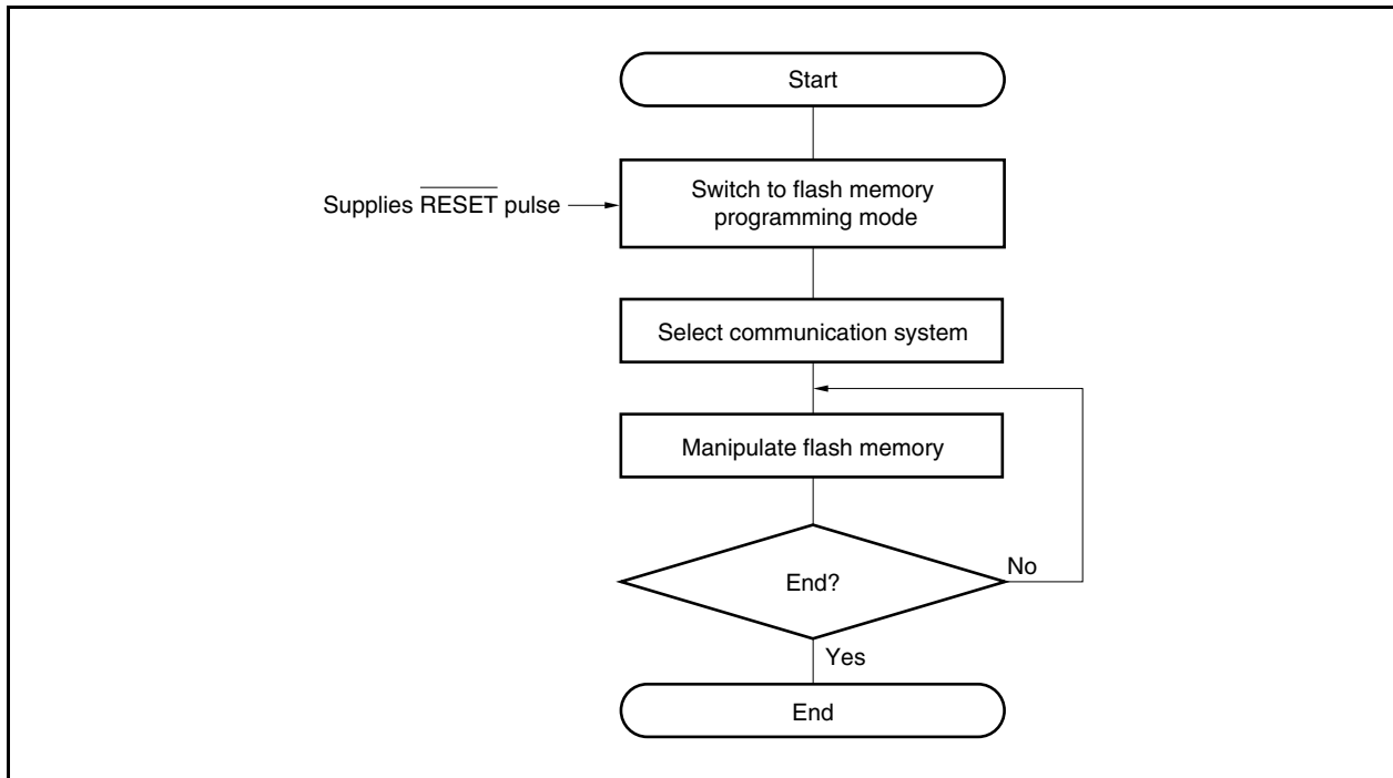
Figure 28-10. Procedure for Manipulating Flash Memory
