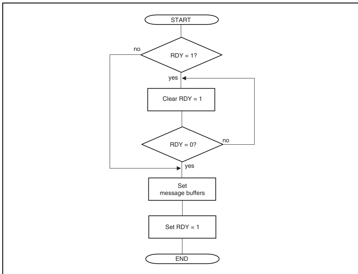
Figure 19-47. Message Buffer Redefinition
