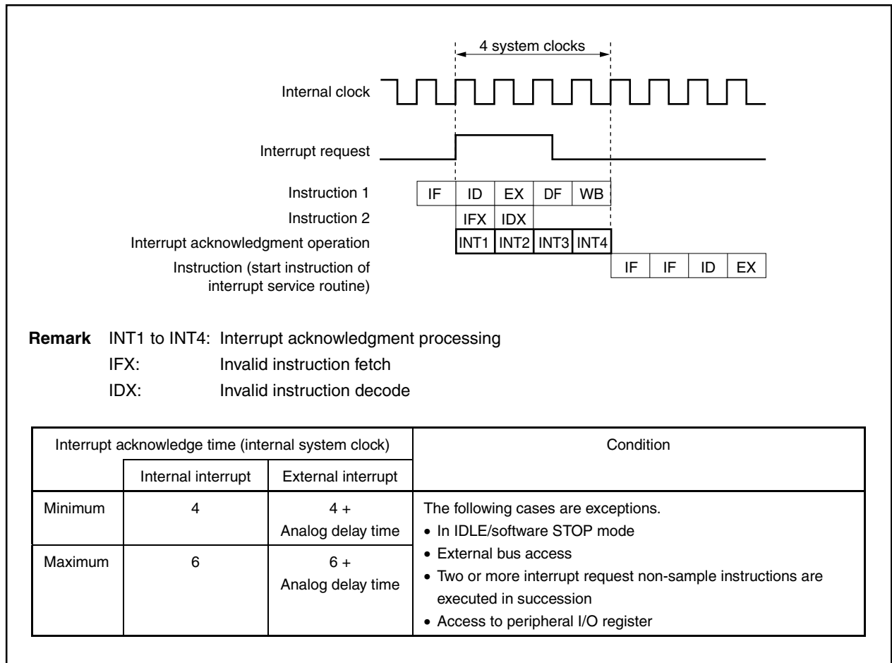
Figure 22-14. Pipeline Operation at Interrupt Request Signal Acknowledgment (Outline)
