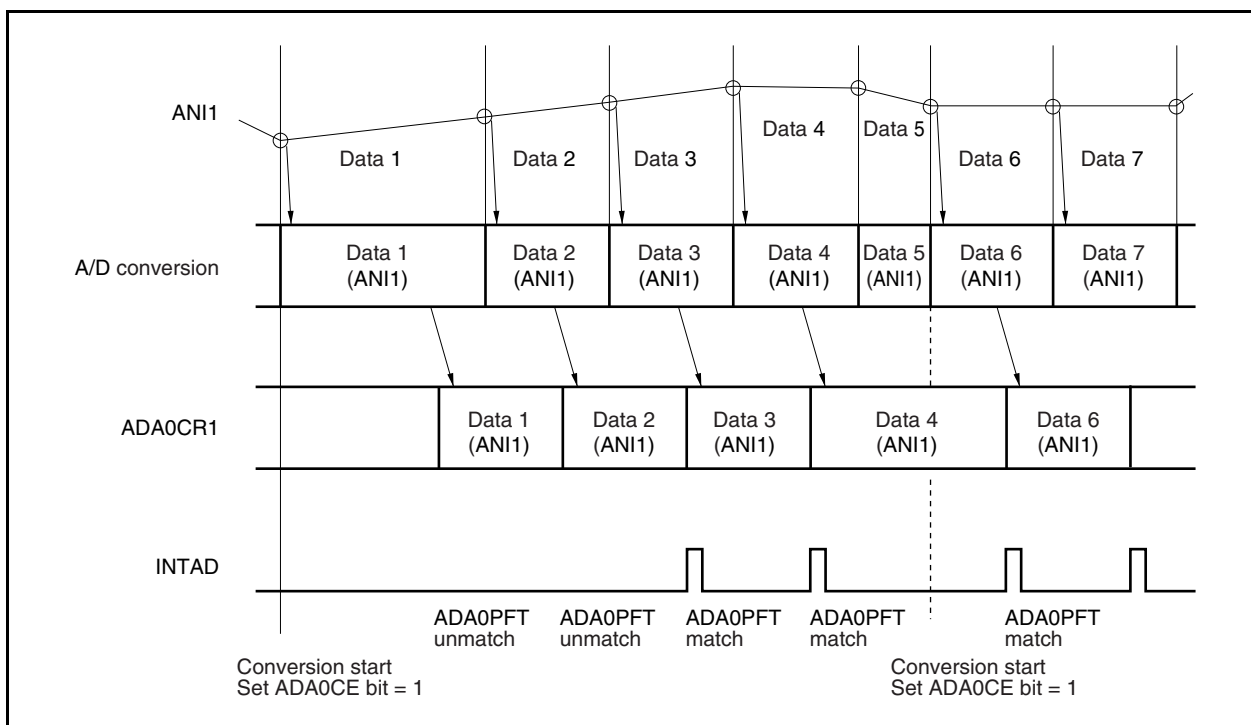
Figure 13-8. Timing Example of Continuous Select Mode Operation (When Power-Fail Compare Is Made: ADA0S Register = 01H)
