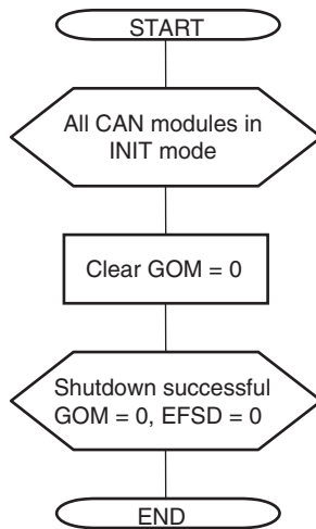
Figure 19-61. Shutdown Process (Normal Shutdown)
