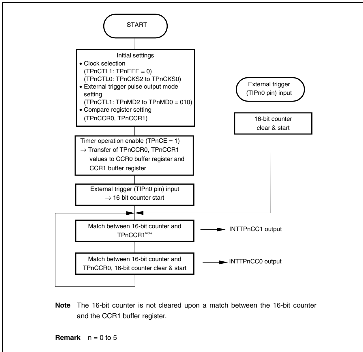
Figure 7-10. Flowchart of Basic Operation in External Trigger Pulse Output Mode
