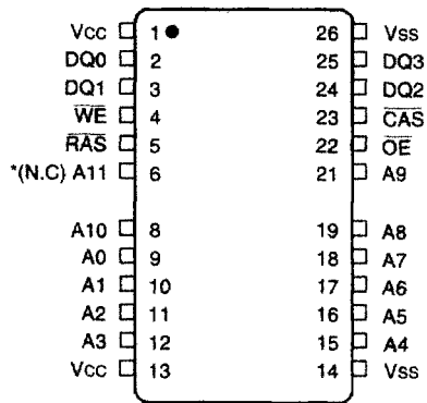
24/26Pin Plastic SOJ (300mil)
