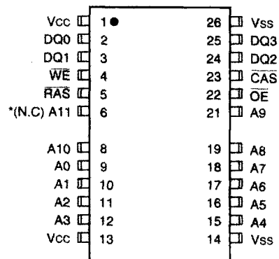
24/26Pin Plastic TSOP-II (300mil)
