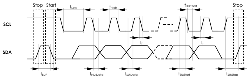
Figure 17 - 2-wire data transfer chronograms
