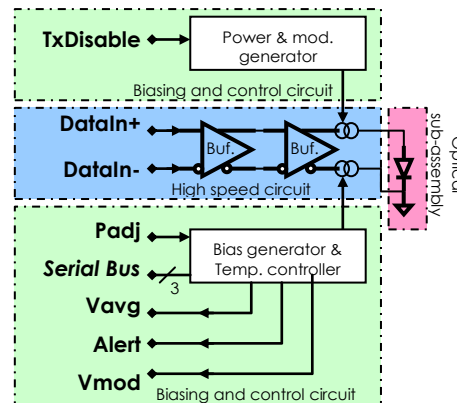
Figure 3 - Transmitter block diagram
