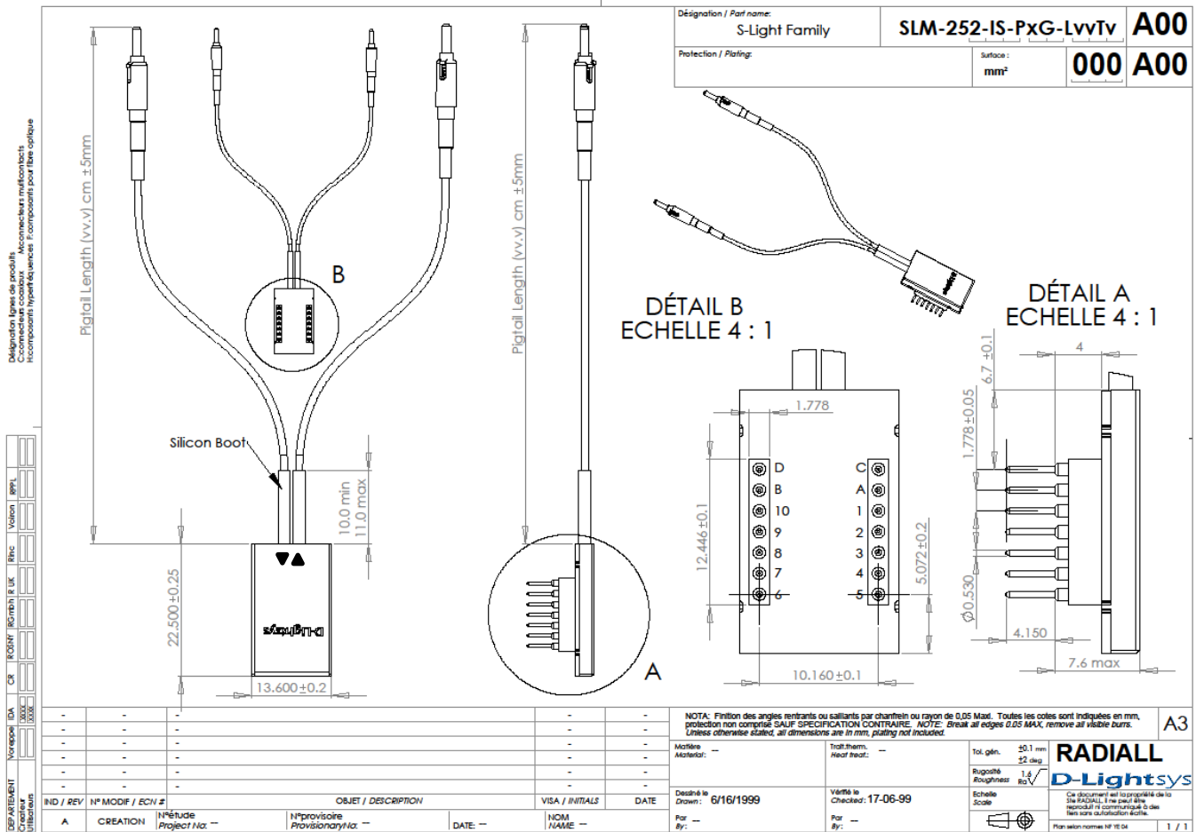
Note that the silicon boot is a flexible strength release boot Figure 21 - 2x7 SFF MSA compatible mechanical drawing.
