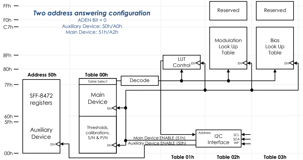
Figure 14 - Memory organization for ADEN bit set to 0 (SFF-8742)
