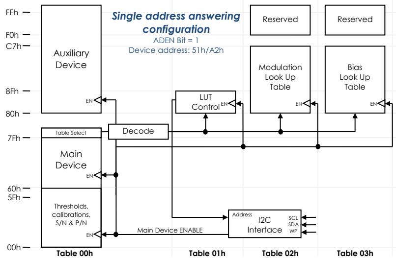
Figure 15 - Memory organization for ADEN bit set to 1
