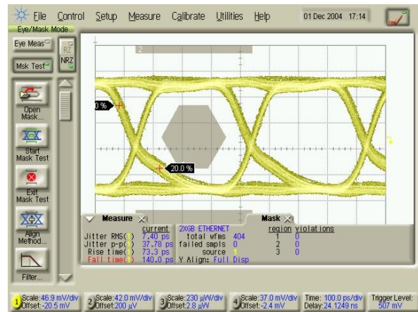
Figure 20 - 2.5Gbps Rx electrical eye diagram. 90°C external temperature.
