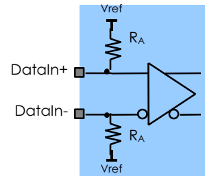
Figure 4 - Input stage
