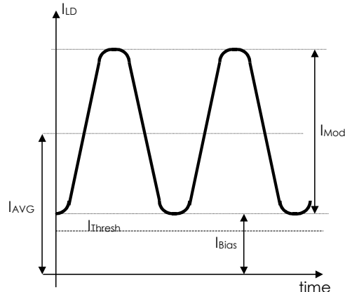
Figure 6 - Laser diode current
