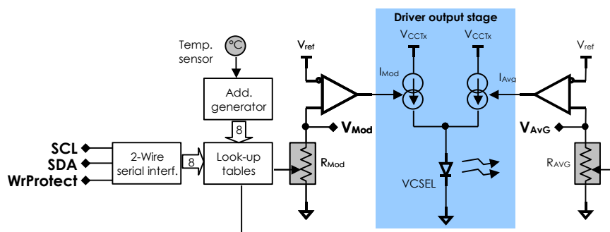
Figure 7 - Average and modulation current control circuit
