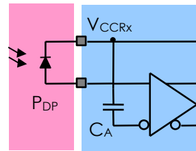
Figure 10 - Photodiode input stage
