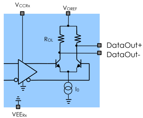
Figure 11 - Data output stage
