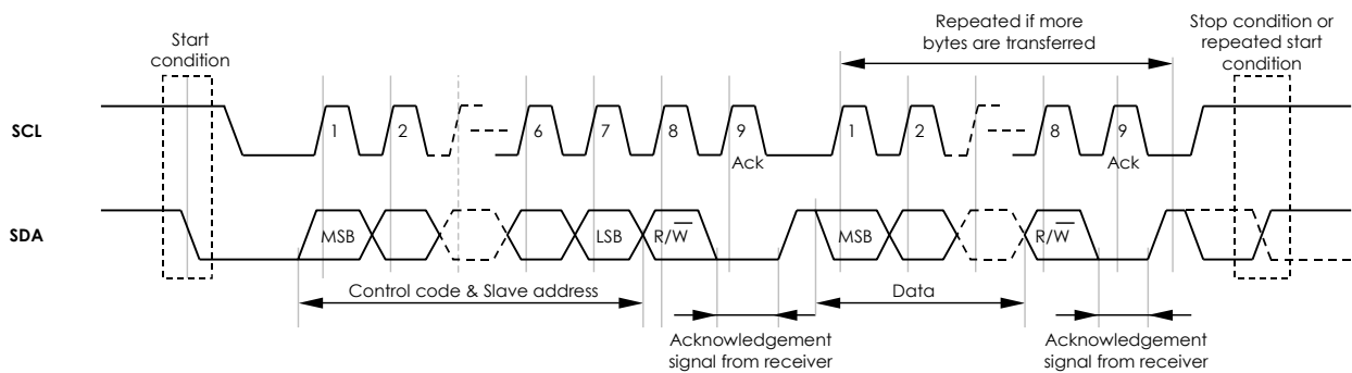
Figure 16 - 2-wire data transfer chronograms
