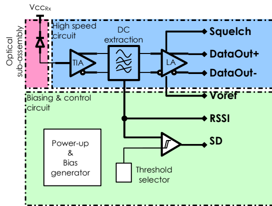
Figure 9 - Receiver bloc diagram
