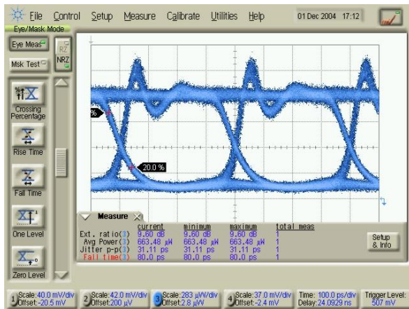
Figure 19 - 2.5Gbps Tx optical eye diagram. 90°C external temperature.
