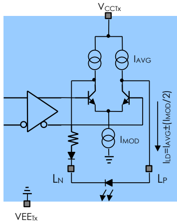
Figure 5 - Output stage
