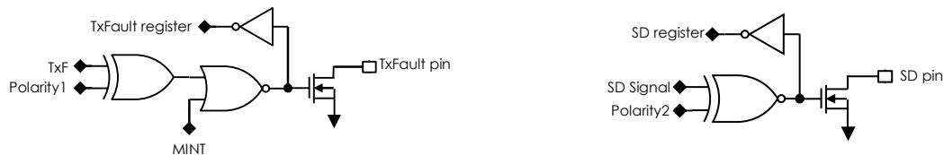
(a) TxFault Pin logic circuit
