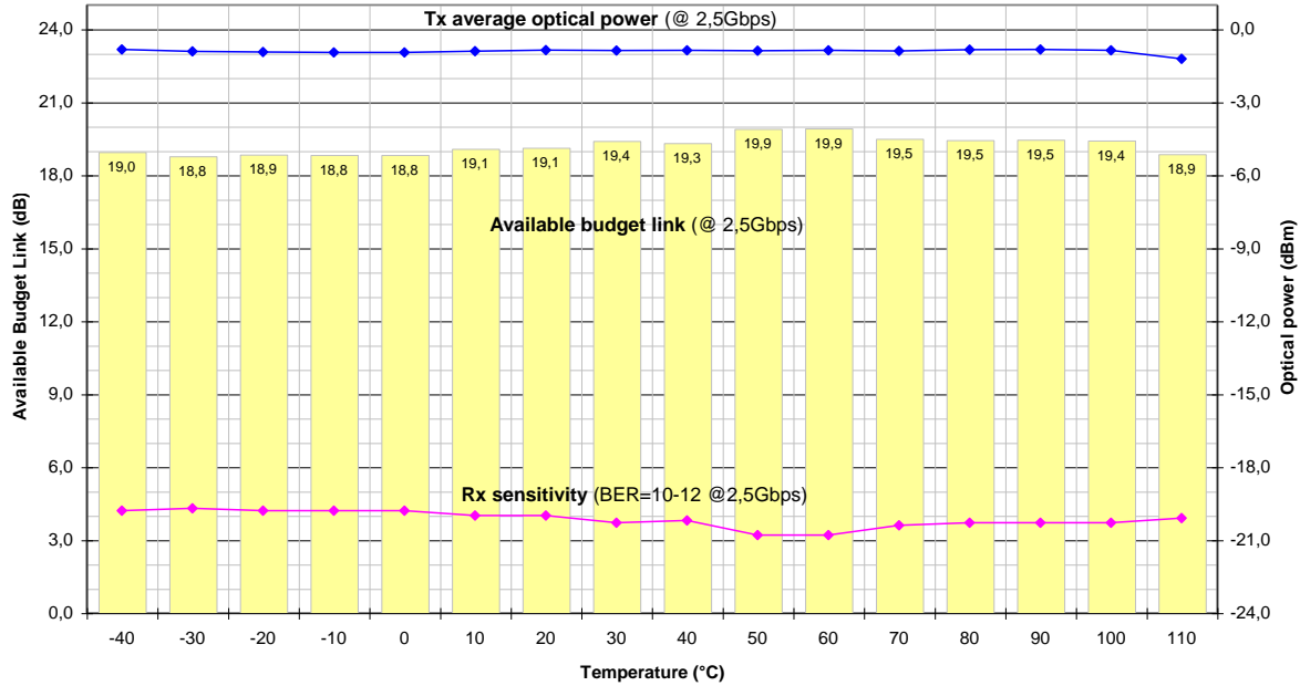
Figure 18 - Typical Tx optical power, Rx optical sensitivity and corresponding available budget link as a function of temperature at 2.5 Gbps.
