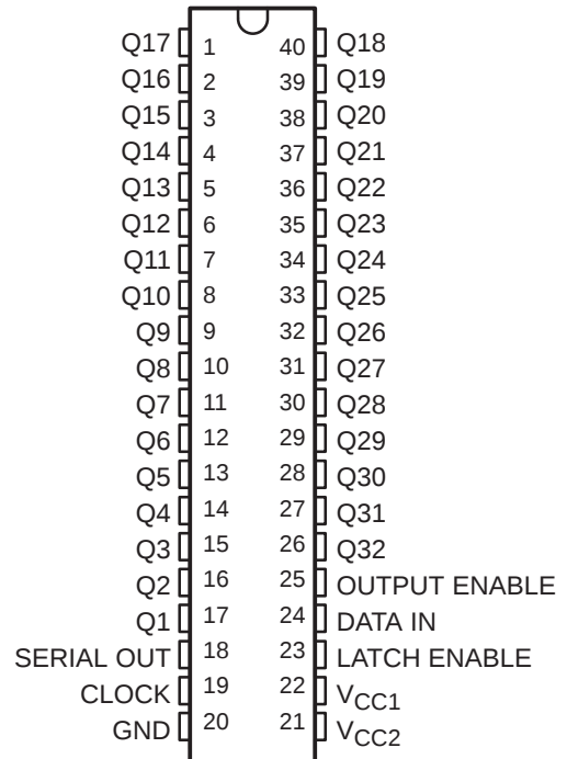
SN75555 . . . N PACKAGE (TOP VIEW)
