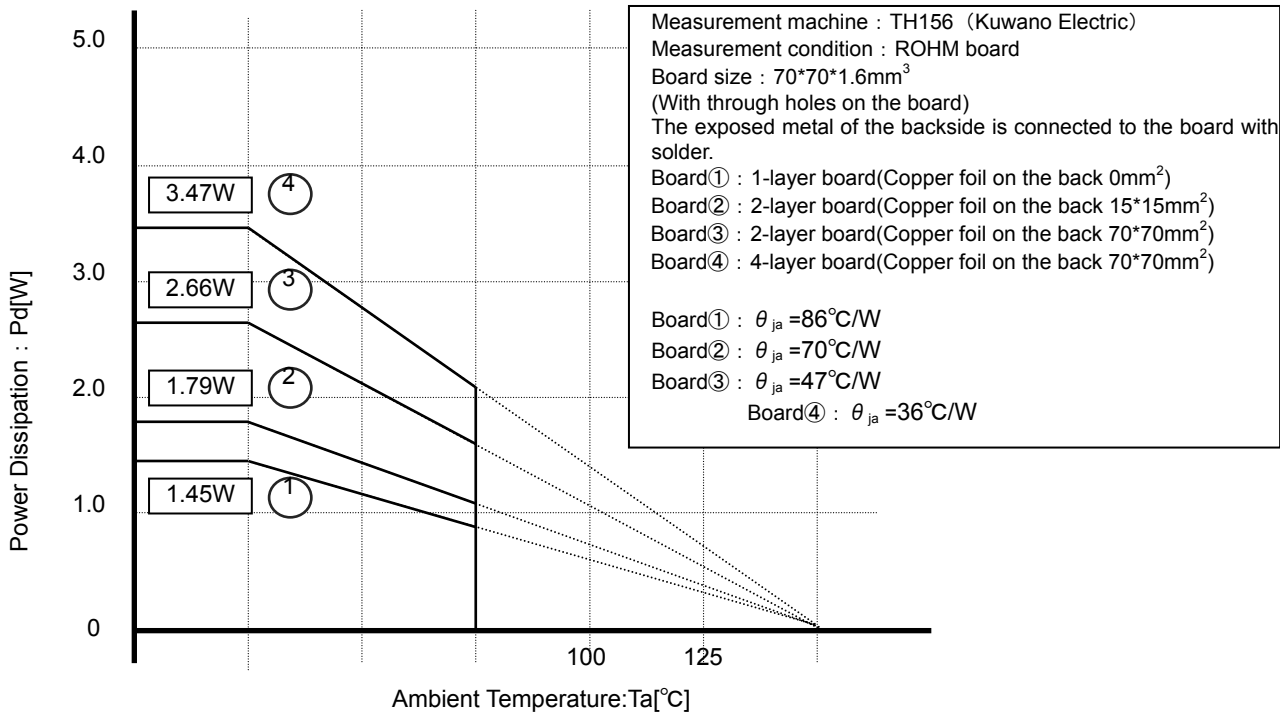
Fig. 2 HSOP25 Derating curve
