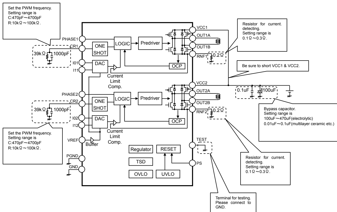
Fig.1 Block diagram &amp; Application circuit diagram
