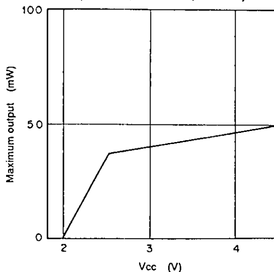
Maximum output vs. Vcc characteristics (8 \Omega load) ( f_o=1\text{kHz} , THD=10%, R_L=8\ \Omega )
