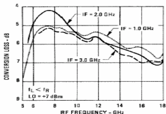
Conversion Loss
